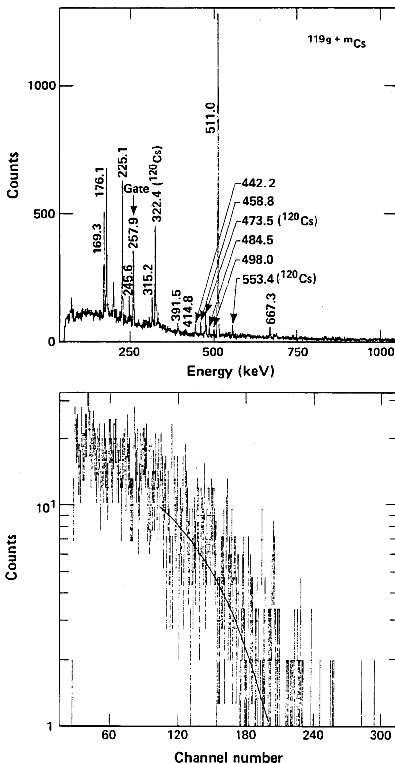
Figure 29. Beta-coincident gamma ray and beta decay spectra of ^{119\text{m}+g}\text{Cs} .
