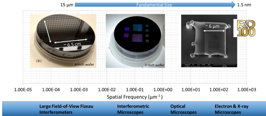
Figure 3. Several BPR test samples designed, fabricated, and tested for a variety of metrology tools, including Fizeau interferometers, interferometric microscopes, and scanning probe and atomic force microscopes. The fundamental sizes of the arrays range from 1.5 nm to 15 \mu\text{m} .
