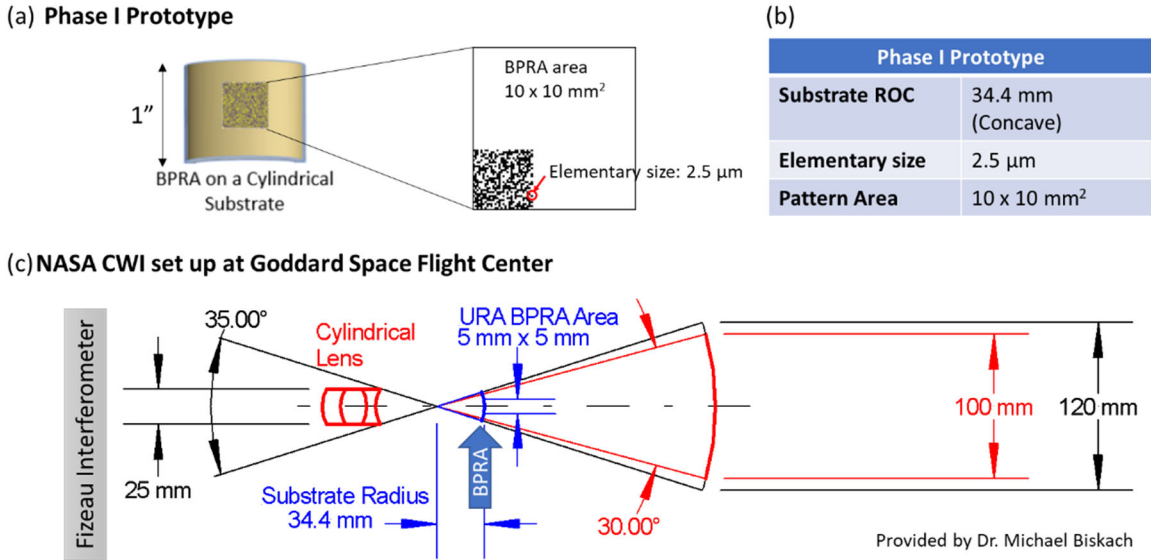
Figure 5. (a) Illustration of the prototype BPRA test artifact on a cylindrical substrate. (b) a table of design parameters optimized to characterize the CWI setup at NASA Goddard Space Flight Center, (c) A scheme of the CWI setup at NASA. The blue arrow marked with “BPRA” indicates the placement of the fabricated BPRA test artifact.
