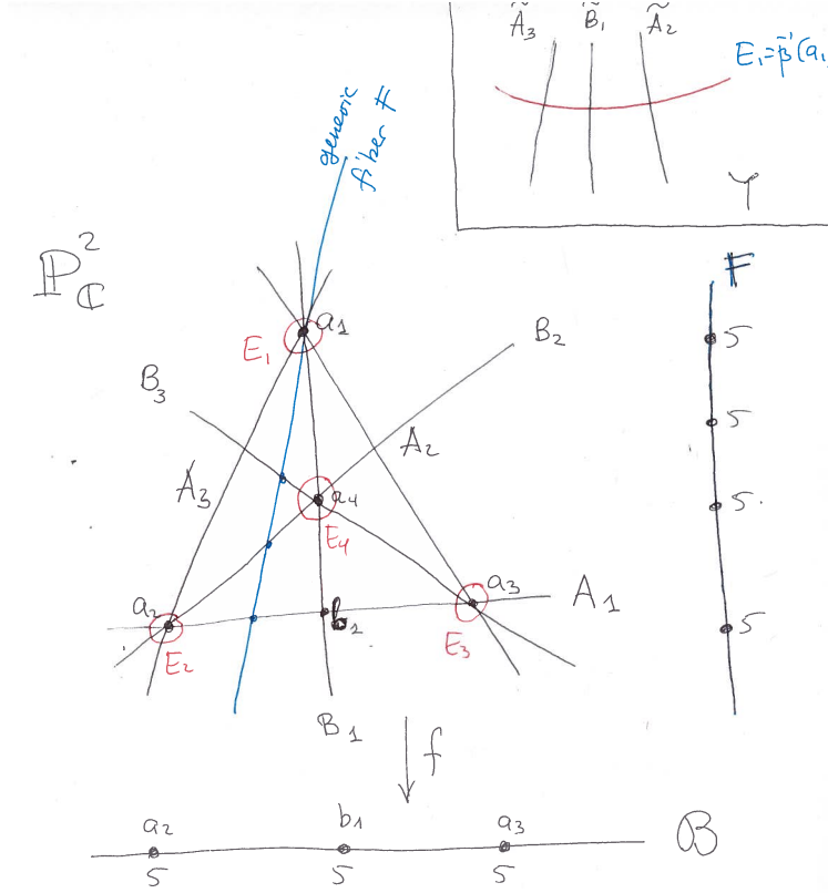
FIGURE 2. Singular Kodaira orbi-fibration
