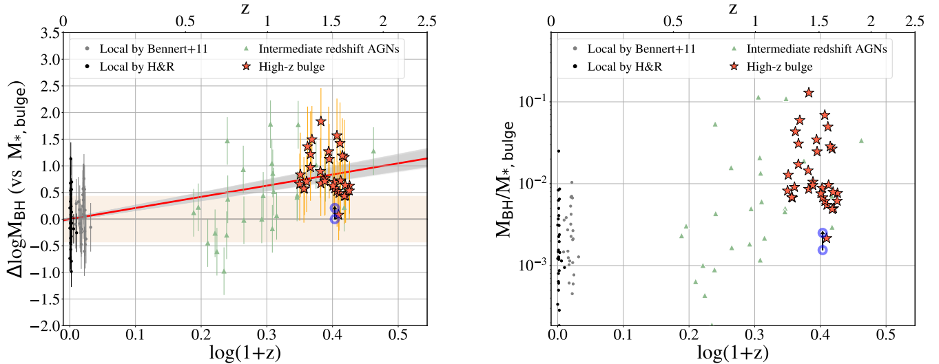
FIG. 13.— Same as Figure 8, but for M_{\text{BH}}-M_{*, \text{bulge}} relations. The intermediate sample consists of 27 objects from Bennert et al. (2011b) and Schramm & Silverman (2013) , listed in Table 7. Cisternas et al. (2011) do not provide information to infer their bulge mass.
