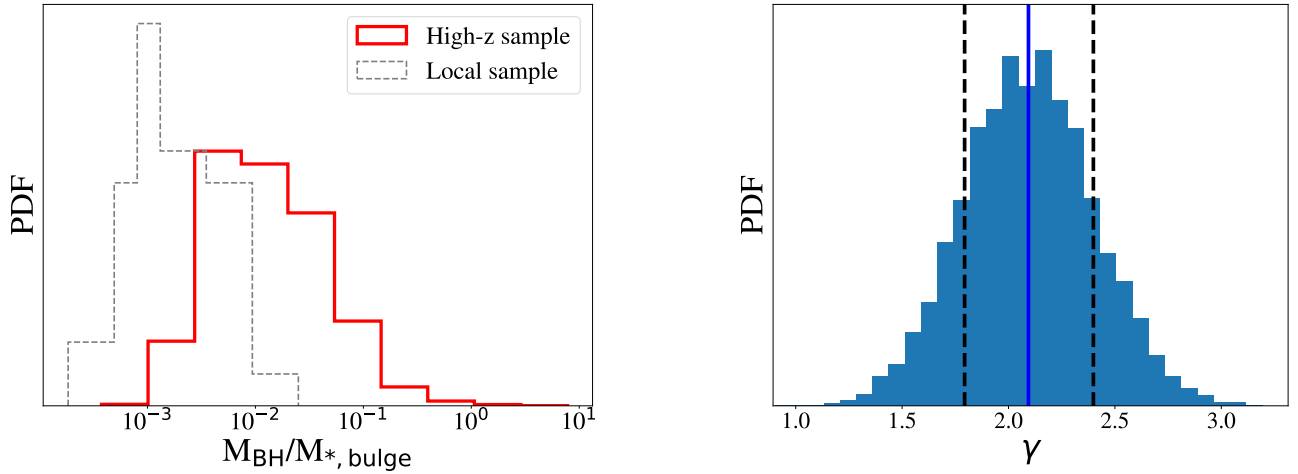
FIG. 12.— Illustration of the distribution from the 10,000 time realizations. Left: M_{\text{BH}}/M_{*} distribution for 32 high- z sample, compared to the local one. Right: \gamma distribution, with median value (blue line) and 1\sigma region (dashed line).
