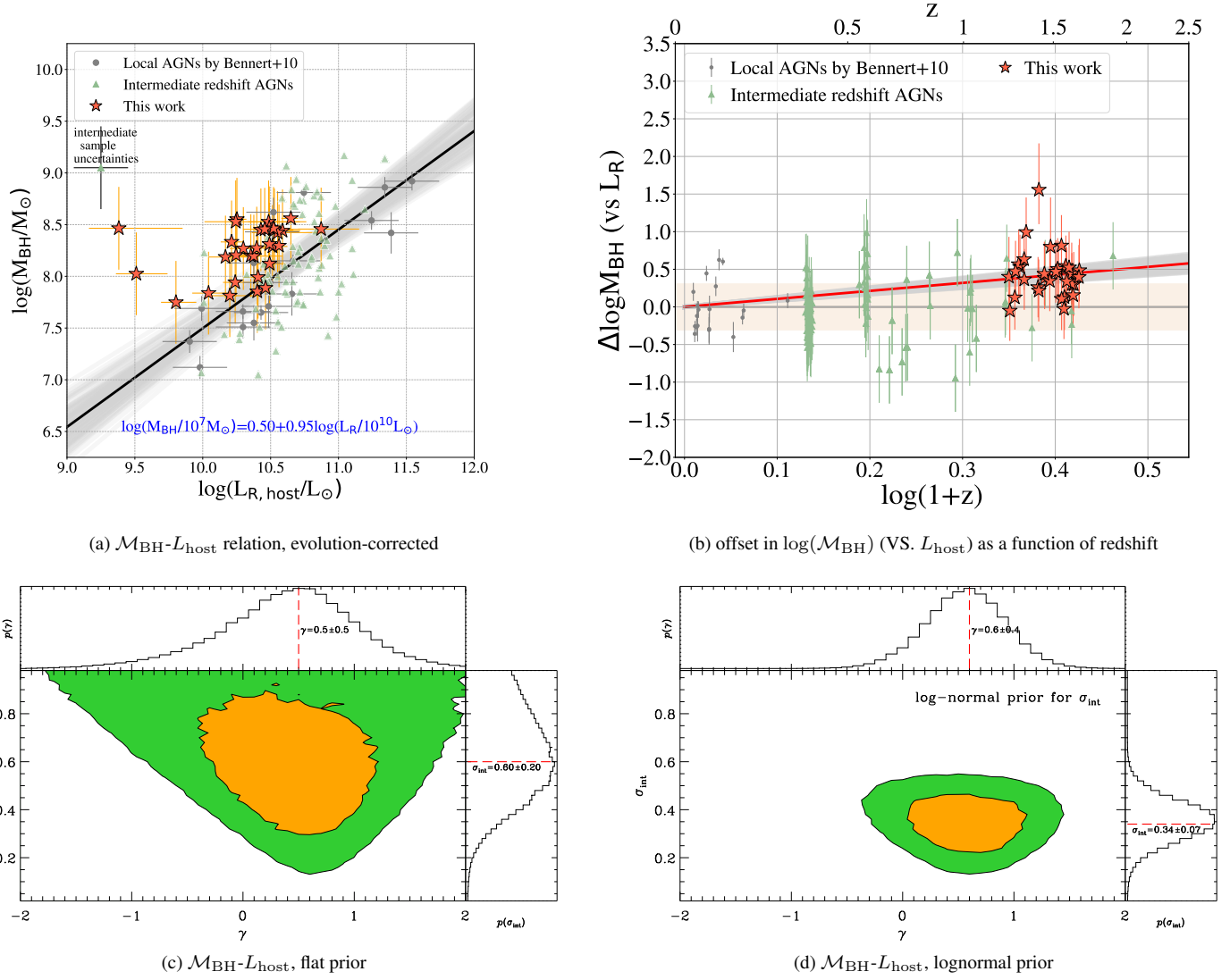
FIG. 14.— Same as previous figures but for \mathcal{M}_{\text{BH}}-L_{\text{host}} relation, considering the passive evolution correction for host galaxy luminosity.
