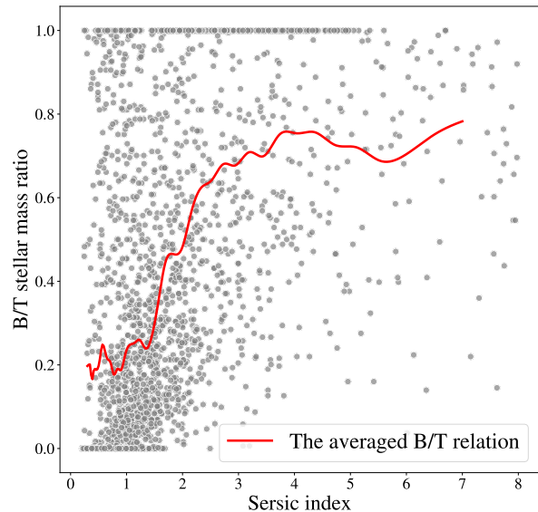
FIG. 11.— Relation between bulge-to-total stellar mass ratio and single-Sérsic index using CANDELS inactive galaxies with \log(M_*/M_\odot) \in [9.0, 11.5] . The red curve is the averaged B/T ratio at different Sérsic index. Note that this curve is only for demonstrating the expected B/T value at different Sérsic index. In this work we adopt the Monte Carlo approach to randomly sample the B/T to account for the scatter.
