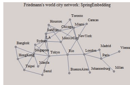
Figure 1. Spring embedding of Friedmann city graph.
