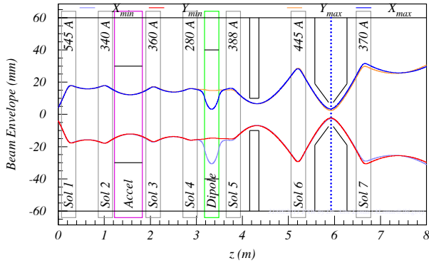
FIG. 5: {}^4\text{He}^+ 50 keV, 50 mA (2.5 kW, neutralization 90 %, no post-acceleration) beam envelopes through the gas-jet target station beam line. The dotted blue vertical line represents the gas-jet target location.
