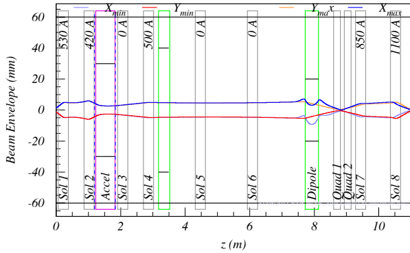
FIG. 16: {}^4\text{He}^+ 400 keV 625 \mu\text{A} (350 kV post-acceleration, 250 W, neutralization 90 %) beam envelopes through the solid-target station beam line. The two high-energy quadrupoles are shown but not used in the present calculation.
