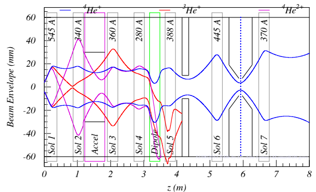
FIG. 11: Horizontal beam envelopes for a {}^4\text{He}^+ 50 keV 50 mA, with 1 mA of {}^3\text{He}^+ and 1 mA {}^4\text{He}^{2+} contaminations (neutralization 90 %). While the {}^4\text{He}^{2+} is eliminated in the analyzing magnet chamber, the {}^3\text{He}^+ is stopped by the pumping stage aperture. A similar study have been performed for a \text{H}^+ 50 keV 100 mA beam with 10 mA of \text{H}_2^+ and 1 mA of \text{H}_3^+ . In this case both parasitic beams are eliminated at the column entrance, by the analyzing magnet chamber and by the pumping stage aperture.
