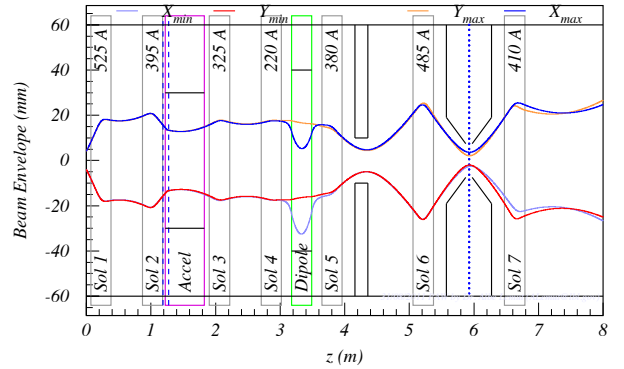
FIG. 9: {}^4\text{He}^+ 60 keV, 50 mA (10 kV post acceleration, 3 kW, gap-width 2.6 mm, screening voltage -3 kV, neutralization 90 %) beam envelopes through the gas-jet target station beam line. Between the two dashed blue vertical lines the beam is treated at full space charge (length 86.4 mm).
