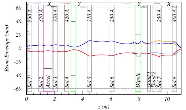
FIG. 15: {}^4\text{He}^+ 50 keV 5 mA (no post-acceleration, 250 W, neutralization 90 %) beam envelopes through the solid-target station beam line. The two high-energy quadrupoles are shown but not used in the present calculation.
