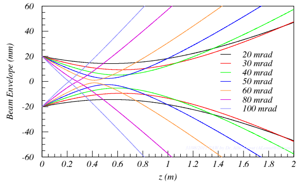
FIG. 4: {}^4\text{He}^+ 50 keV, 50 mA initially uniform (initial emittance \epsilon_{4RMS} = 4 \pi mm mrad), 2 cm radius, free drifting beams (neutralization 90 %) for several initial converging angles. The longest drifting distance for the beam to reach the same initial radius is 1.3 m for the 30 mrad convergent beam.
