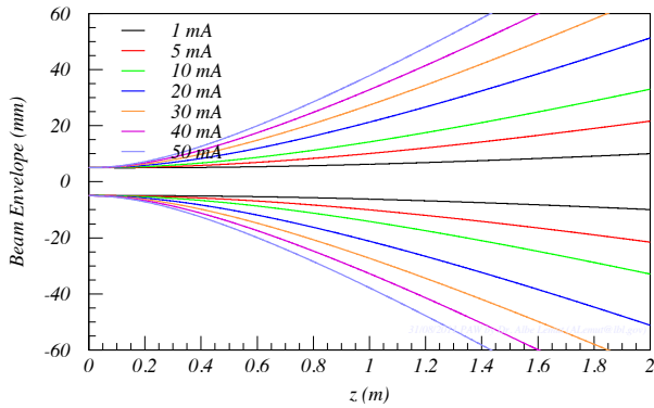
FIG. 3: Beam envelope growth for {}^4\text{He}^+ 50 keV initially quasi-parallel ( \epsilon_{4RMS} = 4 \pi mm mrad, beam envelope divergence 0.7 mrad), 0.5 cm radius, uniform, free drifting beams (neutralization 90 %) at selected currents. The 50 mA beam reaches a 2 cm radius after 0.6 m.
