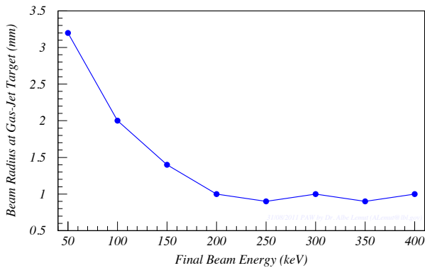
FIG. 13: {}^4\text{He}^+ beam radius at gas-jet target location for selected final beam energies. The beam current have been scaled down not to exceed 5 kW of beam power (neutralization 90 %).
