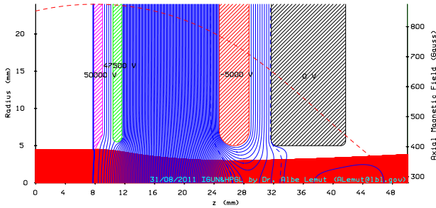
FIG. 2: Calculation of the extraction of {}^4\text{He}^+ 50 mA by means of the IGUN program [16]. The extraction electrode (shaded magenta area, inner radius 4.5 mm), the puller electrode (shaded green area), screening electrode (shaded red area), ground electrode (shaded black area), particle trajectories (red), and equipotential lines (blue) for a 50 kV extraction voltage are shown. The final ( z = 50 mm) beam emittance \epsilon_{4RMS} is 4\pi mm mrad, the radius 3.9 mm, and the divergence 55.1 mrad. The axial magnetic field (dashed red line), and the -200 V equipotential (dashed blue lines) are also plotted (see text in Sec III B).
