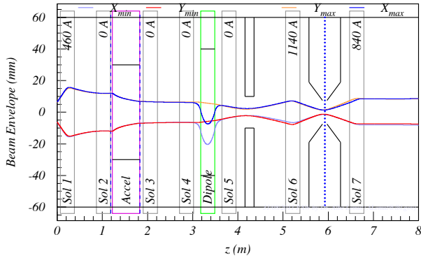
FIG. 12: {}^4\text{He}^+ 400 keV 12.5 mA (350 kV post acceleration, 5 kW, gap-width 550 mm, screening voltage -5 kV, neutralization 90 %) beam envelopes through the gas-jet target station beam line. Between the two dashed blue vertical lines (overlapped on the focal elements symbols) the beam is treated at full space charge (length 647.7 mm).
