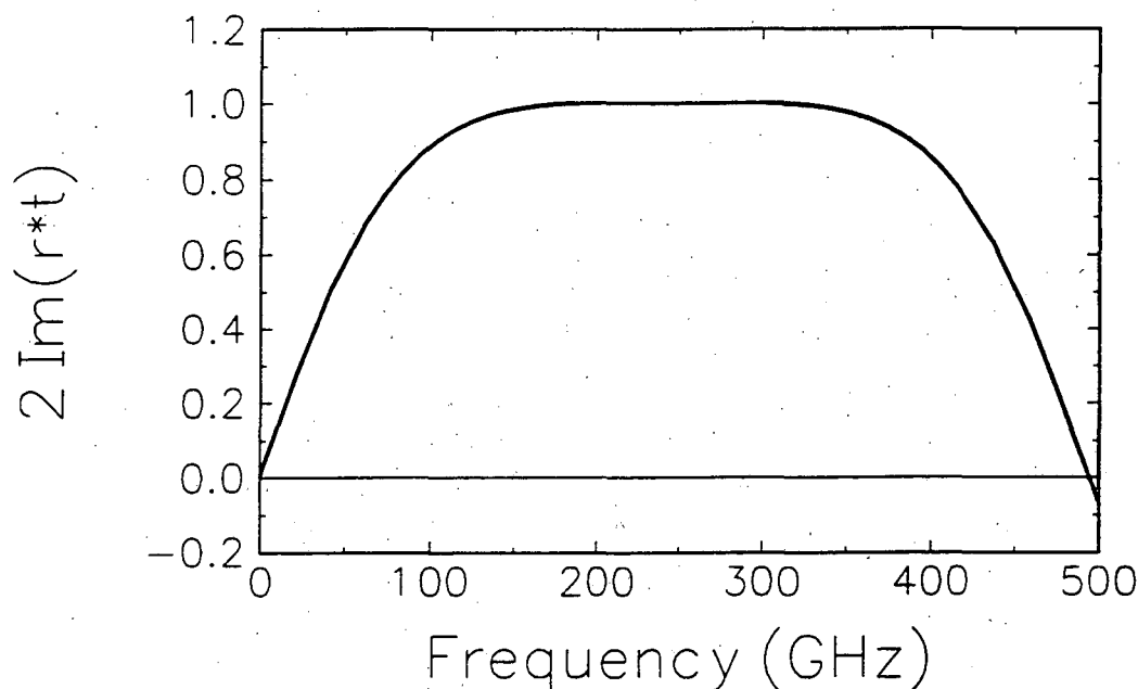
Figure 6.3: Beam splitter efficiency 2\text{Im}[r_{\perp}t_{\perp}^*] plotted as a function of frequency for a Mylar beamsplitter with thickness 175\text{ }\mu\text{m} and \theta_1 = \pi/4 . This beamsplitter has useful efficiency from 50 – 450 GHz.
