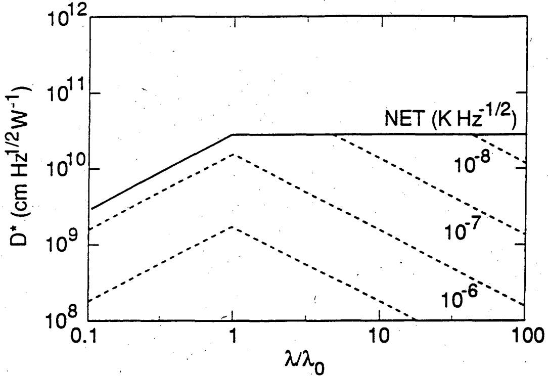
Figure 3.4: Specific detectivity D^* as a function of reduced wavelength \lambda/\lambda_0 where \lambda_0 depends on the minimum achievable values of the heat capacity per unit area C_A and thermal conductance G_{\min} as well as the response time \tau , the number N of electromagnetic modes which couple, and the solid angle \Omega of the pixel's field of view. The solid line shows the predicted phonon noise limit for a bolometer on a thin membrane. The dashed lines show upper limits on D^* for thermometers with various values of NET.
