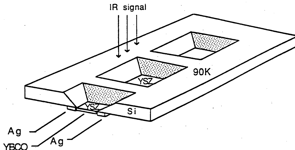
Figure 4.1: Diagram of three membrane bolometers. Each bolometer consists of a YBCO film which functions as the radiation absorber and as the thermometer. The YSZ membrane is in contact with the heat sink along its perimeter. Radiation is incident on the bolometer from the top side and is partially collected by the 54^\circ facets in the silicon which are produced by the anisotropic Si etch.
