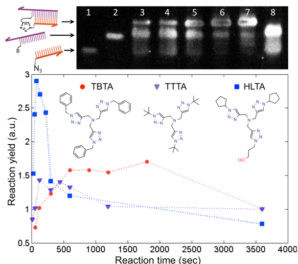
Fig. 2 Use of denaturing polyacrylamide gel electrophoresis to quantify the DNA-templated crosslinking reaction yield in solution. (Top) Sample gel image. Lanes 1 and 2 are the target and anchor strands, respectively. Lanes 3-7 are a series of time points from a mixture of both strands after hybridization and reaction with the Cu(I) catalyst under one set of conditions tested. Lane 8 is a control where the Cu(I) catalyst was omitted. (Bottom) Reaction yield with three copper chelating ligands as a function of time. The decrease in yield at longer times can be attributed to oxidative degradation of the DNA. We found that degradation could be significantly reduced by minimizing the amount of oxygen present and by using an excess of the ligand.
