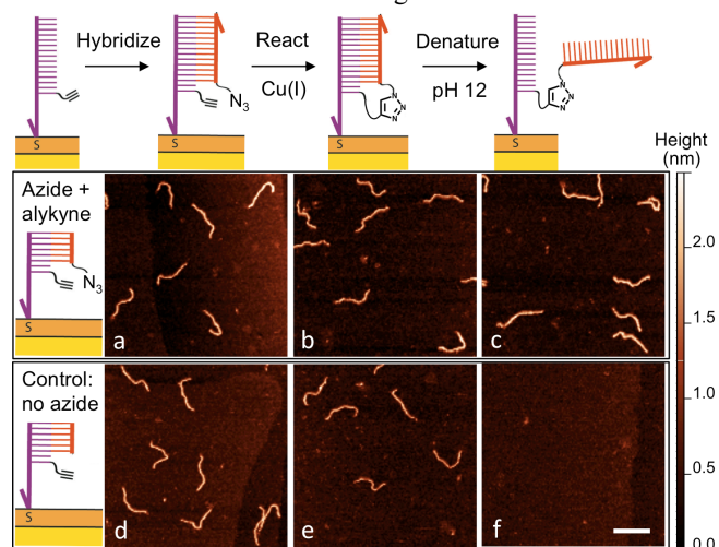
Fig. 3 AFM images taken after each step of attaching 396 bp DNA to the surface. (a) First the azide-labeled DNA targets are hybridized with surface anchor strands containing an alkyne group. (b) Next the surface is exposed to Cu(I), catalyzing the formation of the triazole product. (c) To verify that the DNA is covalently crosslinked, the surface is exposed to alkaline conditions so that any unreacted DNA is denatured and rinsed away. (d), (e) and (f) show the same hybridization, reaction, and denaturation steps, respectively, but with the azide group omitted. In this case, >99% of the DNA was removed after denaturing. Scale bar is 100 nm.
