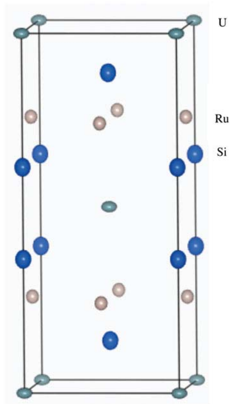
Figure 1. (colour online) Crystal structure of \text{URu}_2\text{Si}_2 determined by the single-crystal X-ray diffraction. The ellipsoids at the atomic sites are drawn using the anisotropic atomic displacement parameters.
