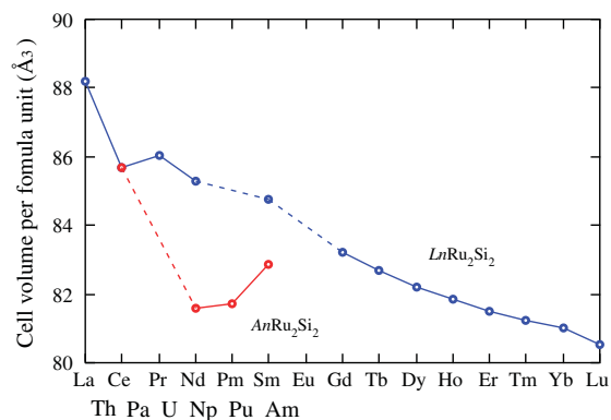
Figure 2. (colour online) Unit cell volume of AnRu_2Si_2 ( An : actinide) and LnRu_2Si_2 ( Ln : lanthanide).
