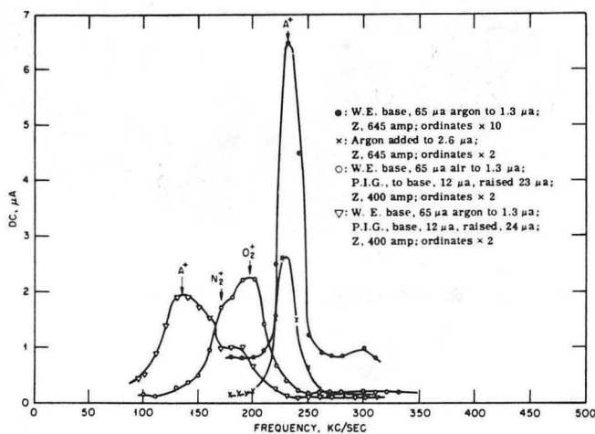
Fig. 3. Resonance curve data from model for uranium separation cyclotron. 12
