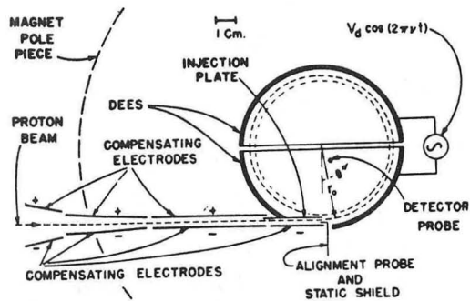
Fig. 10. Decelerating cyclotron designed by Jeffries at Stanford. 18 Outer orbit diameter is 7.6 cm.
