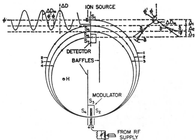
Fig. 7. Brookhaven mass synchronizer decelerating cyclotron. 16 Diameter of first orbit is 28 cm.
