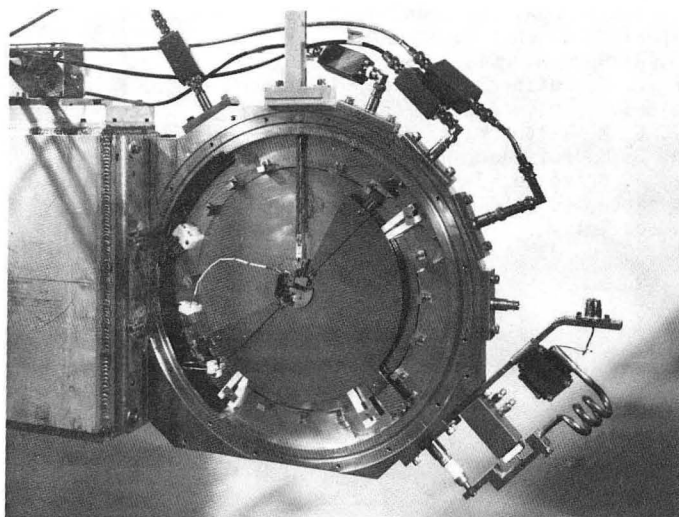
Fig. 11. LBL mass spectrometer cyclotron being developed by Muller and Welch. 19 Orbit diameter is 20 cm.
