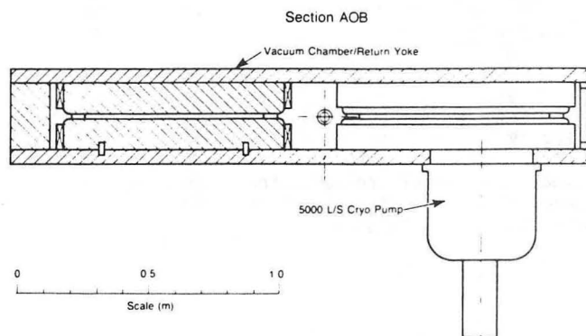
Fig. 12. Proposed mass spectrometer cyclotron of Jongen, Louvain-la-Neuve. 20 Outer orbit diameter is 160 cm.
