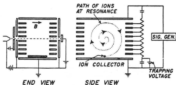
Fig. 4. Omegatron mass spectrometer developed at the National Bureau of Standards. 13 Orbit diameter is 2 cm.
