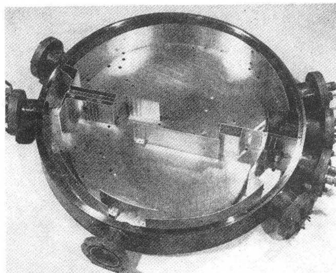
Fig. 8. Brookhaven mass synchronizer. 16
