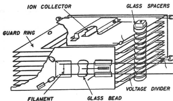
Fig. 5. Cutaway view of omegatron. 13
