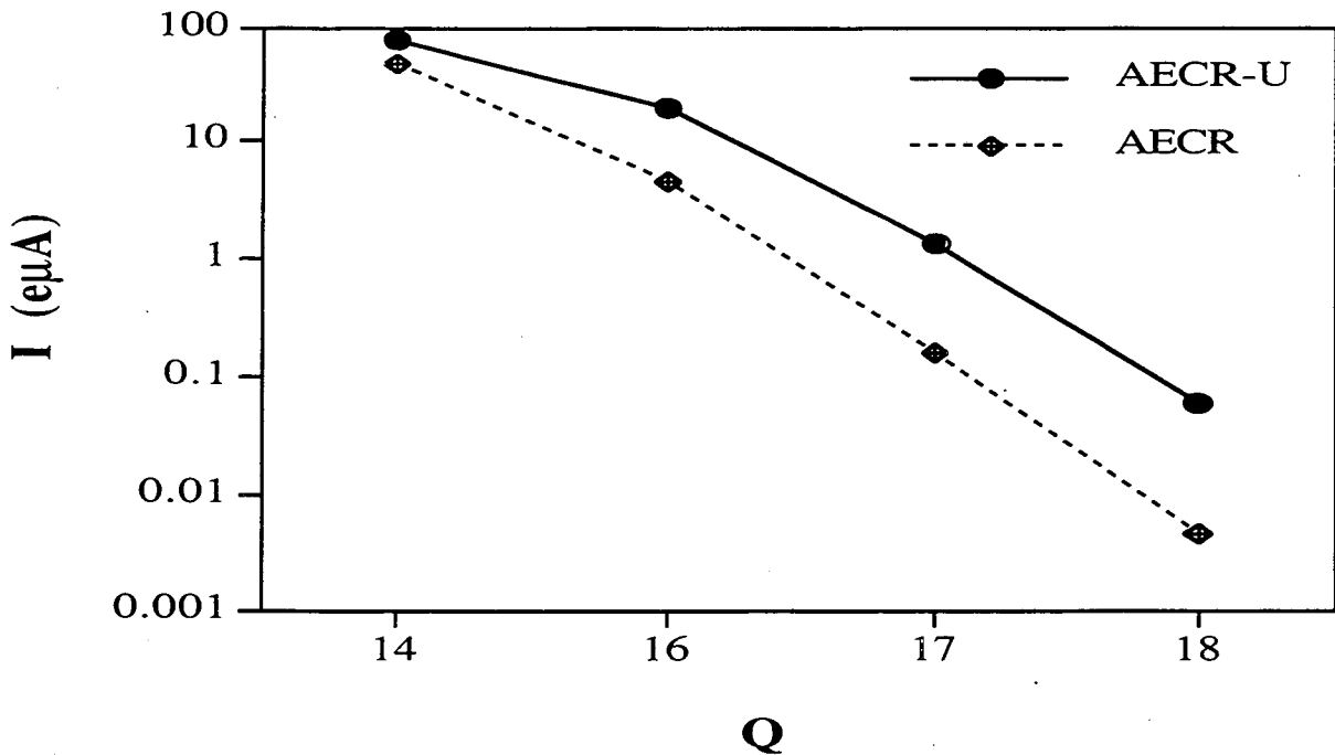
Fig. 4. A comparison of the best high charge state argon ion beams before (indicated by AE-CR) and after the AE-CR source upgrade (AE-CR-U). The 60 e nA of Ar 18+ from the AE-CR-U represents more than an order of magnitude enhancement on the fully stripped argon ions.
