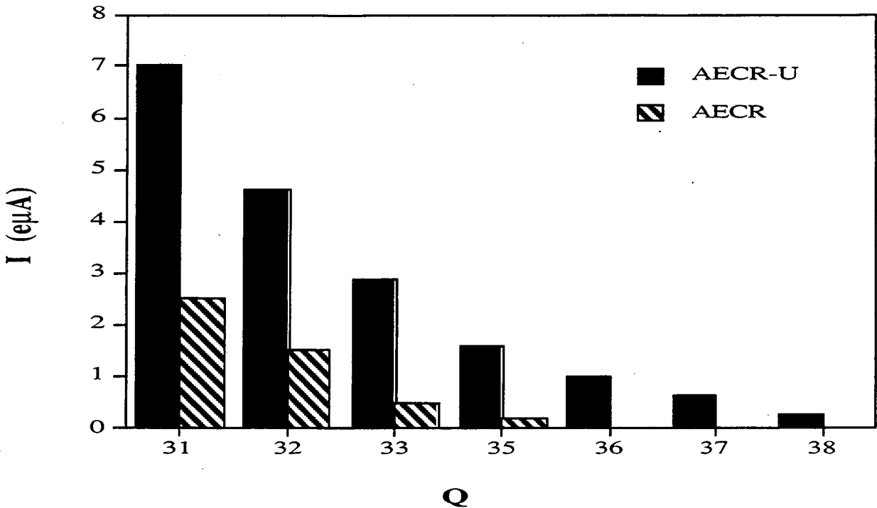
Fig. 3. A comparison of the best high charge state xenon-136 ion beams before (indicated by AE-CR) and after the AE-CR source upgrade (AE-CR-U). Beside a factor of 3 to 5 improvement on xenon charge state 31+ to 35+, at 1 eμA level, the charge state was shifted 4 charge state higher from 32+ to 36+.
