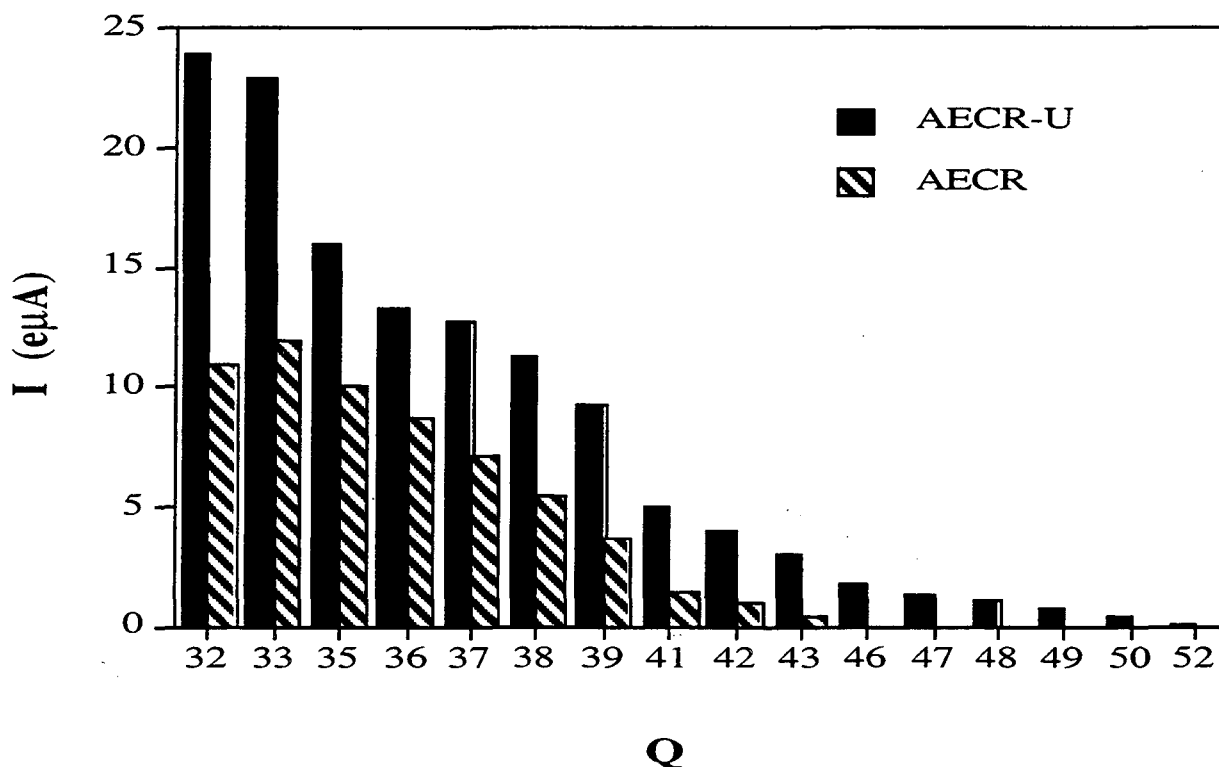
Fig. 2. A comparison of the best high charge state uranium-238 ion beams before (indicated by AECR) and after the AECR source upgrade (AECR-U). Beside enhancement on the lower charge states, at 1 \mu\text{A} level, the charge state was shifted 6 charge states higher from 42+ to 48+.
