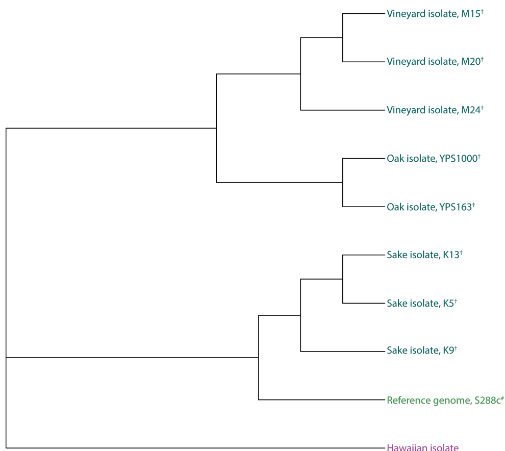
Figure 4.8. Neighbor-joining tree of Hawaiian, laboratory, and wild S. cerevisiae strains. Constructed from polymorphic sites at five unlinked loci. Isolates in dark green text and denoted with † were constructed with Genbank sequences from Fay & Benavides [165]. Isolates in light green text and denoted with # were constructed from the S288c reference Saccharomyces cerevisiae genome assembly (April 2011 release) [167,168]. Isolates in pink text are from this study.
