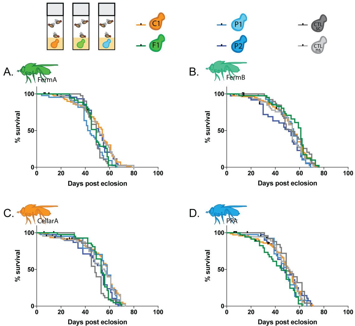
Figure 2.6. Fly-associated yeasts have no differing effects on Drosophila longevity.
