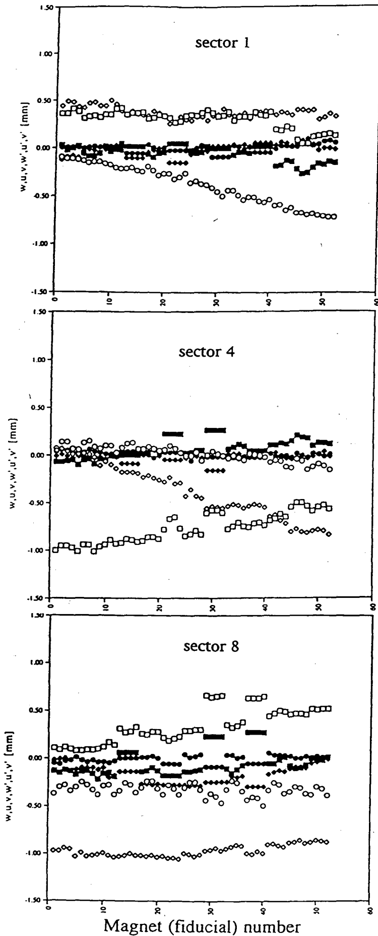
Figure 9 Deviations of Storage Ring magnets in the local magnets coordinate system before and after alignment in 1995 in sectors 1,4,8.
