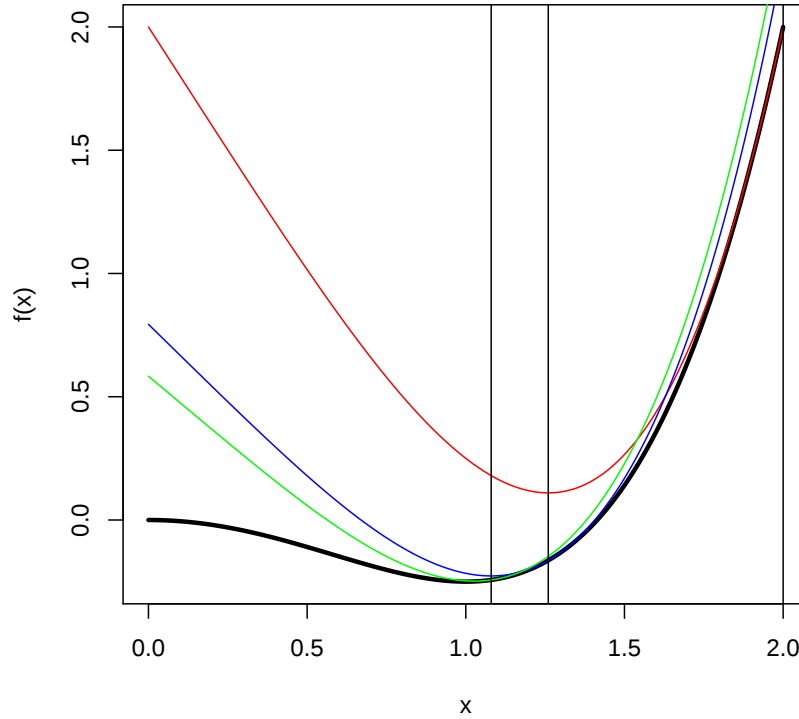
FIGURE 1. Majorization Example
