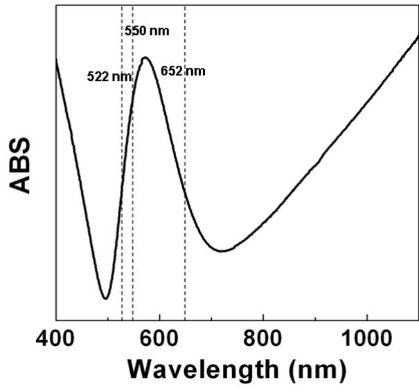
Figure 4-9. UV-Vis spectrum of the gold island film sputtered on a glass slide.
