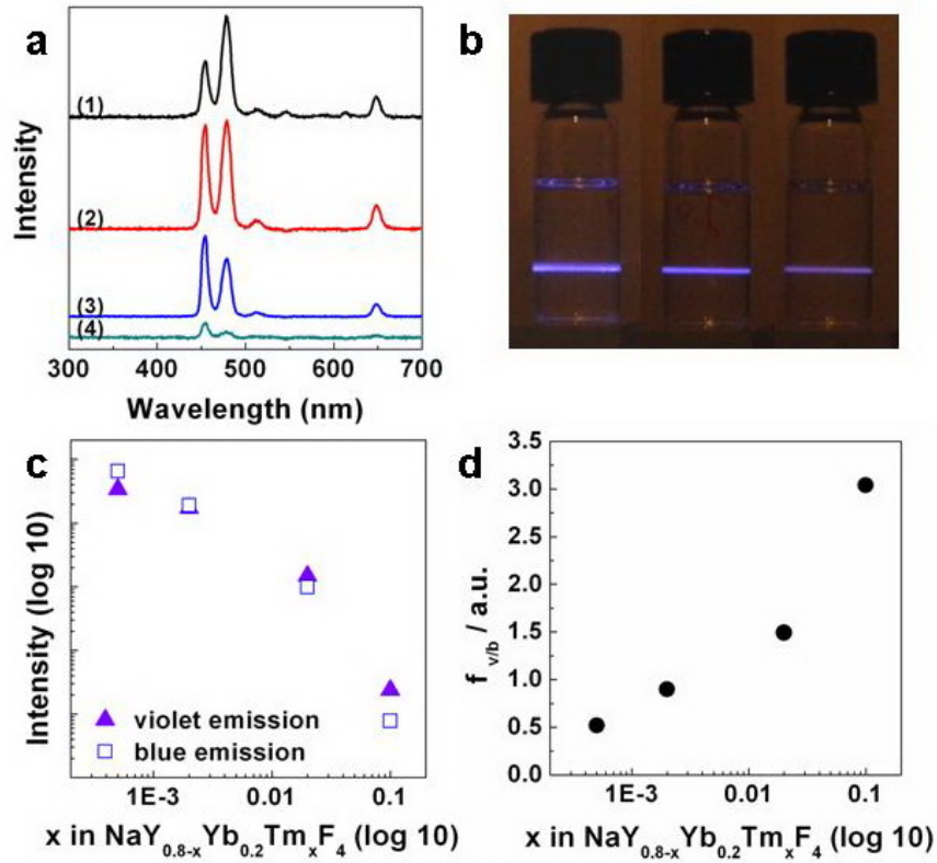
Figure 2-4 (a) Upconversion emission spectra of NaY 0.8-x Yb 0.2 Tm x F 4 NCs with different Tm 3+ concentrations, x = 0.0005, 0.002, 0.02, 0.1, for (1), (2), (3), (4) respectively. (b) Digital camera pictures of NaY 0.78 Yb 0.2 Tm 0.02 F 4 , NaY 0.798 Yb 0.2 Tm 0.002 F 4 and NaY 0.7995 Yb 0.2 Tm 0.0005 F 4 samples under 980 nm excitation. (c) Upconversion emission intensity (normalized by Tm 3+ ion concentration) versus doping concentration of Tm 3+ in NaY 0.8-x Yb 0.2 Tm x F 4 NCs. (d) Diagram of violet to blue emission (f v/b ) ratio versus Tm 3+ doping concentration in NaY 0.8-x Yb 0.2 Tm x F 4 NCs.
