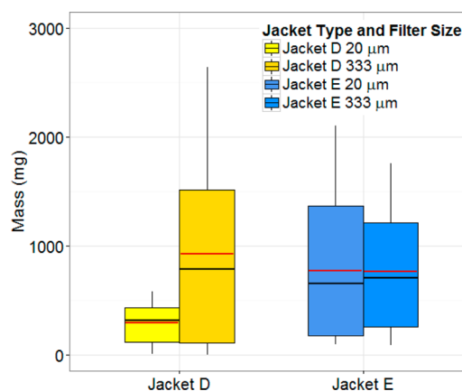
Figure 4. Distribution of fiber mass recovered for jacket D versus jacket E on the 20 and 333 \mu\text{m} mesh filters ( n = 14 each box), across all treatments including aged or new and front- or top-load washing modes. Red lines indicate means, black lines medians, and black dots outliers (beyond 1.5 times the interquartile range).
