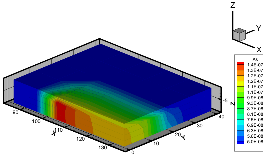
Fig. 4.82. Close-up view of spatial distribution of total aqueous As concentration after 100 years of CO 2 intrusion in the 3D model with CO 2 leakage rate of 7.5 \times 10^{-5} kg/s.
