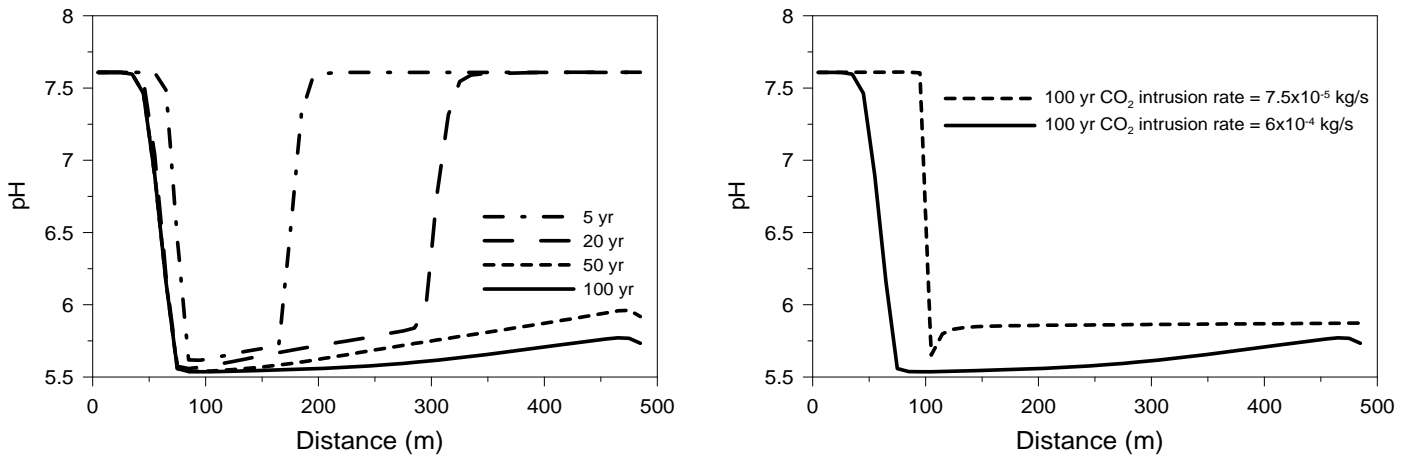
Fig. 4.54. pH evolution at different times (left) along the x-axis at y = 0 m for CO 2 intrusion rate of 6x10 -4 kg/s, and sensitivity of pH to CO 2 intrusion rate.
