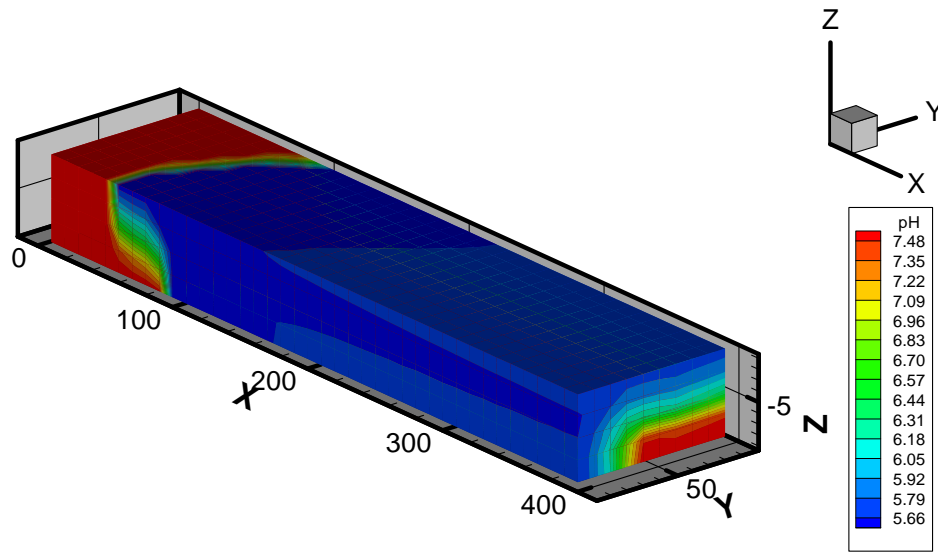
Fig. 4.106. Spatial distribution of pH after 100 years of CO 2 intrusion in 3D model with CO 2 leakage rate of 6 \times 10^{-4} kg/s.
