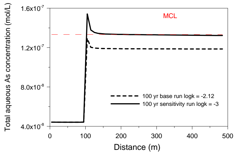
Fig. 4.26. Computed As concentration after 100 years of CO 2 intrusion in a sensitivity run (logK = -3) and base model (logK = -2.12)
