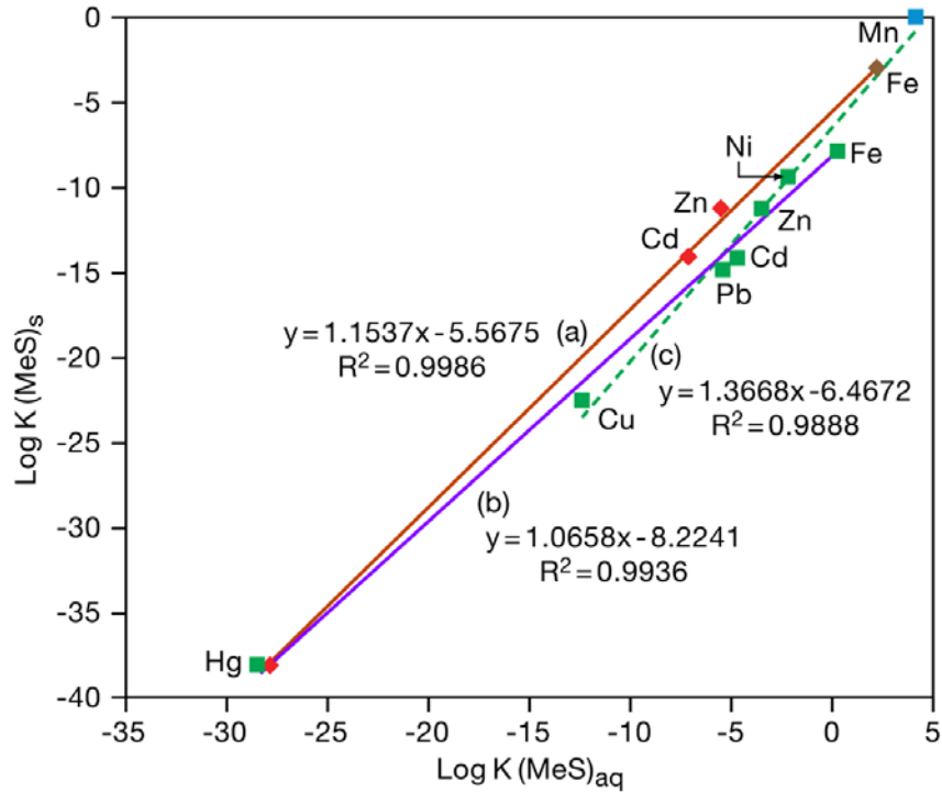
Fig. D1. Correlation between the solubility product of a sulfide mineral, and the apparent dissociation constant of the corresponding neutral species in solution at 25°C.
