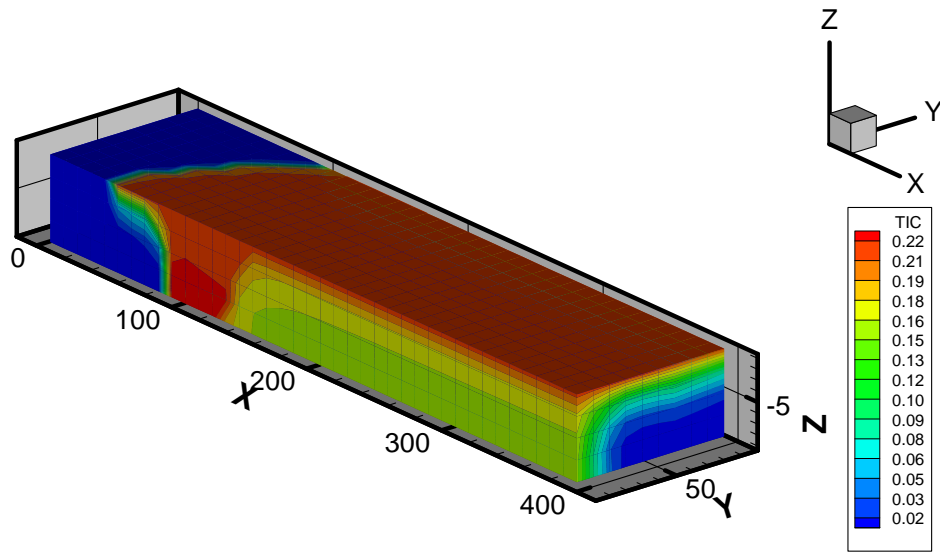
Fig. 4.104. Spatial distribution of TIC after 100 years of CO 2 intrusion in 3D model with CO 2 leakage rate of 6 \times 10^{-4} kg/s.
