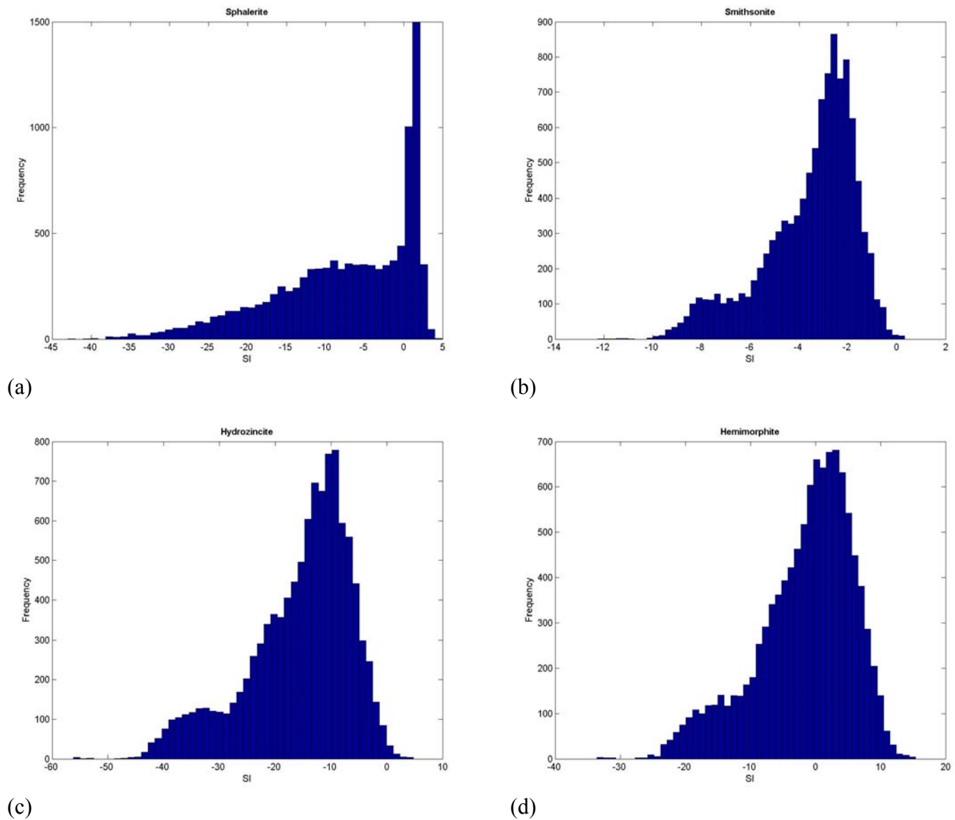
Fig. 3.33. Frequency Distribution of the Saturation Indices of (a) Sphalerite, (b) Smithsonite, (c) Hydrozincite and (d) Hemimorphite. The Saturation Indices are calculated, using a selected set of groundwaters from the NWIS, and assuming Eh to be defined by Fe(III)/Fe(II) in solution.
