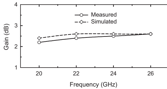
Figure 2.8: Measured and simulated gain vs. frequency for the 60° angled-dipole antenna.
