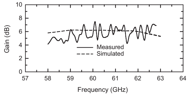
Figure 2.19: Measured and simulated gain of the 60 GHz 45° angled-dipole antenna.
