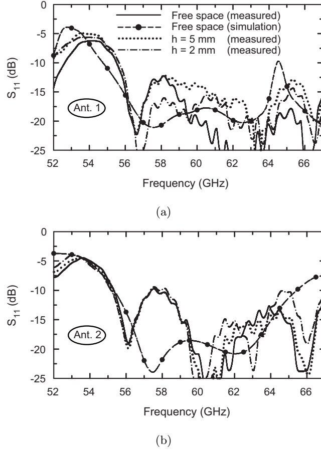
Figure 4.20: Measured S_{11} of : (a) Ant. 1 , (b) Ant. 2. Simulations shown for free space case only for Ant.1 and Ant. 2.
