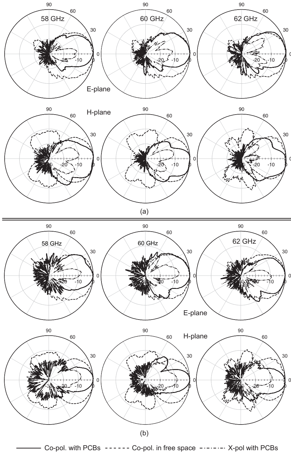
Figure 4.17: Measured radiation patterns of the 60 GHz Yagi-Uda antenna with two PCBs on top and bottom of the antenna: (a) without metal shield, (b) with box shielding.
