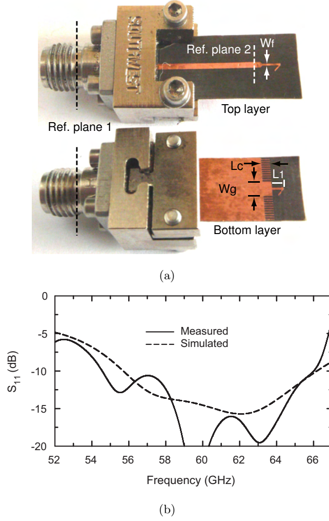
Figure 2.17: (a) Fabricated 60 GHz 45° angled-dipole antenna: W_f = 0.3 , W_g = 2.1 , L_1 = 1.6 , L_c = 1.1 , ground plane width = 8 (all dimensions are in mm), (b) measured and simulated S_{11} at Ref. plane 1.
