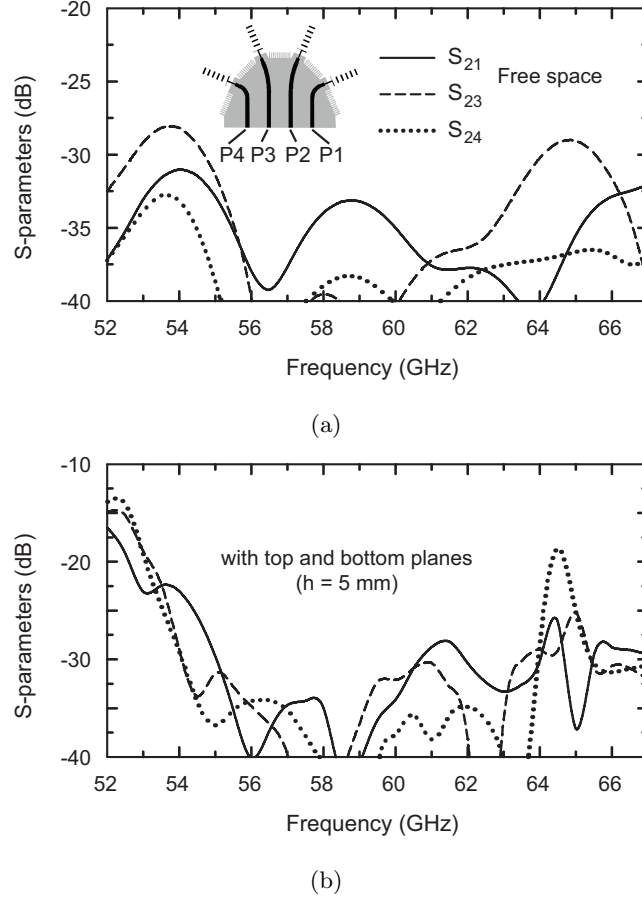
Figure 4.19: Simulated mutual coupling coefficients ( S_{mn} ): (a) in free space, (b) with top and bottom metal planes for h = 5 mm.
