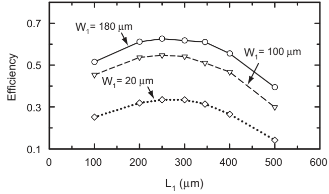
Figure 6.3: HFSS simulated radiation efficiency vs. L_1 and W_1 for h = 125 μm and \epsilon_r = 3.8 .
