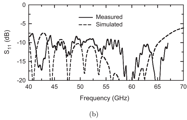
Figure B.1: 40 - 70 GHz Fermi tapered slot antenna (FTSA) with edge corrugations: (a) fabricated prototype, (b) measured and simulated S_{11} .
