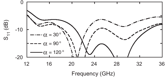
Figure 5.2: Simulated S_{11} of the triangular monopole for three different flare angles.
