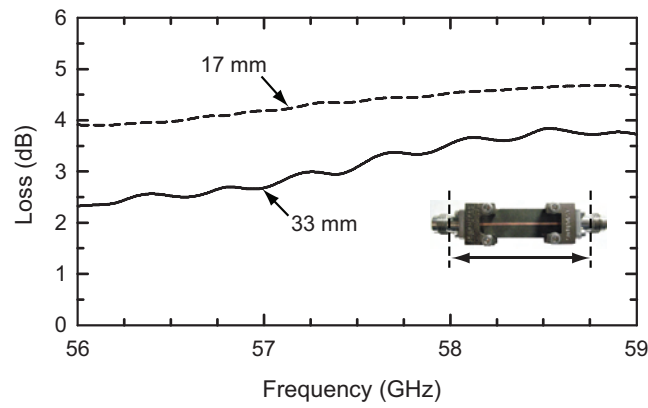
Figure C.4: Measured total loss between S_{11} and S_{22} ref. planes for L = 17 \text{ mm} and L = 33 \text{ mm} .
