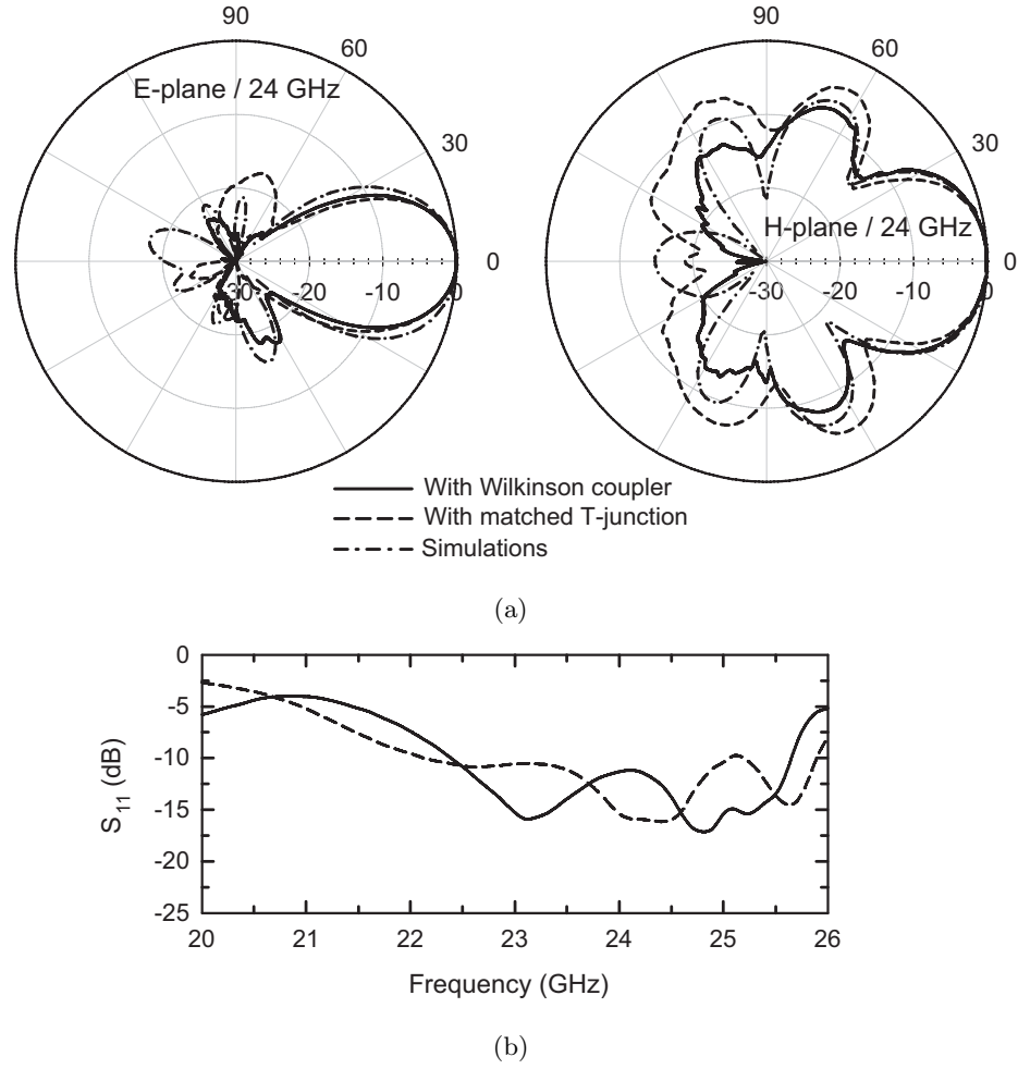
Figure 3.8: (a) Radiation patterns of the two-element arrays, (b) measured S_{11} .
