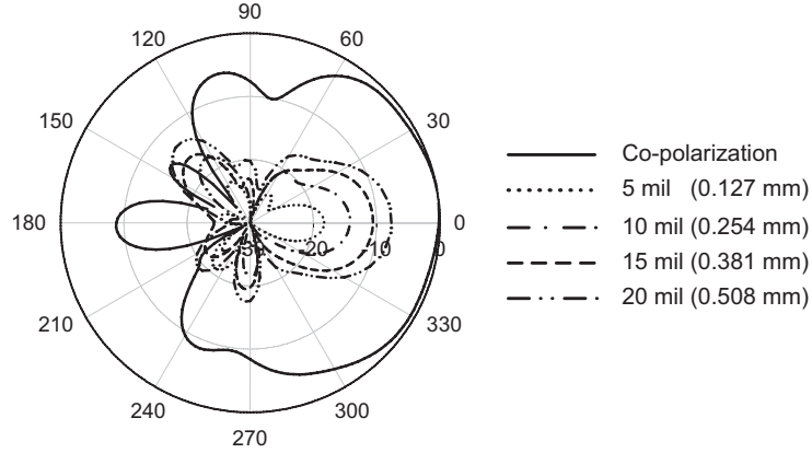
Figure 2.5: Simulated co- and cross-polarization of the 60° angled-dipole at 24 GHz for different substrate thickness.
