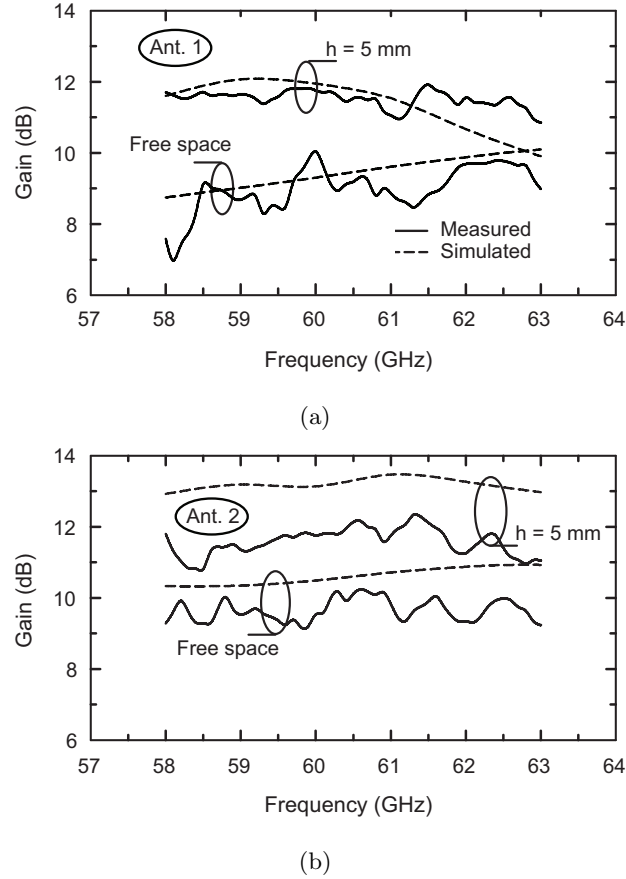
Figure 4.22: Measured and simulated gain of the switched array in free space and with copper sheets above and below ( h = 5 mm): (a) Ant. 1, (b) Ant. 2. Simulations are done with matched ports at all antennas.
