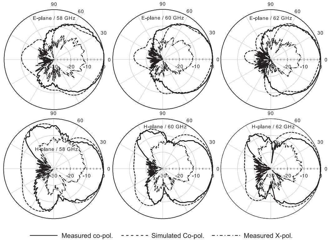
Figure 2.18: Radiation patterns of the 60 GHz 45° angled-dipole antenna.
