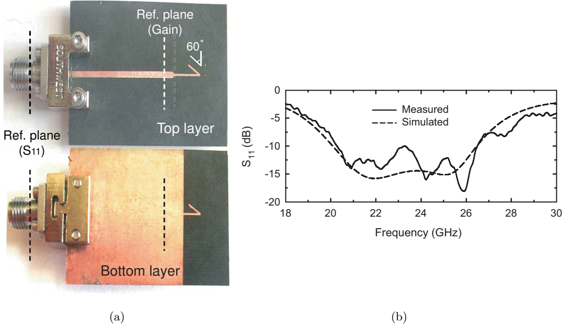
Figure 2.6: (a) Fabricated 60° angled-dipole antenna. The ground plane width is 26 mm and the microstrip line length is 21 mm, (b) measured and simulated S_{11} .
