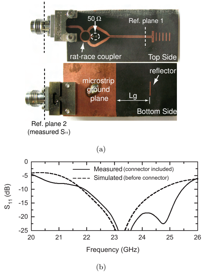
Figure 3.14: (a) Fabricated CPS-fed Yagi-Uda antenna with rat-race coupler, L_g = 14 mm, (b) measured and simulated S_{11} (referenced to 50 \Omega ).
