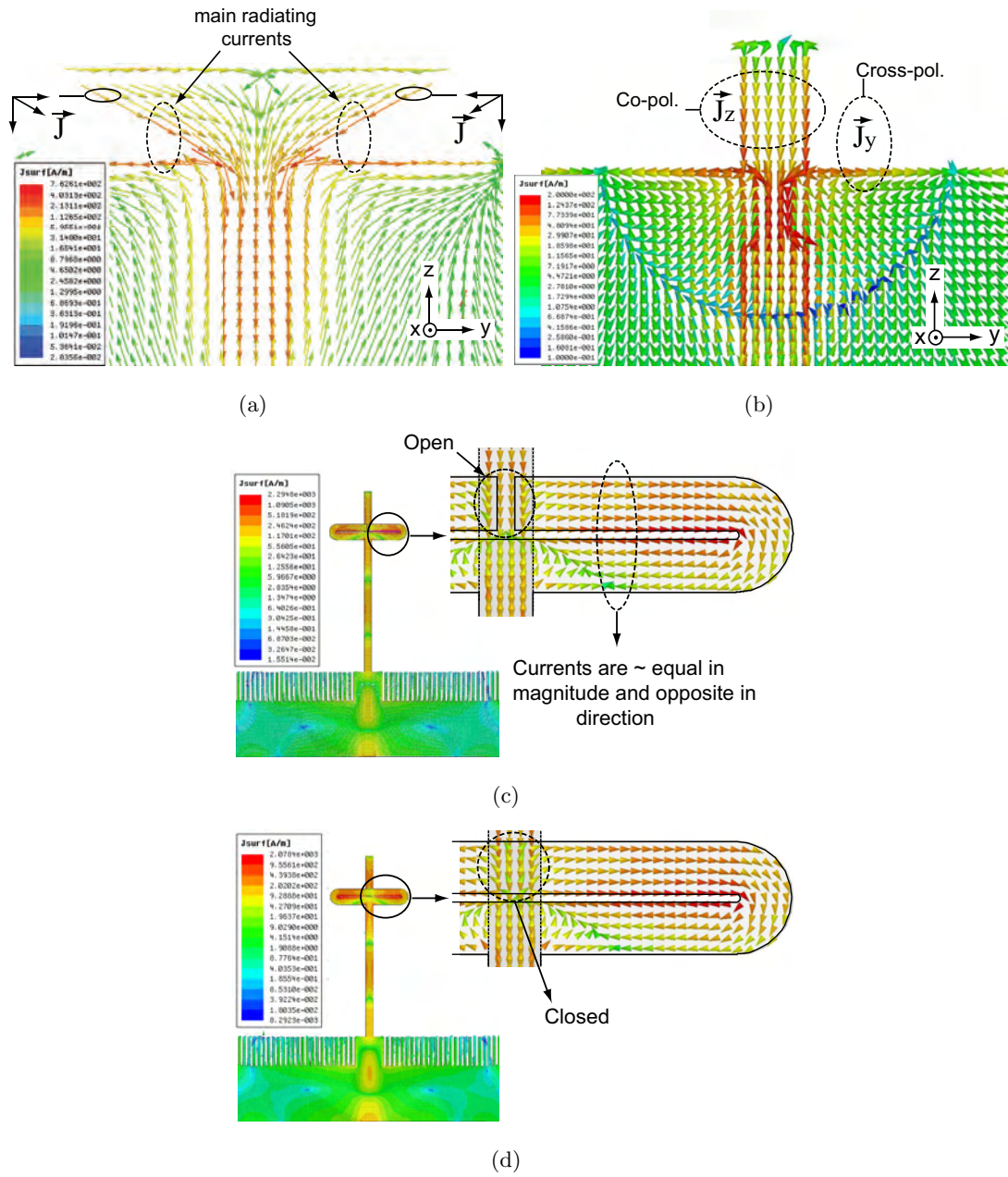
Figure 5.7: HFSS simulated surface current density at 24 GHz on: (a) triangular monopole antenna, (b) straight monopole, (c) modified monopole antenna with magnetic ground plane and with open folded-current choke, (d) with closed folded-current choke.
