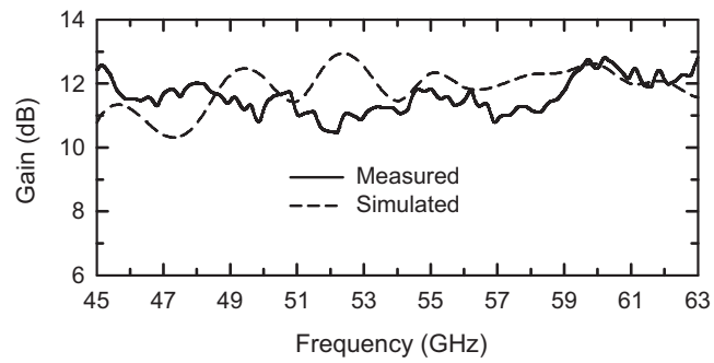
Figure B.3: Measured and simulated gain of the 40 - 70 GHz FTSA antenna.
