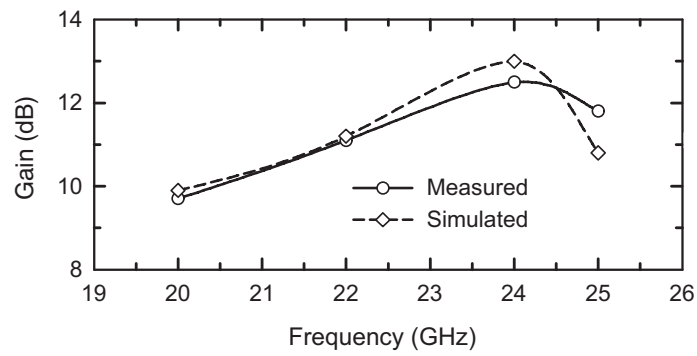
Figure 3.9: Measured and simulated gain of the two element array of the microstrip-fed Yagi-Uda antennas (with Wilkinson coupler) at Ref. plane 2.
