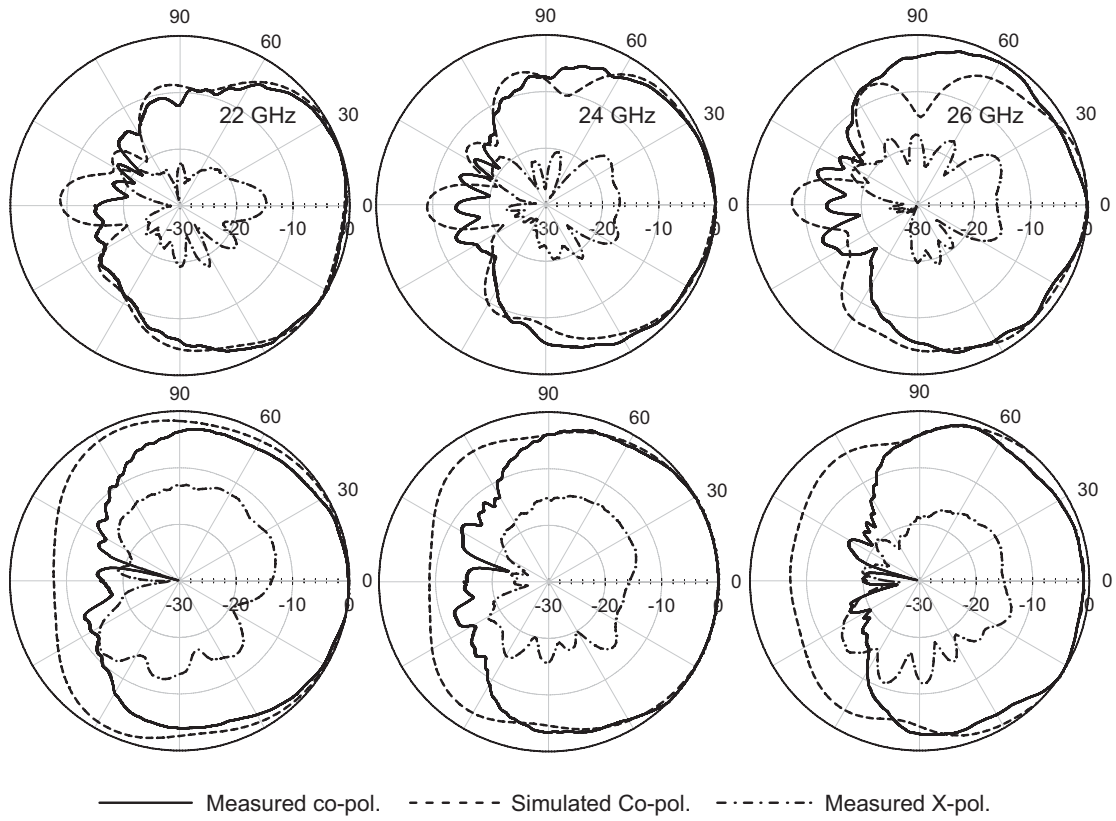
Figure 2.7: E-plane (top) and H-plane (bottom) radiation patterns of the 60° angled-dipole antenna.
