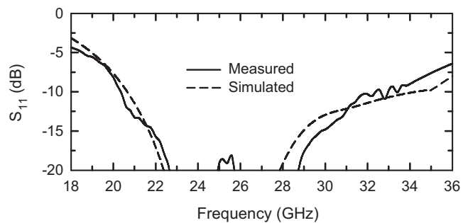
Figure A.2: Measured and simulated S_{11} of the double-dipole antenna.
