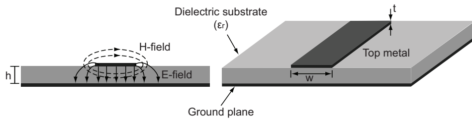
Figure C.1: Microstrip line configuration: front view and field distribution (left), 3-D geometry (right).
