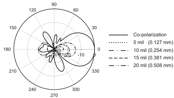
Figure 3.2: Simulated co- and cross-polarization of the microstrip-fed Yagi-Uda antenna at 24 GHz for different substrate thickness.
