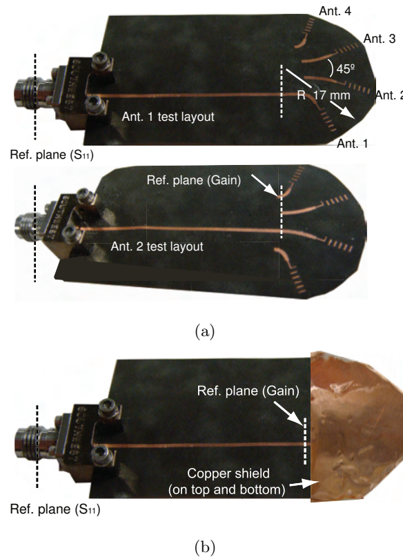
Figure 4.18: Fabricated 4-element switched-beam array of the 60 GHz Yagi-Uda antennas: (a) free space case, (b) with top and bottom shielding planes.
