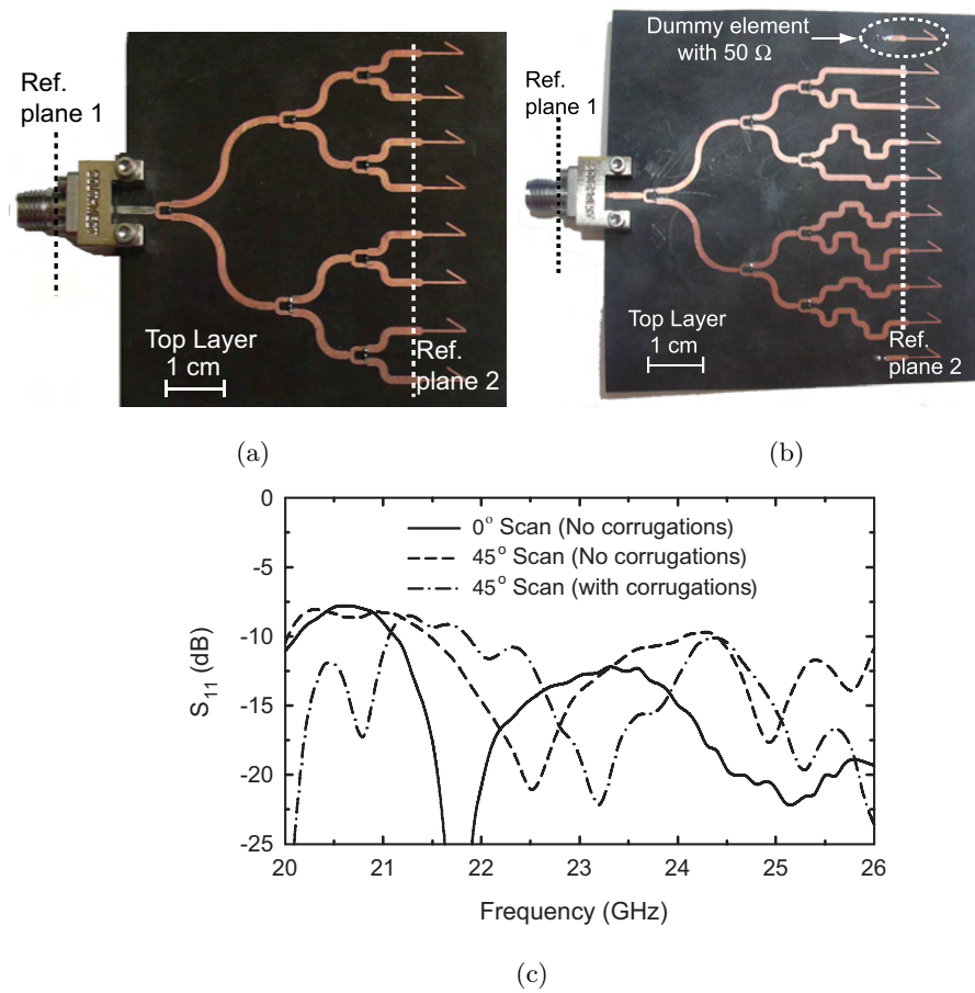
Figure 2.15: Fabricated eight-element array: (a) without scanning, (b) with 45^\circ fixed scan angle at 24 GHz ( 50^\circ scan at 22 GHz), (c) measured S_{11} .
