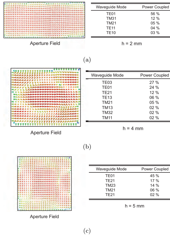
Figure 4.12: HFSS simulated waveguide modes and aperture fields at 60 GHz for: (a) h = 2 mm, (b) h = 4 mm, (c) h = 5 mm.
