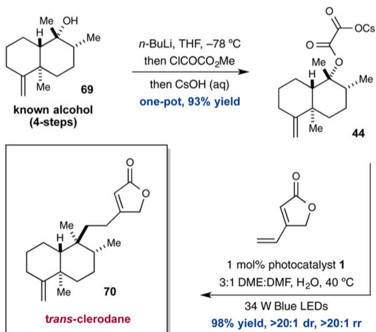
Scheme 2. Six-Step Synthesis of a trans -Clerodane Natural Product
