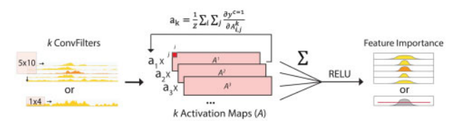
Fig. 2. Grad-CAM for Enhancer Localization: After a positive prediction, we can use Grad-CAM to extract epigenetic features and genomic locations that were important in making the positive prediction. By superimposing activation maps ( A^{k,l} ) weighted by an importance score ( a_k ), Grad-CAM maps highlight the most salient features in making a final output, which we used to generate high resolution core enhancer annotations
