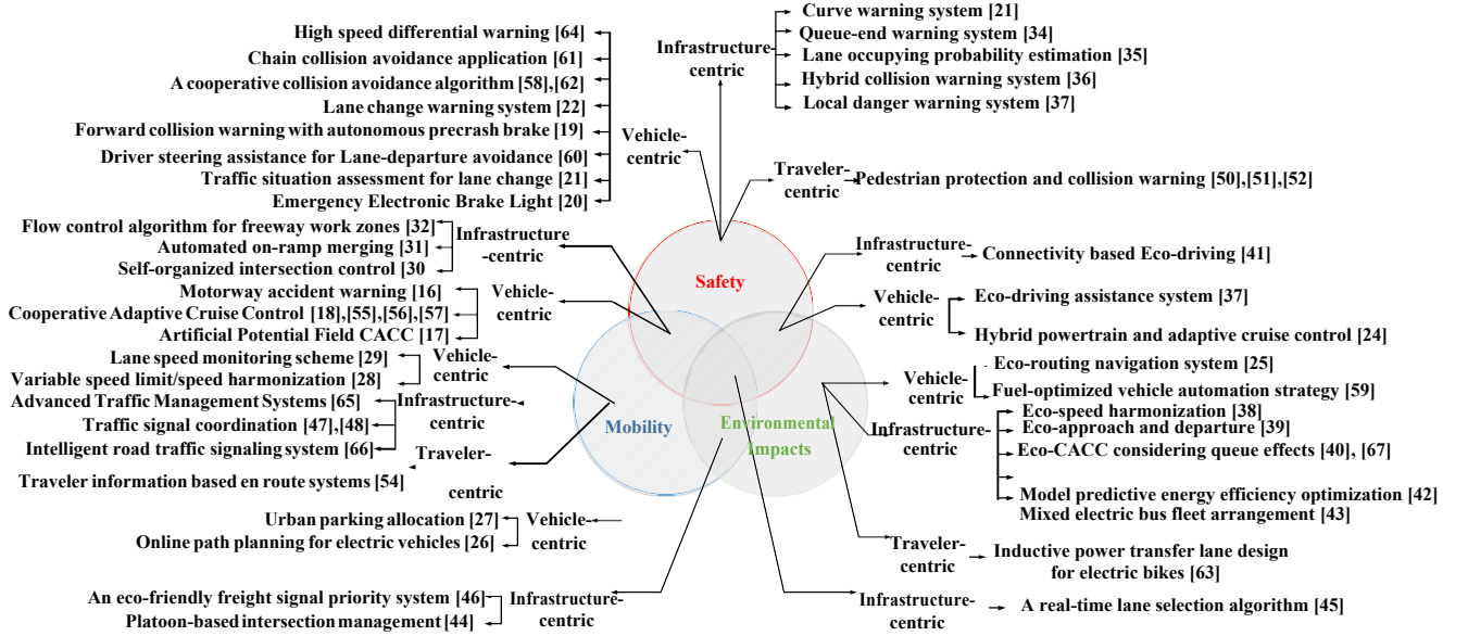
Fig. 2. Taxonomy of CAV applications
