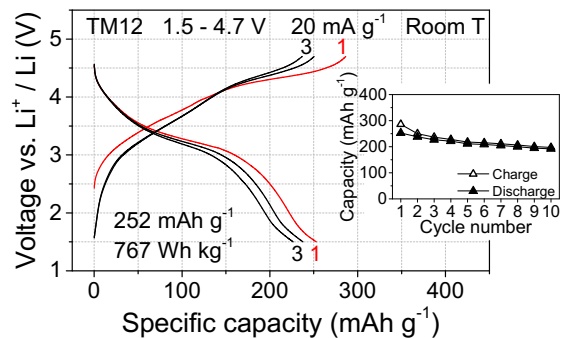
Figure S14 | Electrochemical performance of TM12. Voltage profiles and capacity retention of TM12 within the voltage window of 1.5–4.7 V at 20 mA g -1 and room temperature. Note that the composition of TM12 is not designed for an optimized electrochemical performance, instead, as a demonstration of the excellent structural compatibility of DRX structure. Despite the very diluted TM redox capacity (< 0.35 electron per f.u., corresponding to a capacity of <100 mAh g -1 ) and the incorporation of some very heavy metal ions, such as Ta, and Sb, it still shows reasonably good specific capacity of 252 mAh g -1 .
