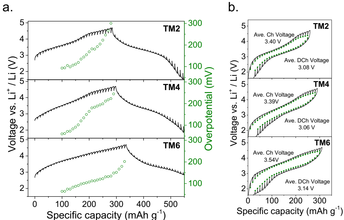
Figure S4 | Voltage profiles of TM2, TM4, and TM6 from GITT tests. Each step in the GITT voltage profiles corresponds to a galvanostatic charge/discharge of 10 \text{ mAh g}^{-1} at a rate of 20 \text{ mA g}^{-1} followed by a 6-h relaxation step. a. First-cycle voltage profiles of TM2, TM4 and TM6. The overpotentials at each step between 100 \text{ mAh g}^{-1} charged states and the top-of-charge states are calculated and plotted as green dots in the figures. b. Second-cycle voltage profiles of TM2, TM4, and TM6 by GITT tests. The green dots mark the quasi-equilibrium voltage at each step. The average voltages after relaxation are calculated and noted in the figure. TM2 and TM4 show similar voltage hysteresis of 0.32\text{V} and 0.33\text{V} , respectively, while TM6 presents a slightly larger voltage hysteresis of 0.40\text{V} . We attribute the slightly larger voltage hysteresis in TM6 to the non-symmetric \text{Cr}^{3+}/\text{Cr}^{6+} oxidation and reduction processes, as discussed in Supplementary Note 4. This phenomenon, induced by \text{Cr}^{6+} migration, was also observed in many other Cr-containing cathodes. 4,5
