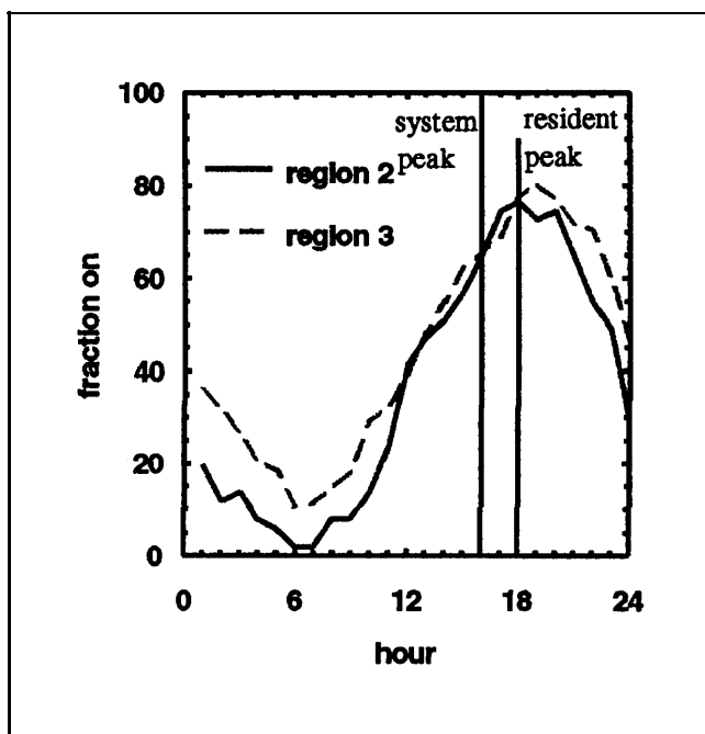
Figure 2. Fraction of the Sample of Residential Air Conditioning Units Which Are on as a Function of Time on the Day of Peak System Demand
