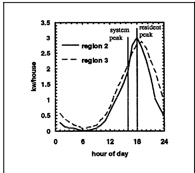
Figure 1. Air Conditioning Demand as a Function of Time for the Day of Peak System Demand. Note the different times for system peak and household air conditioner demand peak.
