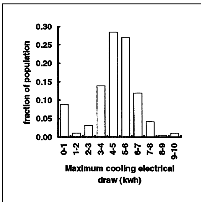
Figure 3. Distribution of the Maximum Cooling Electrical Draw for the Sample Set of Houses in Regions 2 and 3. The average and standard deviation are 4.57 and 1.84 kwh, respectively.
