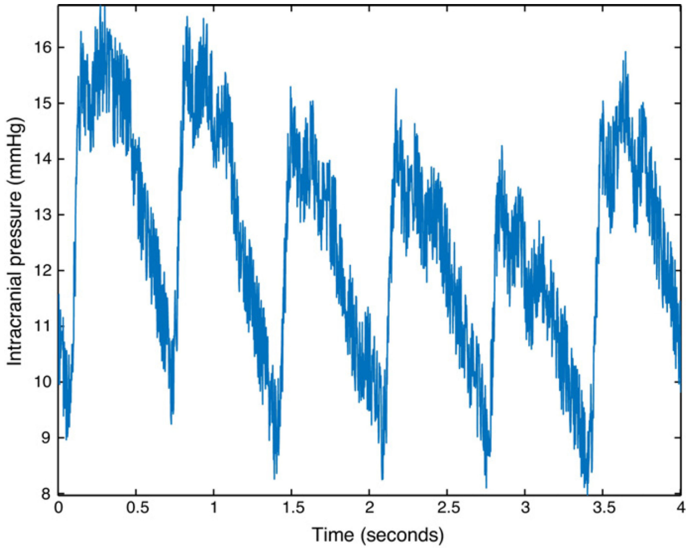
Fig. 1. Illustration of a typical intracranial pressure signal (ICP) recorded in clinical conditions. ICP typically exhibits significant noise on its envelope that challenges its morphological analysis.
