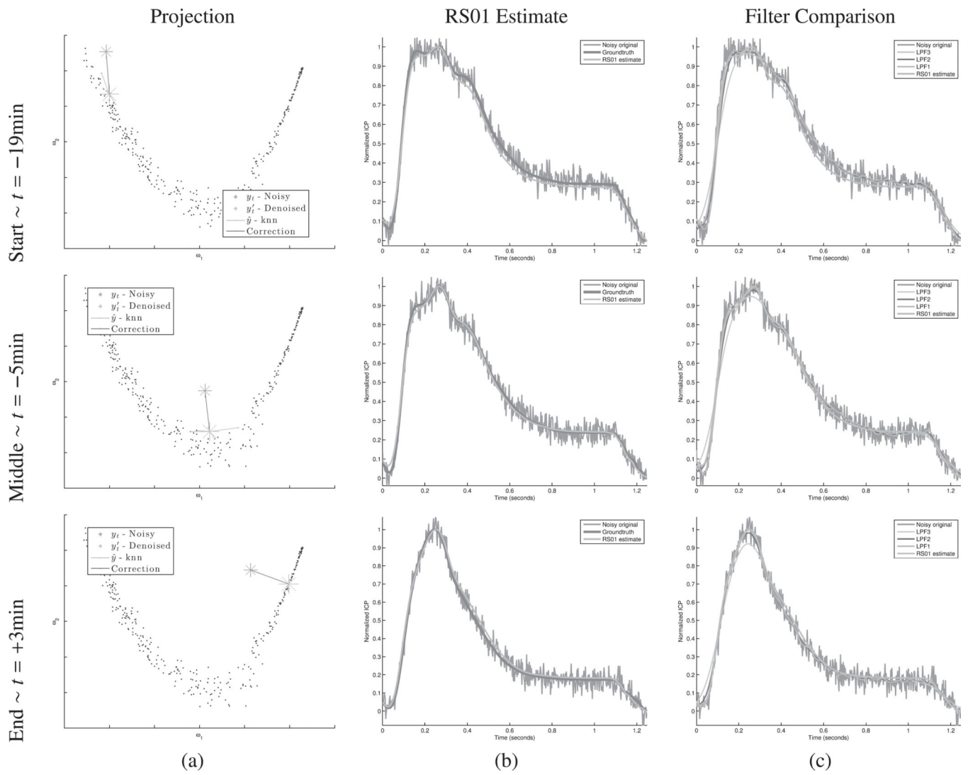
Fig. 6. Denoising of an idealized ICP stream corrupted by AWGN noise of variance \sigma = 4\% . (a) Signals are projected to the subspace and (b) denoised using the RS01 algorithm using geodesic constraints. (c) The estimate is compared to various generic filters.
