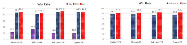
Figure 4: Results of the win rate in the evaluation of instruction-following ability were compared between the model tuned for All instruction data and the model tuned for Pithy data with the addition of noise embedding using GPT4 on a 500K dataset in the cybersecurity domain. It is worth noting that the Pithy instruction data used only 6% instruction data.
