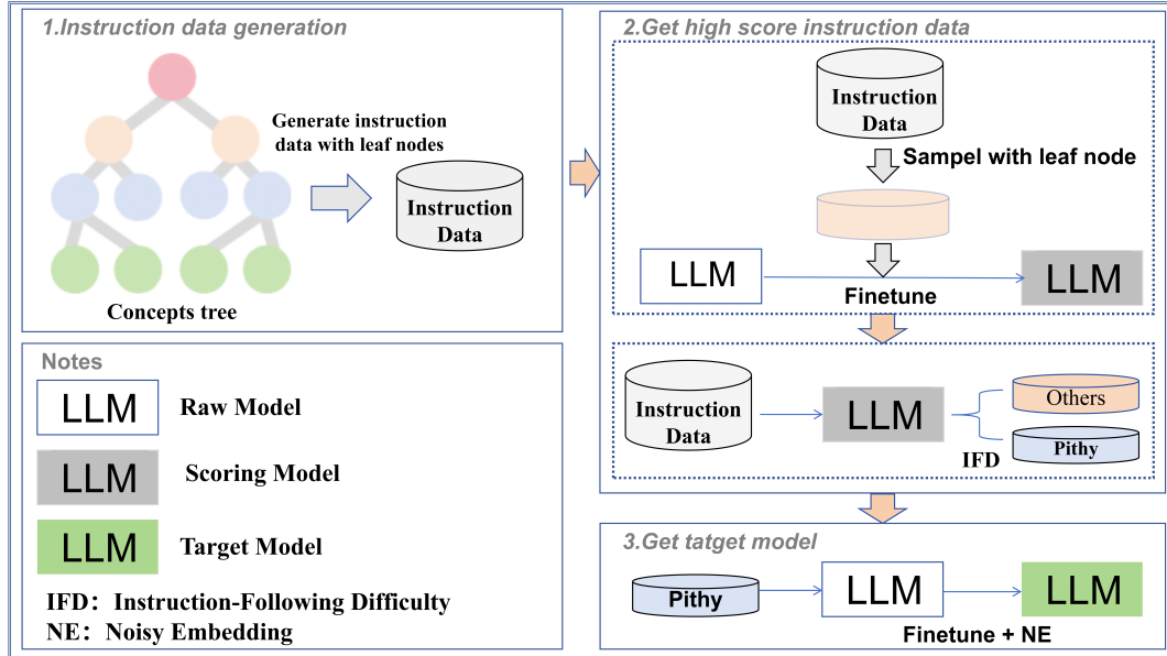
Figure 2: Framework of UNIFIT. It consists of three parts: instruction data generation using Concept Trees, filtering high-quality instruction data(Pithy) through instruction following difficulty(IFD), and instruction tuning with the addition of noise embedding(NE). Specific details are available at Methodology
