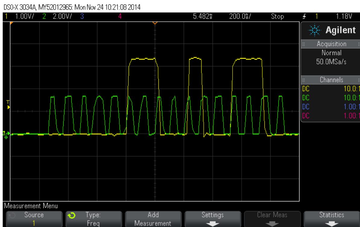
Figure 4-7: Data output at the SPI line
