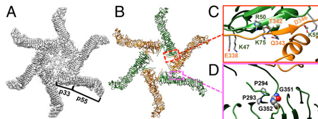
Fig. 3. Interactions between VacA protomers in the hexamer (OA-1). (A) Cryo-EM map of the VacA hexamer. (B) Model of the VacA hexamer. (C) The protomer–protomer intermolecular interactions including multiple side-chain hydrogen bonds and salt bridges. (D) The 293 ProPro 294 and 351 GlyGly 352 motifs (28) probably control the orientation of the protruding segment from p55. The glycines are shown in sphere and colored by element for clarity.
