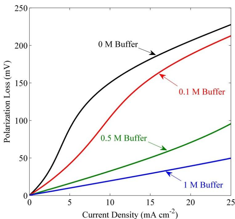
Figure 6: Polarization loss versus current density for 0.1 M, 0.5 M, and 1 M buffered electrolyte. Operating conditions: pH 7.8, 1 M KHCO_3 , no membrane, i_l = 10 \text{ mA cm}^{-2} , p_{CO_2} = 1 \text{ atm} , boundary layer thickness = 100 \text{ }\mu\text{m} , and k_l a \delta = 0.33 \text{ s}^{-1} .
