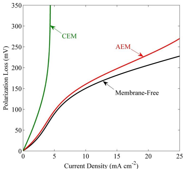
Figure 9: Comparison of polarization losses in the membrane-free 1M KHCO 3 electrolyte with the electrolyte separated by an anion exchange membrane (AEM) and a cation exchange membrane (CEM). Operating conditions: pH 7.8, 1 M KHCO 3 , p_{\text{CO}_2} = 1 \text{ atm} , boundary layer thickness = 100 \mu\text{m} , and k_1 a \delta = 0.33 \text{ s}^{-1} .
