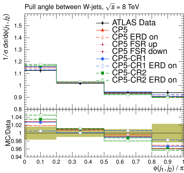
Fig. 20 Normalised \bar{t}\bar{t} differential cross section for the pull angle between jets from the W boson in top quark decays, calculated from the charged constituents of the jets, measured by the ATLAS experiment using \sqrt{s} = 8 TeV data [58] to investigate colour flow. The coloured band and error bars on the data points represent the total experimental uncertainty in the data
