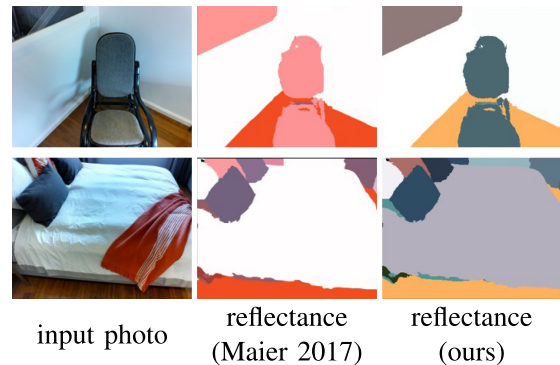
FIGURE 7. Comparison of our differential rendering enabled material reconstruction 4 with a traditional computer vision method. 31 We obtain higher fidelity reconstruction due to the ability to account for interreflections and shadows.
