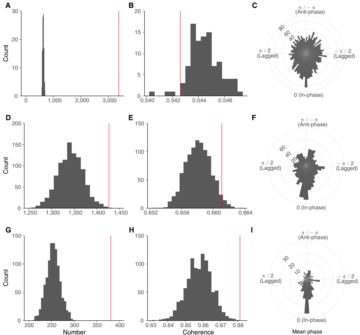
Fig. 2. Histograms of coherent relationships in fishery catches across spatial scales. (A, D, and G) Number of significant coherent relationships (count) observed (red line) and expected from a null model (gray histogram) globally (A), within ocean basins (D), and within FAO regions (G). (B, E, and H) Average coherence values observed (red line) and expected from a null model (gray histogram) globally (B), within ocean basins (E), and within FAO regions (H). (C, F, and I) Circular histogram of average phase relationships among the significant, coherent relationships globally (C), within ocean basins (F), and within FAO regions (I). For all plots, significance was defined with a false discovery rate of <20\% . See Appendix S1: Fig. S2 for an alternative null model.
