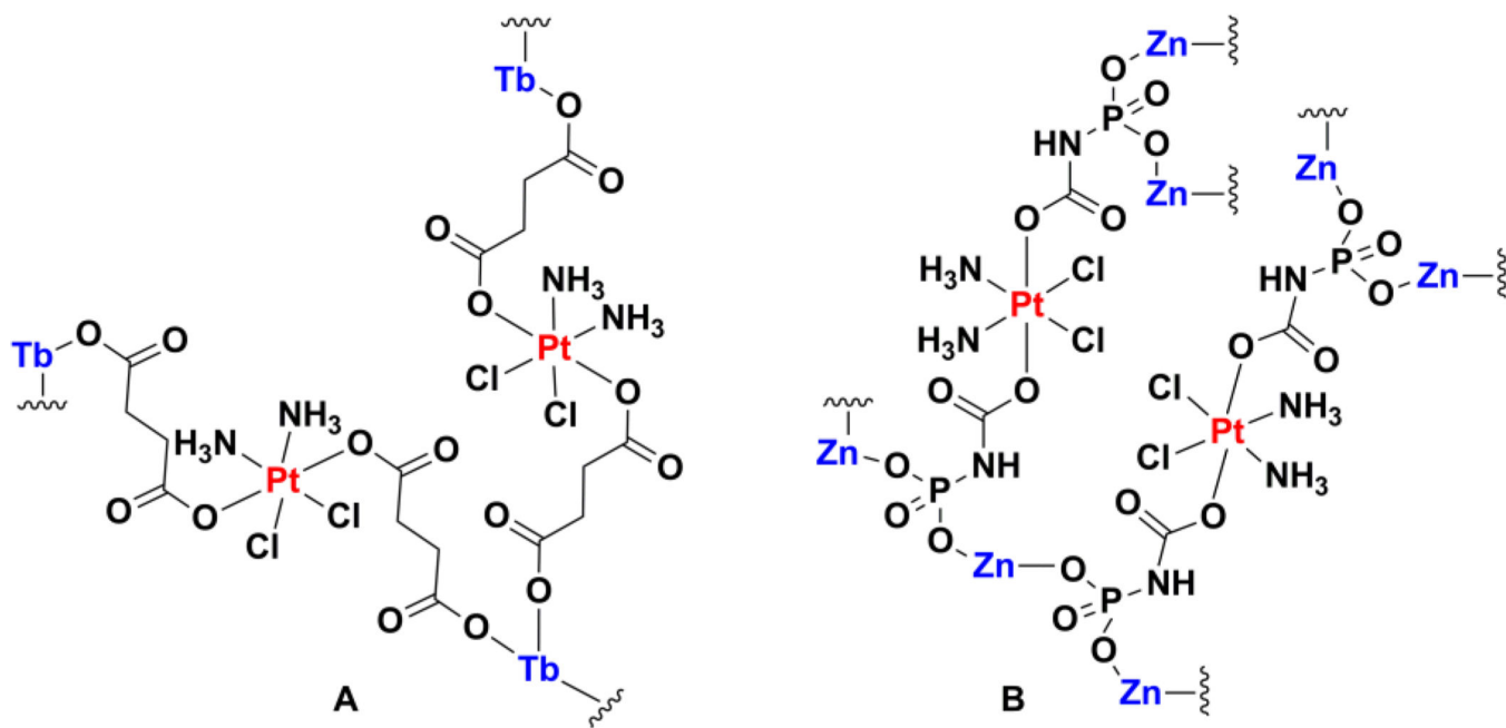
Chart 21. Depiction of the formation of coordination polymers using metal units to link platinum(IV) prodrugs bearing axial ligands with coordinating motifs.
