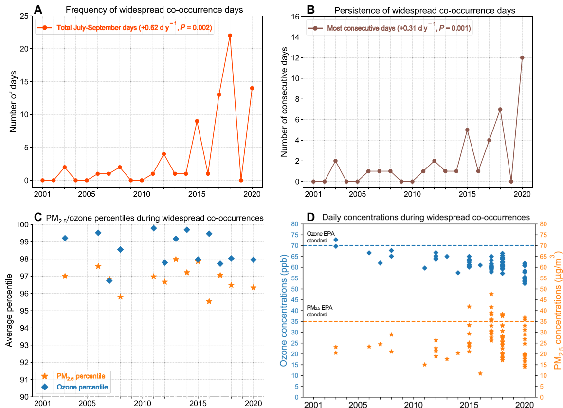
Fig. 2. Widespread \text{PM}_{2.5} /ozone co-occurrences. Time series of (A) the total number and (B) longest consecutive-day persistence of widespread July to September co-occurrence days, defined as days with simultaneous local \text{PM}_{2.5} /ozone co-occurrence in \geq 25\% of western US grid cells. Text in (A) and (B) indicates linear trends ( \text{d y}^{-1} ) with P values based on a permutation test. Characteristics of the individual pollutants during widespread co-occurrences are shown through (C) percentiles of \text{PM}_{2.5} and ozone daily concentrations averaged across all affected grid cells and (D) pollutant concentrations averaged across affected grid cells on widespread co-occurrence days ( n = 72 ). Note that percentiles in (C) are calculated on the basis of the distribution of concentrations in each year (refer to Materials and Methods). Dashed lines in (D) show concentrations corresponding to the Environmental Protection Agency (EPA) regulatory health standards for each pollutant [70 parts per billion (ppb) for ozone and 35 \mu\text{g}/\text{m}^3 for \text{PM}_{2.5} ].
