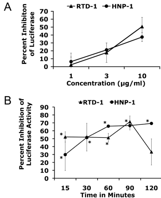
Figure 1. HNP-1 and RTD-1 inhibited luciferase activity in a concentration dependent manner. (A) 293T cells transfected with CDM8-luc were lysed 48 hours post transfection and then cell lysates were incubated with HNP-1 or RTD-1, at 0, 1, 3, or 10 \mu g/ml on ice for 1 hour and luciferase activity was measured. (B) HNP-1 and RTD-1 were added to lysates of 293T cells transfected with CDM8-luc. Cell lysates were incubated with 10 \mu g/ml HNP-1 or RTD-1 on ice for 15, 30, 60, 90, or 120 minutes and luciferase activity was measured. The data points in (A) and (B) represent triplicate samples from two experiments. Error bars show standard deviations from the mean. Asterisks represent p < 0.01 by Student's t-test compared to buffer only. doi:10.1371/journal.pone.0009737.g001
