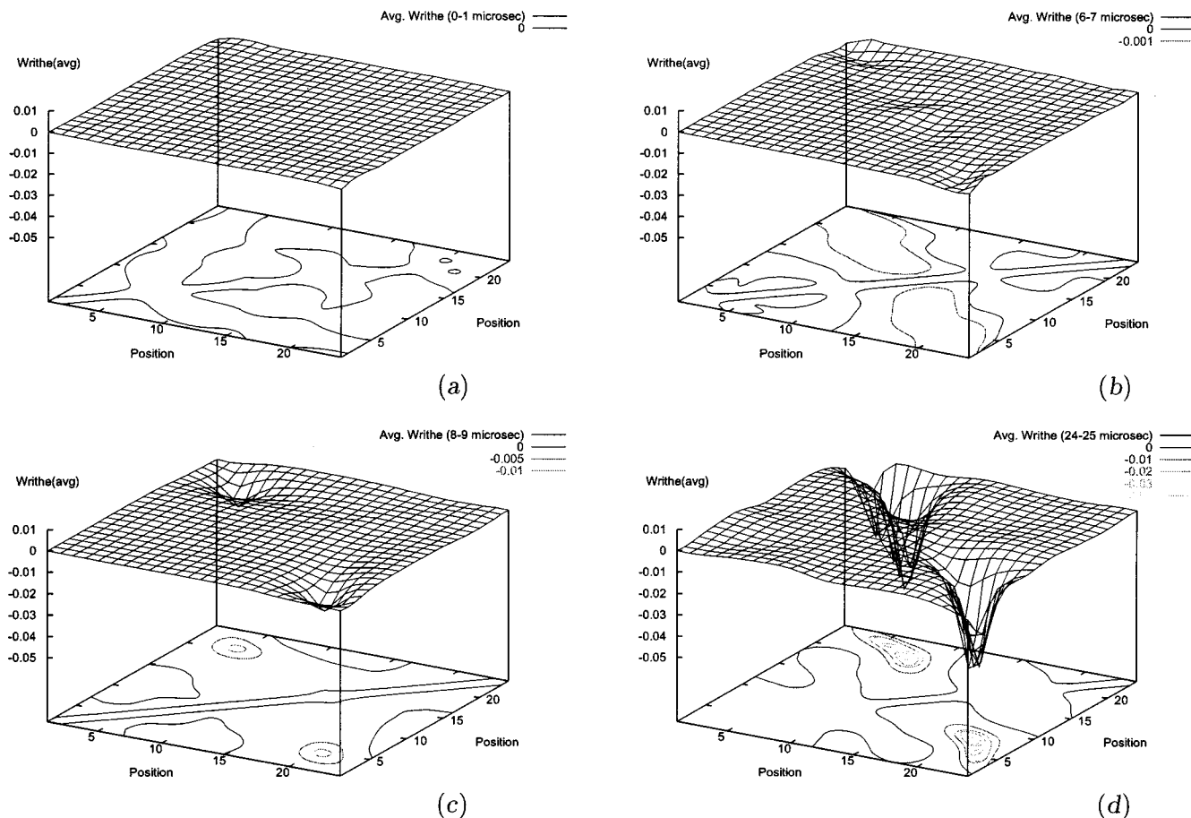
FIG. 5. Time-averaged writhe densities for S^- from 0 to 25 \mu s: (a) 0–1 \mu s; (b) 6–7 \mu s; (c) 8–9 \mu s; (d) 24–25 \mu s. Contours in the base planes are two-dimensional (2D) projections of the writhe surfaces, with elevations indicated. The buckling event evident in c leads to a plectonemically supercoiled structure, represented in d , where the crossings of maximal writhe are \{5,23\} = -0.05325 and \{9,19\} = -0.05721 (see contour map). These crossings correspond to locations of self-contact in the structure at 25 \mu s (refer to discussion and Fig. 7).
