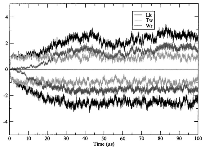
FIG. 4. Linking number Lk , twist Tw , and writhe Wr from 0 to 100 \mu\text{s} . All quantities remain nearly constant on average after \approx 25 \mu\text{s} .
