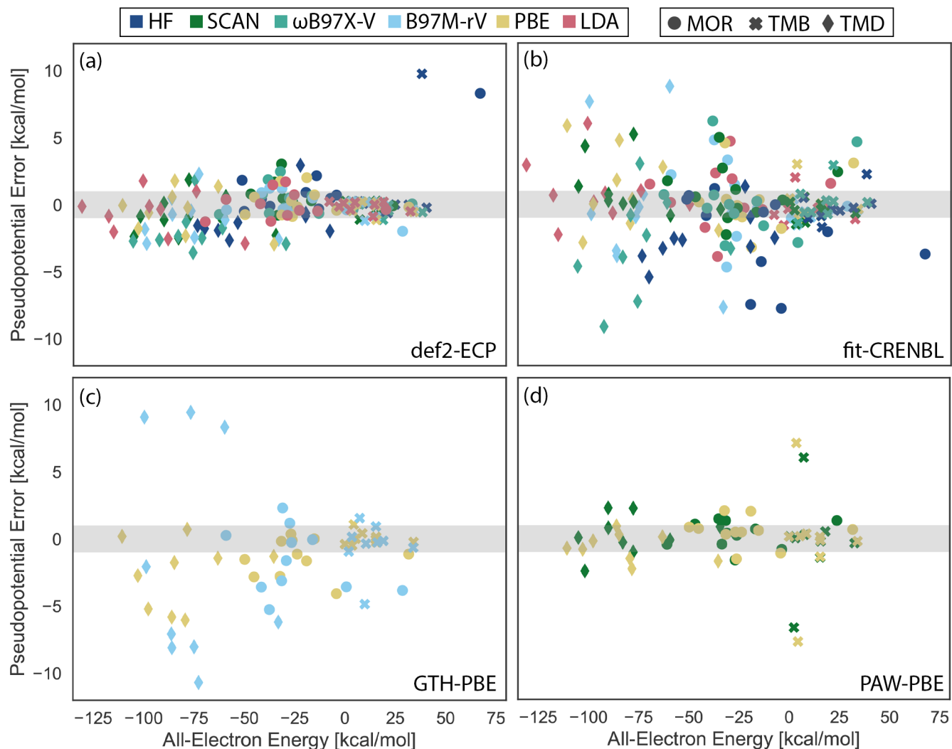
Figure 3: Pseudopotential errors [kcal/mol] for (a) def2-ECP, (b) fit-CRENBL, (c) GTH-PBE, and (d) PAW-PBE for the TMC34 data set of transition metal containing energy changes. TMC34 contains 3 subsets: barrier heights (TMB; crosses), reaction energies (MOR; circles) and dimer bond strengths (TMD; diamonds). Errors generally increase from TMB to MOR to TMD. Gray bands correspond to chemical accuracy of \pm 1 kcal mol ^{-1} . Outliers and other aspects of the data are discussed in the text.
