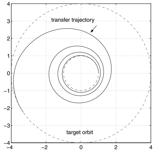
Fig. 12 An antialiased 30-node closed-loop transfer trajectory for problem min T.
