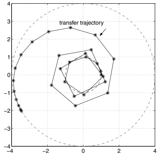
Fig. 11 A 30-node open-loop transfer trajectory for problem min T.
