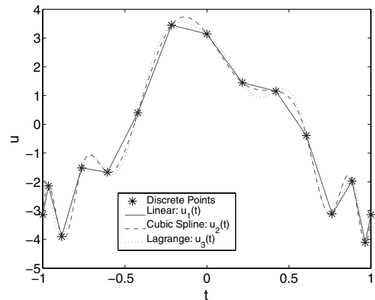
Fig. 4 Continuous-time reconstructions of a control trajectory using various interpolation schemes.
