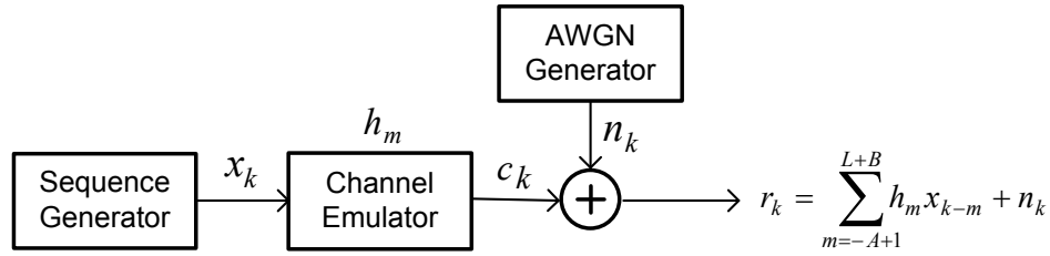
(a) Transmitter and the channel
