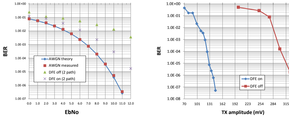
(a) BER curves from the digital loop-back
