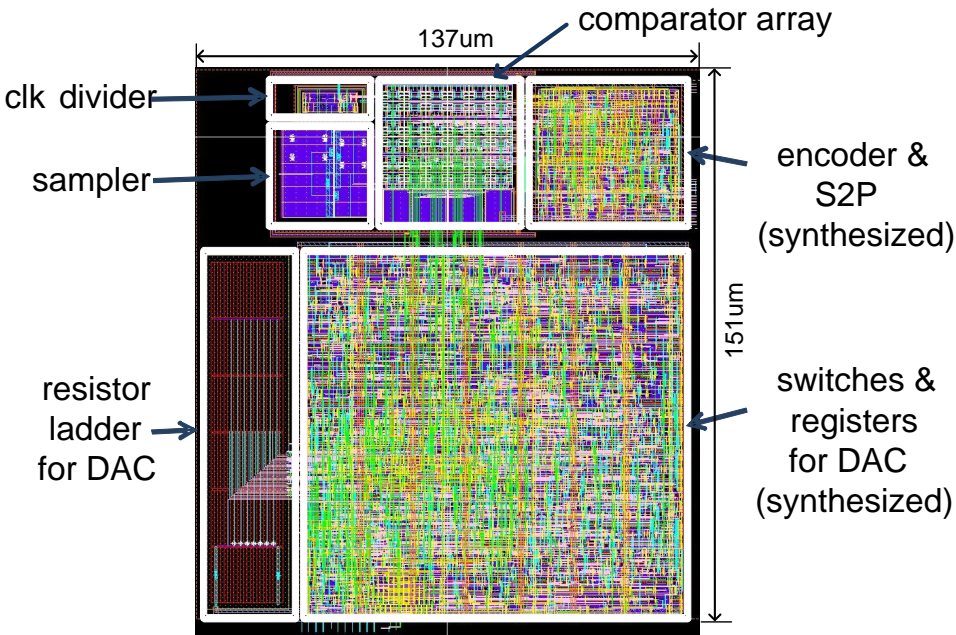
Figure 6.7: ADC layout.
