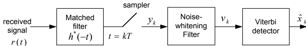
Figure 3.4: Optimum receiver for an ISI channel and AWGN [66].
