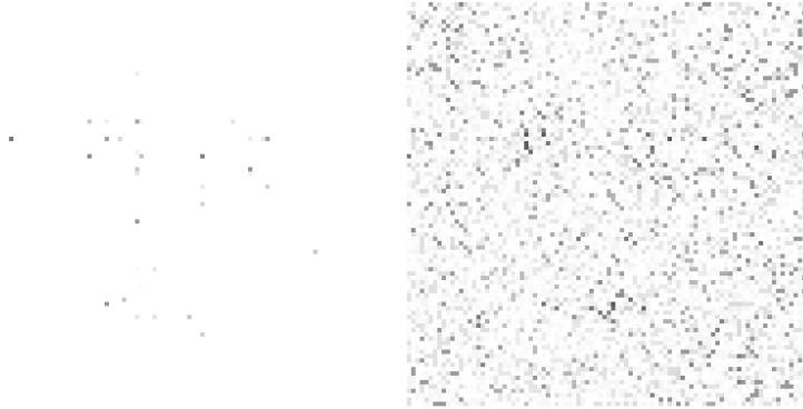
Figure 2.1: Two malicious images we generated with our algorithms. The left image is detected as a face if fed directly into a face detector. The right image is detected as a face, even after it is subjected to distortions imposed by the physical world: When displayed on a tablet and captured using a camera, the resulting image is detected as a face 97% of the time.
