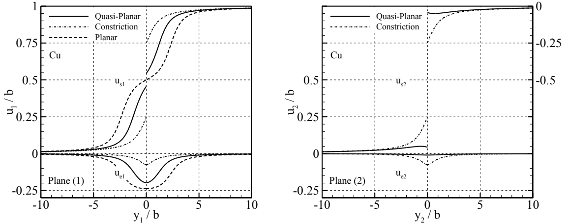
Figure 4-9. In Cu, due to the lower intrinsic stacking fault energy and larger stacking fault zone, the core of a screw dislocation prefers to be quasi-planar and stays in the primary slip plane. The figure shows both screw and edge components on the primary slip plane (left) and the cross-slip plane (right), as compared with planar and constricted core structures
