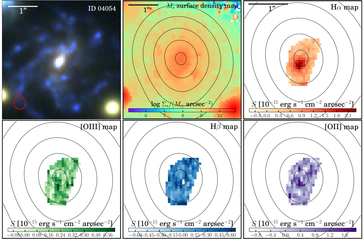
Figure 3.3 Multi-perspective view of the SN Refsdal host galaxy multiple image 1.3, i.e., ID 04054 in our metallicity gradient sample. Upper left : zoom-in color composite stamp cut out from Figure 3.1, where the estimated site of the un-observed past appearance of SN Refsdal is denoted by the red circle. Upper middle : stellar mass surface density map for this galaxy, where the source plane de-projected galactocentric radius contours are overlaid, in 2 kpc intervals, starting from 1 kpc. Upper right : H\alpha surface brightness map combined from the HST grism exposures at all PAs from the GLASS and Refsdal follow-up programs. The black contours again show the de-projected galactocentric radii in the same fashion presented in the stellar mass surface density map in the upper middle panel. Lower rows : combined surface brightness maps of [O III], H\beta , and [O II], presented in the same fashion as in the H\alpha emission line map in the upper right panel.
