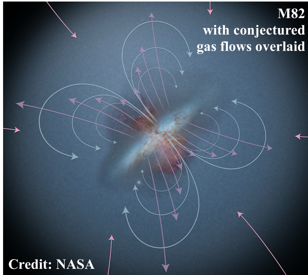
Figure 1.1 Onset of baryon cycling in the local Universe: the Messier 82 galaxy. Overlaid are the conjectured movements of gas in and around this galaxy undergoing active star formation.
