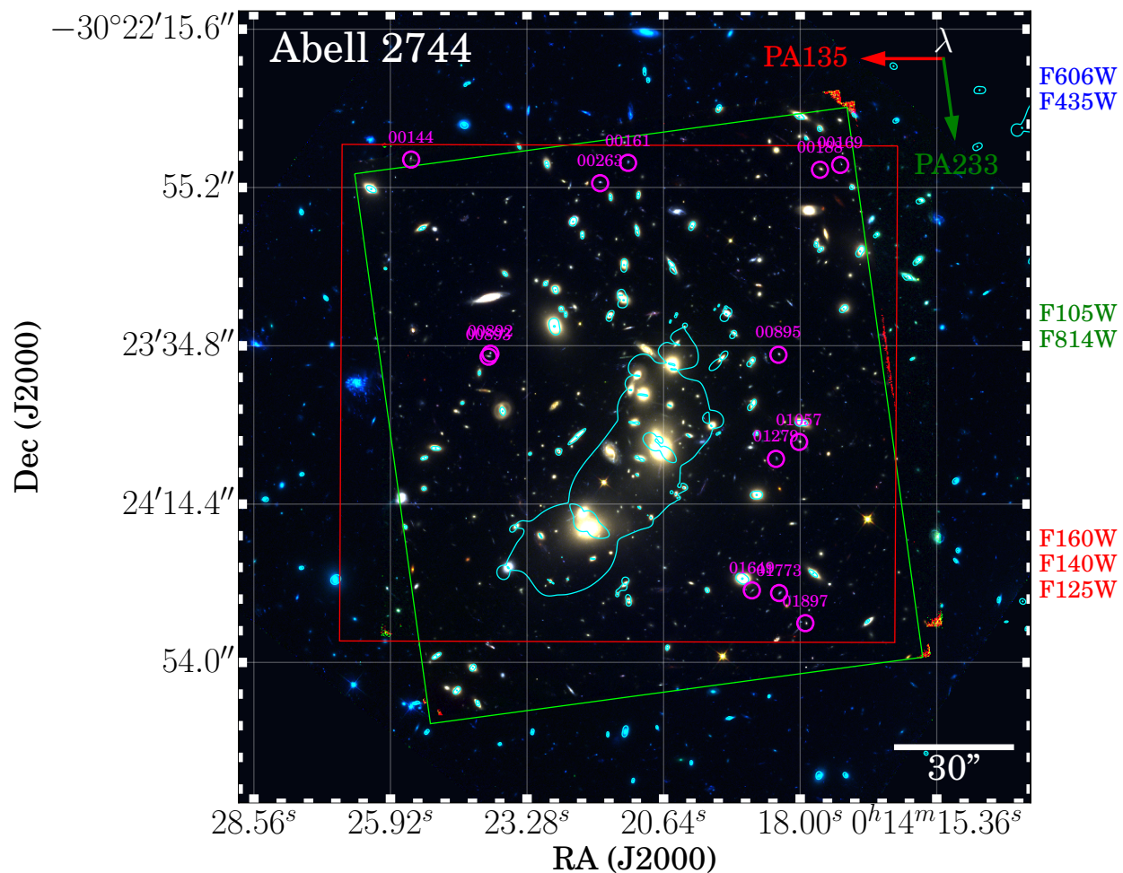
Figure 5.1 The color-composite images of the galaxy cluster centers exposed by HST WFC3/NIR grism elements (10 orbits of G102 and 4 orbits of G141) from the GLASS program. The entire amount of exposure time is equally deposited into 2 separate pointings represented by the red and green squares with light dispersion directions denoted by the arrows in the upper right corner. The sample of star-forming galaxies in which I secure unbiased measurements of metallicity radial gradients are marked by magenta circles. The cyan contours are the critical curves at sample median redshift.
