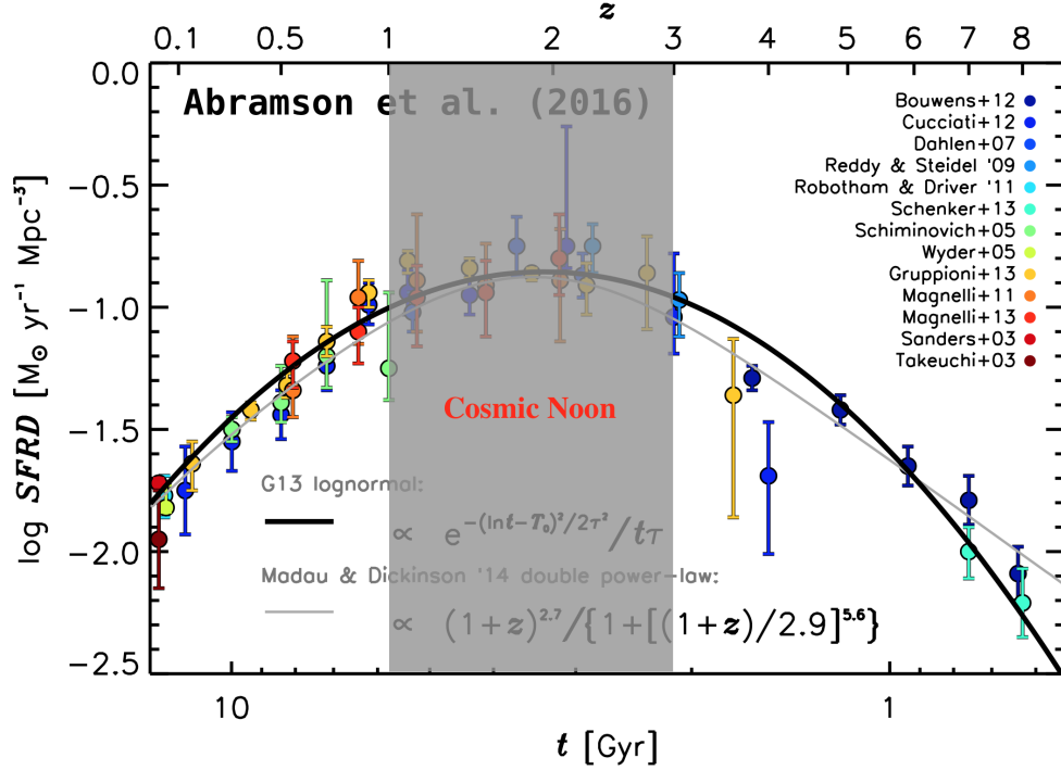
Figure 1.2 The rise and fall of the cosmic average star-formation rate density. The grey shaded region marks the peak epoch of cosmic star formation, usually coined the “cosmic noon”. At the cosmic noon, our Universe assembled roughly one half of its present day stellar mass using less than one third of its age. Figure credit: Abramson et al. (2016).
