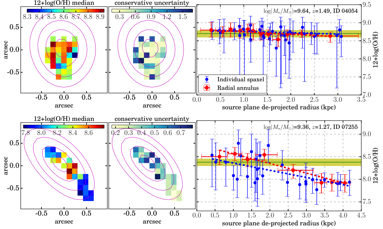
Figure 3.10 Maps of metallicity constraints (median value in the left column and conservative uncertainty — the larger side of asymmetric 1\text{-}\sigma error bars — in the center column) and plots of radial metallicity gradients in the right column. Note that unlike what we show in the combined EL maps (Figures 3.3 and 3.4), here the metallicity maps are rebinned to a scale of 0''.13 , corresponding to the native resolution of WFC3/IR. In the maps, only spaxels with the signal-to-noise ratio of \text{H}\alpha or [\text{O III}] larger than 5 are shown. The same source plane de-projected galactocentric radii that are denoted by black contours in Figures 3.3 and 3.4 are represented by magenta contours, with the only difference being that contours are in 1 kpc intervals now. In the panels in the right column, blue and red points correspond to metallicity measurements for individual spaxels and radial annuli, respectively. The radial gradients derived based upon these measurements are shown by the dashed lines in corresponding colors. The yellow band and green horizontal line mark the global constraint on 12 + \log(\text{O}/\text{H}) , from integrated line fluxes.
