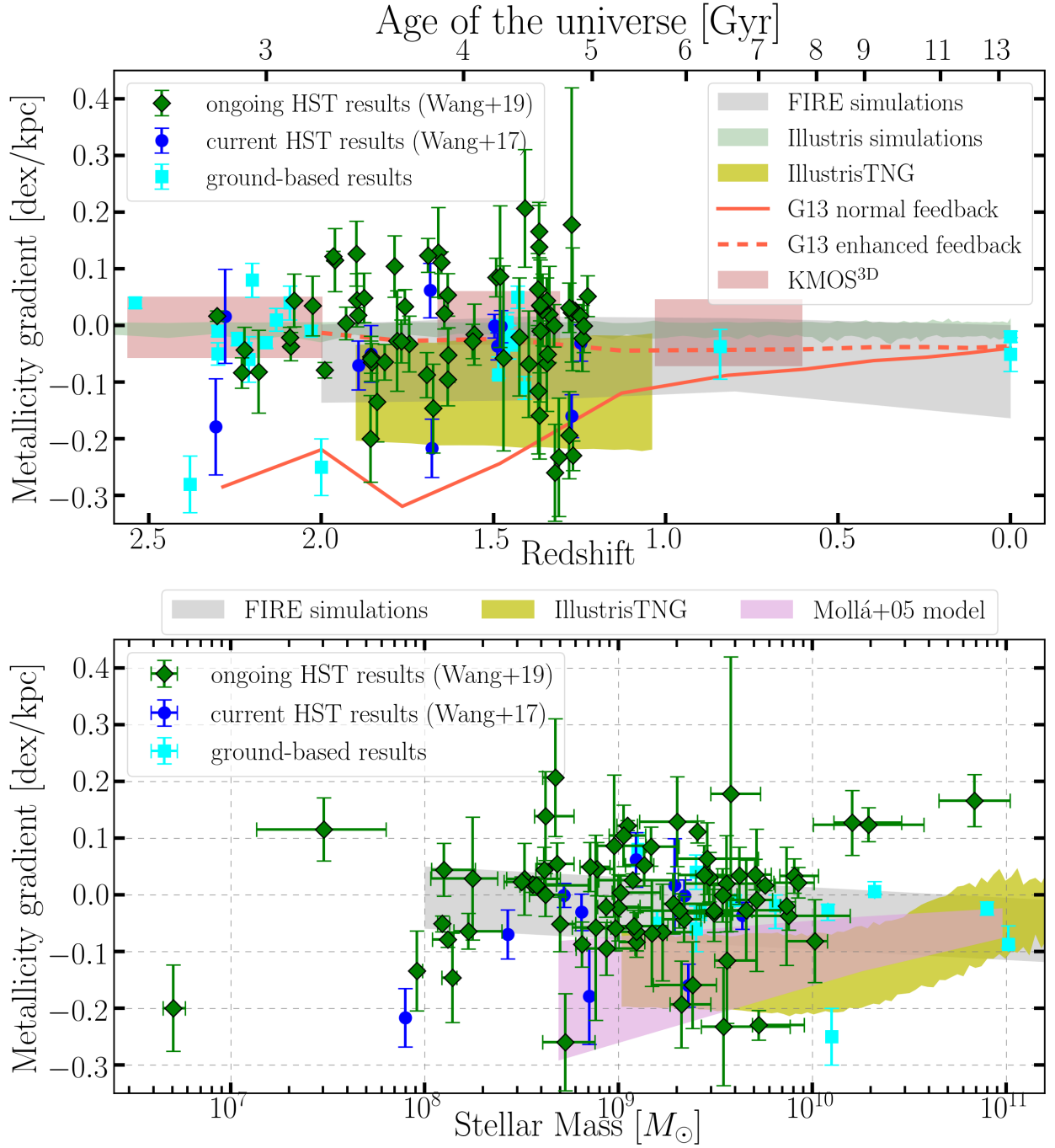
Figure 5.2 The redshift evolution and mass dependence of all metallicity gradients in high- z star-forming galaxies measured at sub-kpc resolution, unbiased from the beam smearing effect. It is obvious that my analysis results based on the combination of HST WFC3/NIR grism slitless spectroscopy and lensing magnification constitute a major portion of all these measurements.
