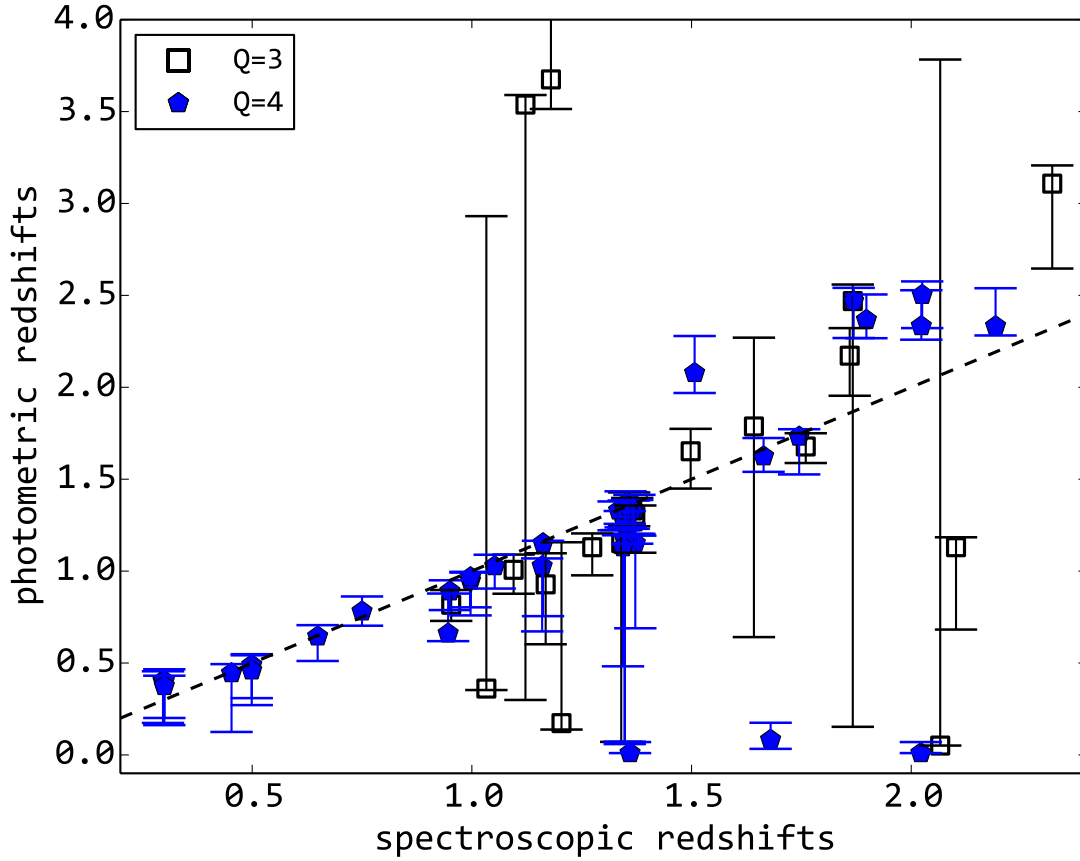
Figure 2.10 Comparison between the spectroscopic and photometric redshifts for the 55 objects with high-confidence emission lines (quality flags 3 or 4). We also show the 1\text{-}\sigma error bars (enclosing 68% of the total probability) around the photometric redshifts. There is reasonably good agreement between photometric and spectroscopic redshifts, with 25 out of 55 spectroscopic redshifts within the photometric redshift error bars. This is acceptable considering that the photometric redshift uncertainties only include the random component, even though they suggest that an additional systematic uncertainty component is present. In order to account for this systematic uncertainty, for the systems used to build the lens model we added 20% in quadrature to our photometric errors.
