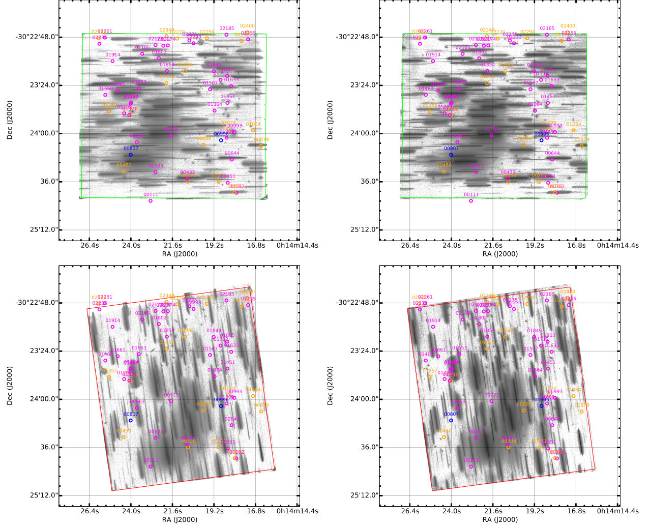
Figure 2.2 The GLASS G102 (left) and G141 (right) grism pointings of Abell 2744 at two distinct P.A.s, with field-of-view shown by the red (P.A.=233 degrees) and green (P.A.=135 degrees) squares. The circles in all panels denote the positions of the emission line objects identified in this work, with color coding following the convention adopted in Figure 2.1.
