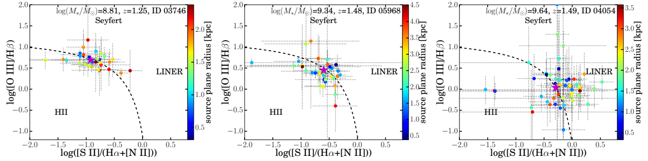
Figure 3.11 Spatially resolved BPT diagrams for three representative sources in our metallicity gradient sample. The points in each panel correspond to spaxels in the combined EL maps for each source, color coded by the source plane de-projected galactocentric radius. Note that similar to what we show in Figure 4.3, all spaxels represented by colored points here are rebinned to recover the native WFC3/IR pixel scale ( 0''.13 ). The magenta star denotes the position where the entire galaxy would lie, calculated from integrated EL fluxes, with the length of the error bar comparable to the size of the symbol. The dashed curve is adapted from the extreme starburst scenario given by Kewley et al. (2006b), assuming the “vanilla” value for [N\ II]/H\alpha . Given the 1-\sigma uncertainties, all the spaxels are broadly consistent with being HII regions.
