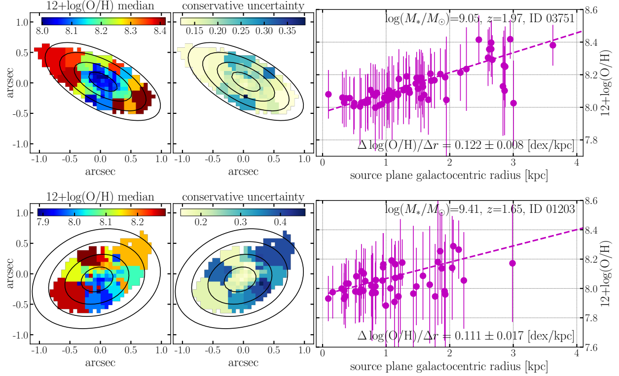
Figure 4.3 Metallicity maps and radial gradient measurements of the two galaxies. The left panels show the 2D maps of the median value estimates of metallicity, and the central panels show their conservative uncertainties (i.e. the larger side of the asymmetric 1-\sigma error bars). The right panels show the corresponding radial gradients measurements. The black contours again mark the source plane de-projected galacto-centric distances as in Figure 4.1. We adopted weighted Voronoi tessellation (Cappellari & Copin, 2003; Diehl & Statler, 2006), with a SNR of 10 on [O III] for the binned metallicity maps. In the right column, these bins are plotted as individual data points. The dashed line denotes the linear regression from these points, with the measured radial slope shown at the bottom of each panel. For both galaxies, the radial gradient is strongly positive (i.e. inverted).
