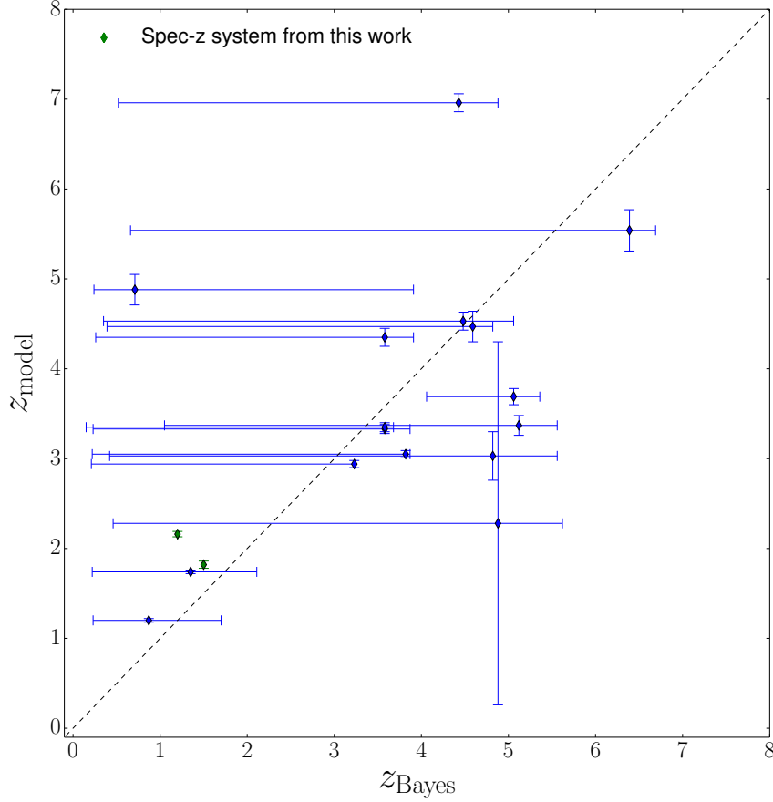
Figure 2.14 Comparison of the redshifts determined in this work ( z_{\text{Bayes}} ) versus the model-predicted redshifts given by Jauzac et al. (2014) for all multiple image systems used in the lens model. Note that the previously confirmed spectroscopic systems are left out of this comparison because z_{\text{model}} were not calculated. Two systems (green) are spectroscopically confirmed in this work for the first time and are included in the comparison. For these two objects, we use the new spectroscopic redshift on the horizontal axis in place of z_{\text{Bayes}} . The z_{\text{model}} values are in significant disagreement with the spectroscopic values for these two systems. z_{\text{Bayes}} represents the peak of a statistical combination of all available photometric redshift probability density functions (Dahlen et al., 2013). The vertical error bars reflect 1\text{-}\sigma Gaussian error on z_{\text{model}} , and the horizontal error bars show the 68% credible interval for z_{\text{Bayes}} . 12/16 systems are consistent at 68% confidence level.
