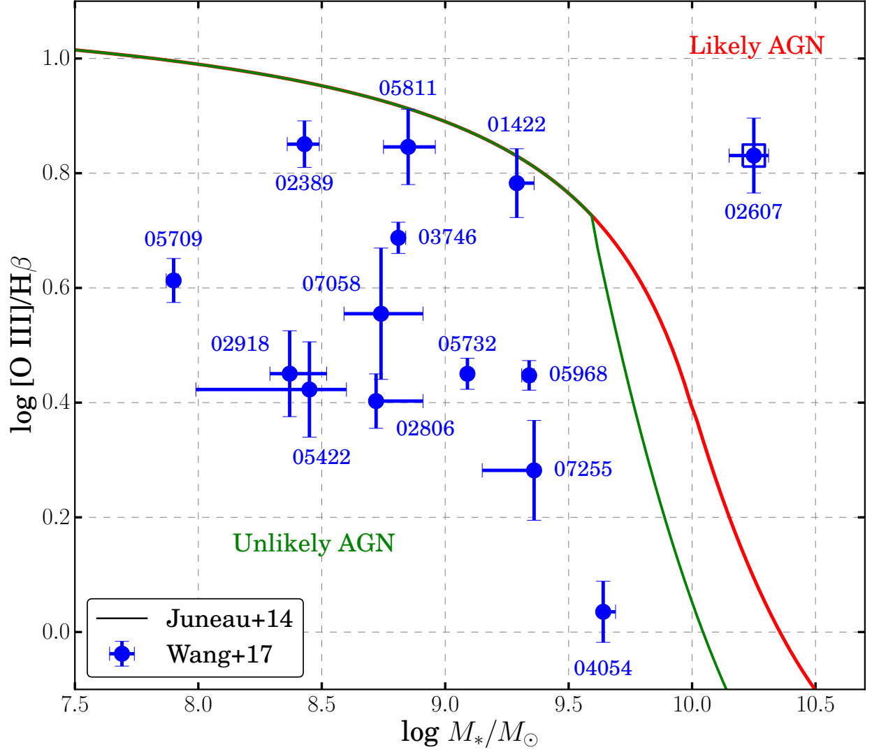
Figure 3.6 Mass excitation diagnostic diagram for our metallicity gradient sample. The curves are the demarcation lines updated by Juneau et al. (2014). The regions below the green curve have a low probability ( < 10\% ) of being classified as AGNs, whereas galaxies located above the red curve are secure AGN candidates. In our sample, the only AGN candidate, i.e., ID 02607, is marked by a square.
