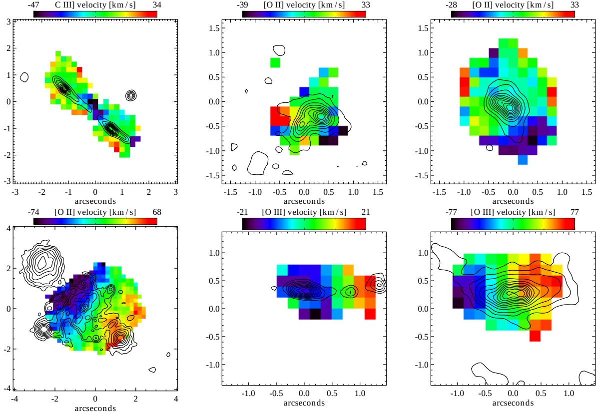
Figure 3.14 Velocity fields derived from integral field spectra. Top row : IDs 02389, 02806, 03746 (left to right) observed with MUSE . Bottom row : ID 04054 observed with MUSE (see also Figure 8 in Grillo et al. (2016)) and IDs 05709, 05968 (left to right) observed with KMOS . In all cases, the color scale shows EL velocity centroids in each spaxel, with contours showing HST / ACS I_{814} band continuum. The kinematics map for galaxy 05709 (shown in the lower middle panel) is the first one to date presented for star-forming galaxies with M_* \lesssim 10^8 M_\odot at z \gtrsim 1 .
