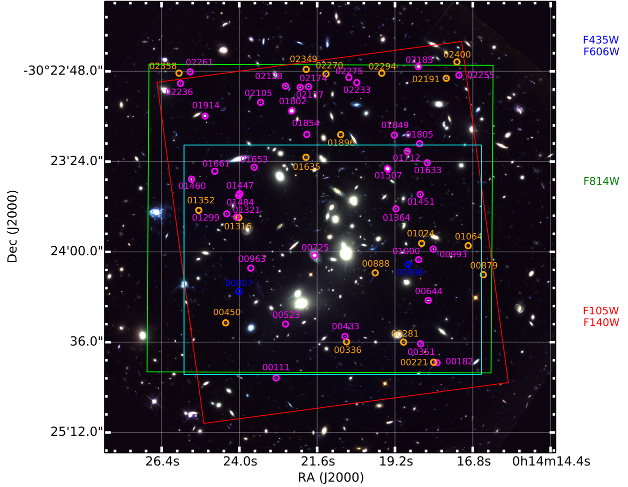
Figure 2.1 The color composite image of Abell 2744 based on the HFF and GLASS imaging. The blue, green and red channels are composed by the filters on the right. The two distinct P.A.s of the spectroscopic GLASS pointings are shown by the red (P.A.=233 degrees) and green (P.A.=135 degrees) squares. Figure 2.2 shows the grism images corresponding to these two P.A.s. The locations of the emission line objects from Table 2.2 are marked by circles, with color coding reflecting the GLASS spectroscopic redshift quality (cf. Section 2.4.2 and column “Quality” in Table 2.2; 2=blue, 3=orange, and 4=magenta). The cyan square shows the outline of Figure 2.3.
