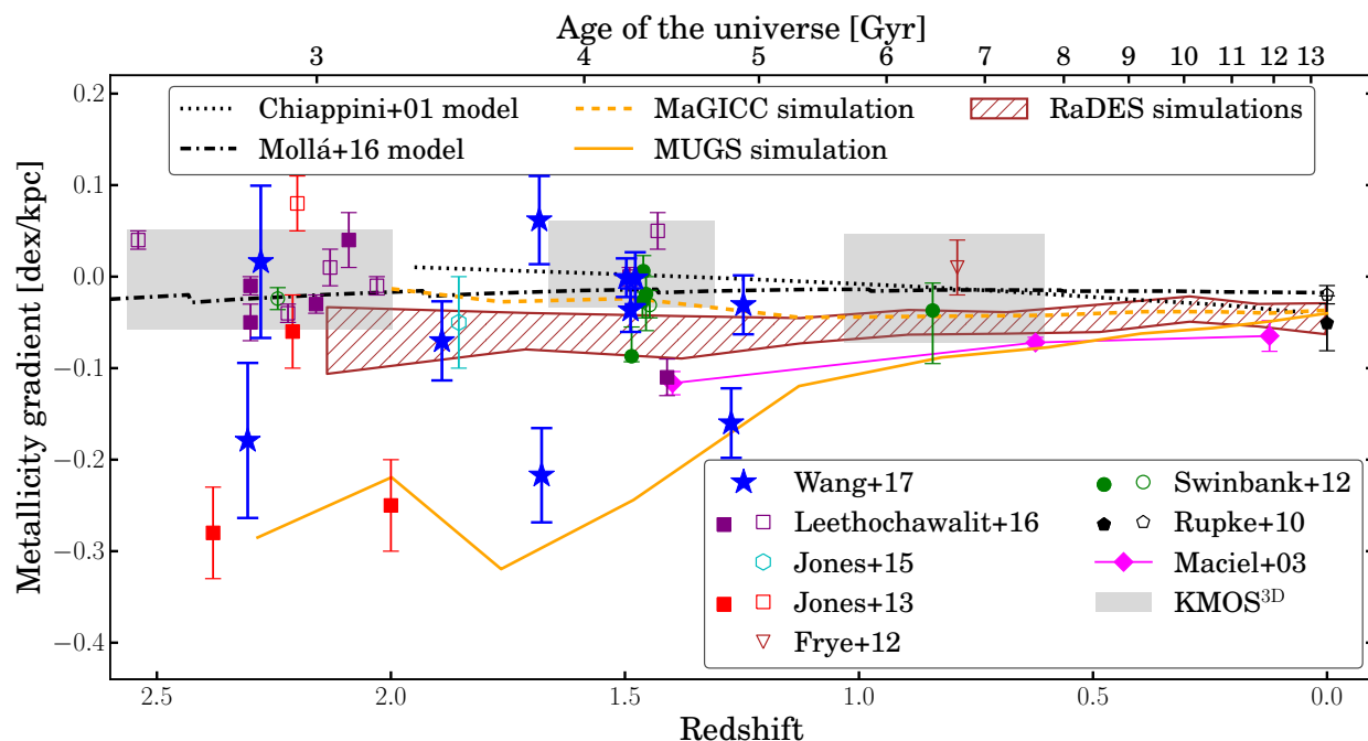
Figure 3.12 Evolution of metallicity gradients with redshift. The blue stars represent the metallicity gradients measured in this work, and the cyan hexagon is from our previous work (Jones et al., 2015b). We include all the high- z metallicity gradient measurements with sub-kpc resolution in the current literature: lensed galaxies analyzed by Frye et al. (2012), Jones et al. (2013), and Leethochawalit et al. (2016), non-lensed galaxies observed with AO (Swinbank et al., 2012). The spread of the KMOS^{3D} measurements obtained with seeing-limited conditions (Wuyts et al., 2016) is marked as grey shaded regions. We also show the averages of local metallicity gradients (Rupke et al., 2010), and the trend of the Milky Way gradient evolution based upon planetary nebula estimates (Maciel et al., 2003). Except for the blue stars, hollow and filled symbols correspond to interacting/merging and isolated systems, respectively. In addition, the predictions from different analytical chemical evolution models and numerical simulations are also shown as comparisons to the observational results (see Section 3.6.1 for more details).
