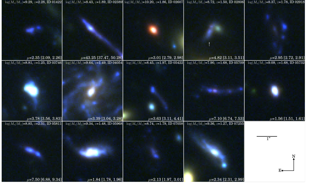
Figure 3.2 Zoom-in color composite stamps of our metallicity gradient sample, cut out from the full FoV image shown in Figure 3.1. In each stamp, we also show the spectroscopic redshift, stellar mass and lensing magnification (best-fit value followed by 1-\sigma confidence interval) of the galaxy. In the panel of ID 02806, we use the white arrow to point to our galaxy of interest (ID 02806). All stamps are on the same spatial scale. The 1'' scale bar and north-east compass are shown in the lower right corner.
