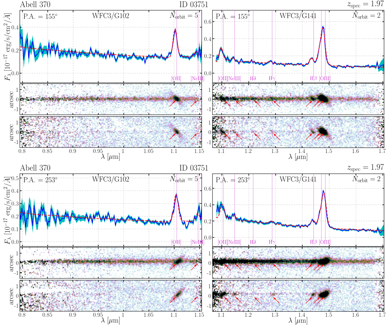
Figure 4.9 The HST grism spectra for source ID 03751 in the field of Abell 370 taken by the GLASS program. The total science integration is equally distributed into two separate P.A.s, reaching 5 orbits of G102 exposures and 2 orbits of G141 exposures per P.A., shown in two sub-figures. In each sub-figure, from top to bottom, we show the optimally extracted 1D spectra and the full 2D spectra before and after source continuum subtraction, for both grism elements. On the 1D spectra, the observed flux is represented by the blue solid line with 1\text{-}\sigma noise level denoted by the cyan shaded band, and the 1D model spectrum (source continuum + nebular emission) is represented by the red dashed curve. The observed locations of emission features are highlighted by vertical dotted lines in magenta and arrows in red, in 1D and 2D spectra respectively.
