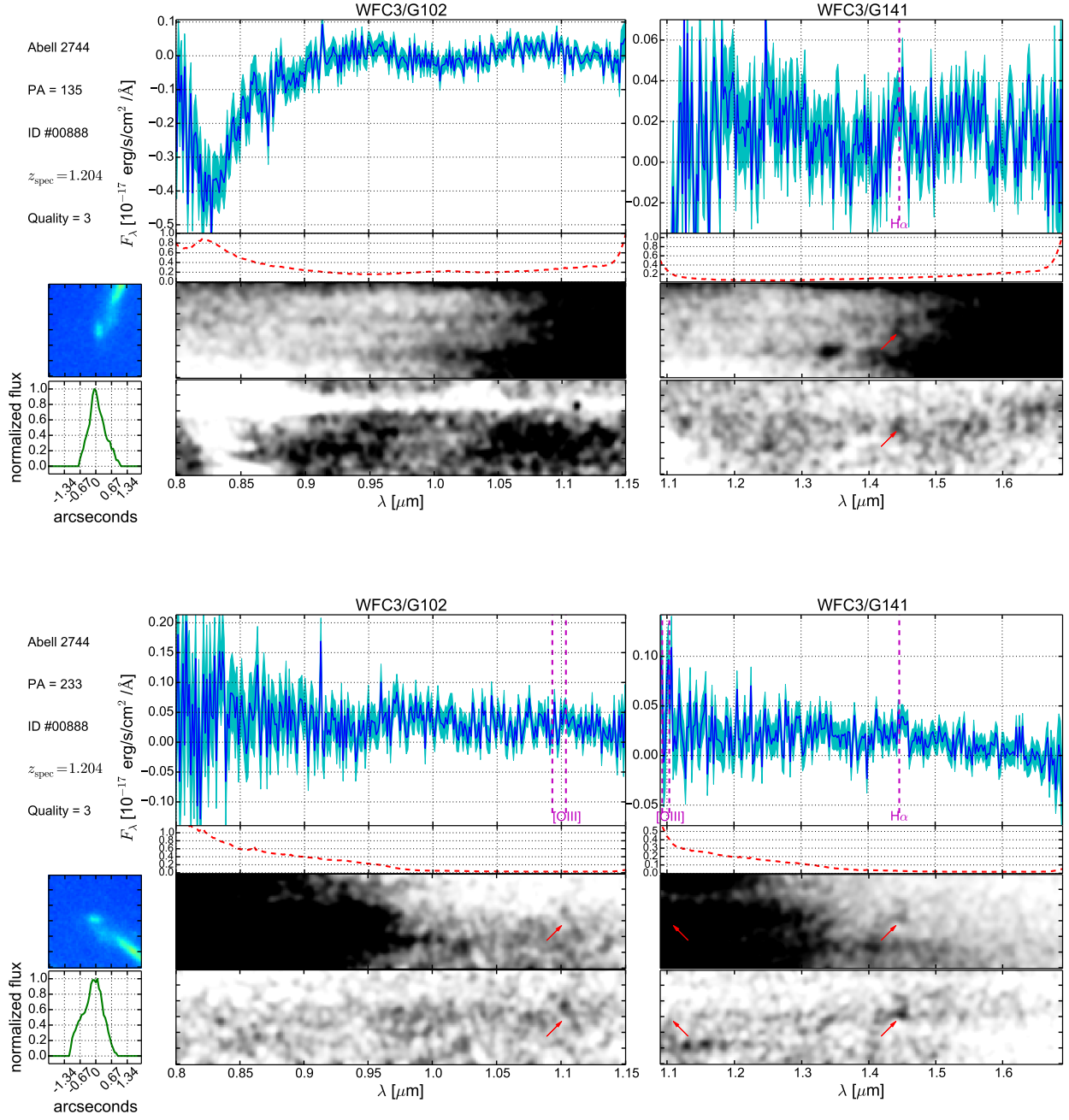
Figure 2.9 Same as Figure 2.8, except that object ID 00888 (arc 56.1) is shown.
