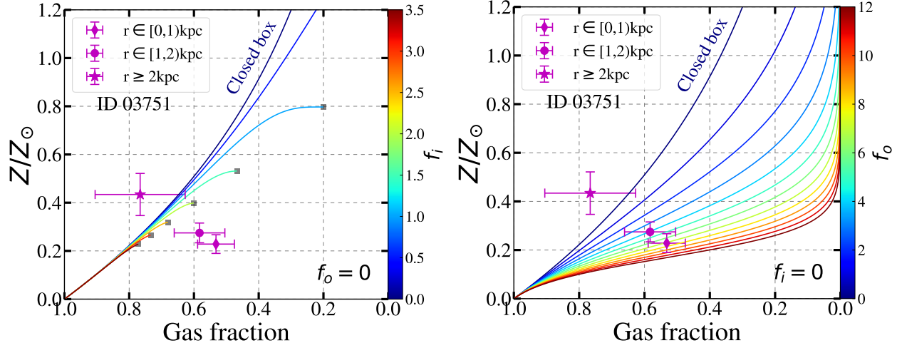
Figure 4.5 Gas fraction and metallicity estimated in different radial annuli for galaxy ID 03751. The diamond, circle, and star symbols represent measurements derived at a galacto-centric radius of r \in [0, 1) kpc, r \in [1, 2) kpc, and r \geq 2 kpc, respectively. We also overlay the curves calculated from a simple chemical evolution model Erb (2008) under extreme conditions, i.e., pure gas inflow ( f_o = 0 ; left) and pure gas outflow ( f_i = 0 ; right). Note that the trajectories of pure gas inflow cases cease at the grey squares for high infall rate ( f_i \gtrsim 1 ) conditions; any extensions from those grey squares toward low gas fraction (while fixing metallicity) are unphysical. This simple comparison shows that purely gas accretion does not suffice to explain the strong inverted gradients seen in our galaxies.
