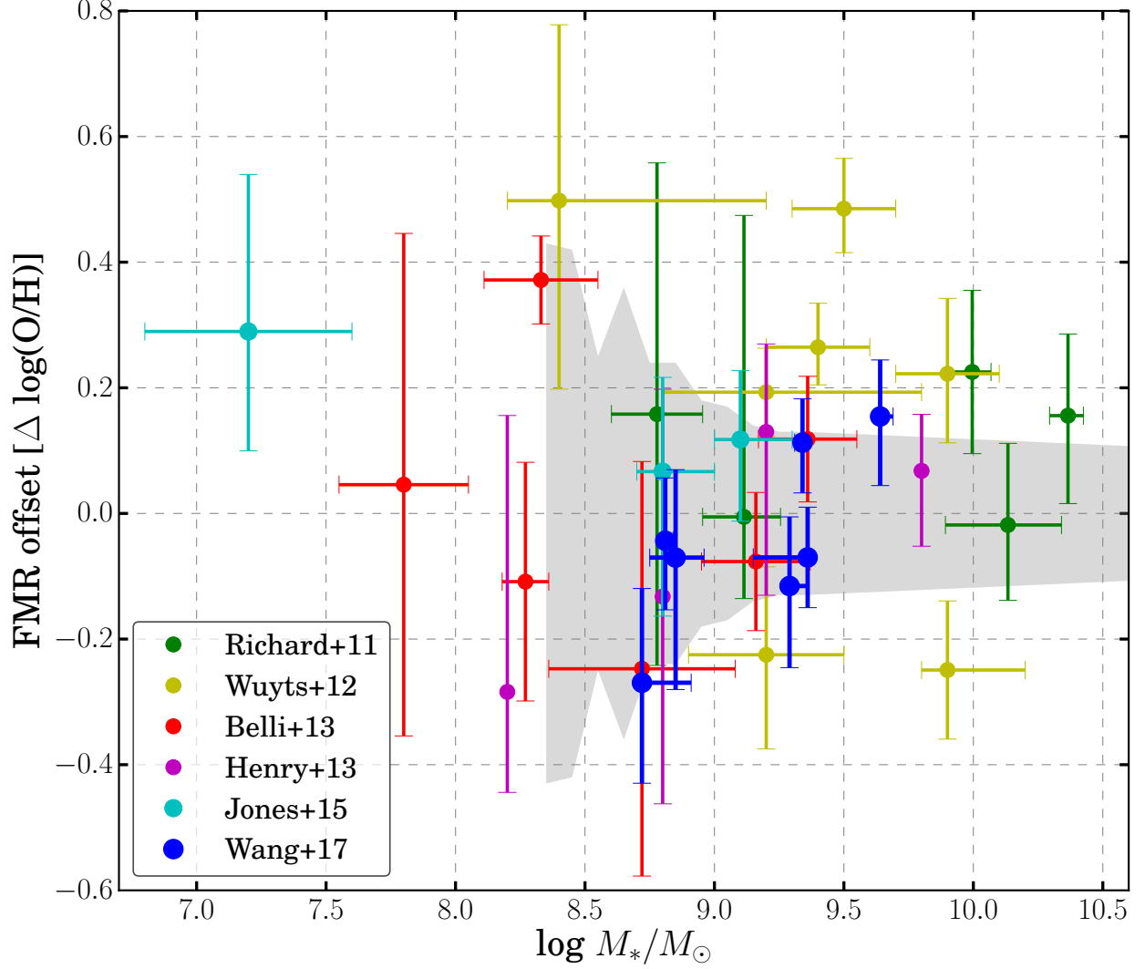
Figure 3.9 The offset from the fundamental metallicity relation first proposed by Mannucci et al. (2010) for the z \sim 1.8 metallicity measurements derived assuming the Maiolino et al. (2008) calibrations. The color-coding for the points is the same as in Figure 3.7. The shaded region shows the intrinsic scatter of the FMR extended to low-mass regime given by Mannucci et al. (2011).
