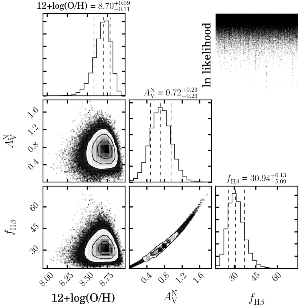
Figure 3.5 The marginalized 1D and 2D constraints on (12 + \log(\text{O}/\text{H}), A_V^N, \text{ and } f_{\text{H}\beta}) , which are drawn from the integrated line fluxes of the Refsdal host galaxy (ID 04054), after all grism exposures are combined. The values on top of each column are the medians with 1-\sigma uncertainties for each parameter. The plot in the upper right corner illustrates a good convergence of the sampling.
