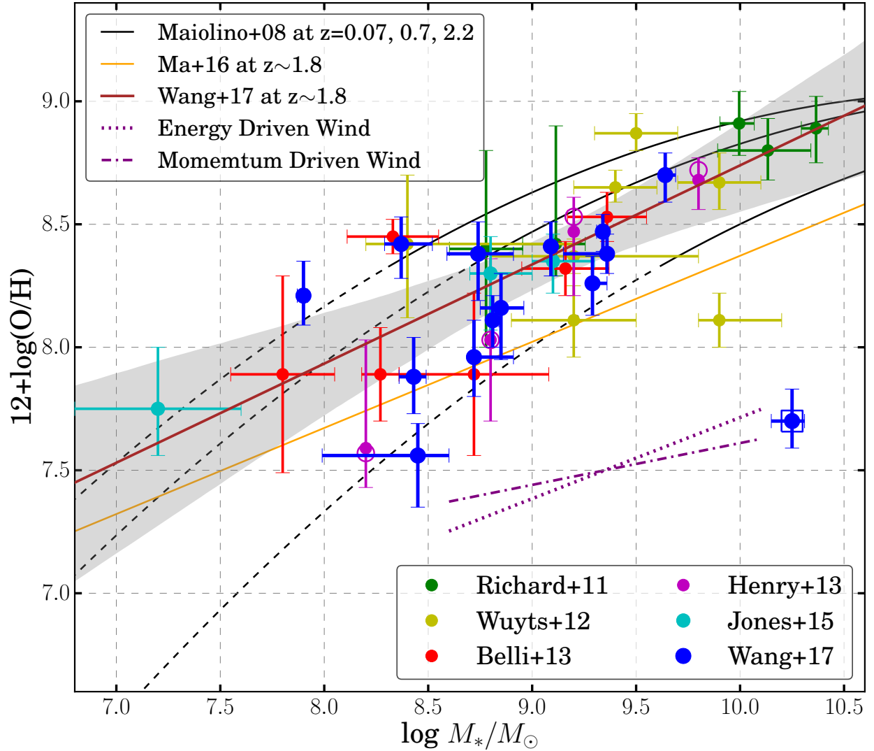
Figure 3.8 The relation between stellar mass and gas-phase oxygen abundance, from observations and simulations at z \sim 1.8 . The color-coding for all the points is the same as in Figure 3.7. For the sake of consistency, all metallicity measurements are derived assuming the Maiolino et al. (2008) strong EL calibrations. The black curves represent the 2nd order polynomials fitted by Maiolino et al. (2008) to data sets at different redshifts, where dashed parts correspond to extensions beyond mass completeness limits of those data sets. The thick brown line denotes our best-fit linear relation based upon all data points except the AGN candidate (i.e. ID 02607) marked by a square. The shaded band marks the 1\text{-}\sigma confidence region. For the Henry et al. (2013b) stack data points, we also show the measurements without dust correction as open circles, which are not included in the fit. The thin orange line is the prediction from the cosmological zoom-in simulations conducted by Ma et al. (2016) at the same redshift range. The purple dotted and dash-dot lines illustrate the slopes given by the energy and momentum driven models, respectively.
