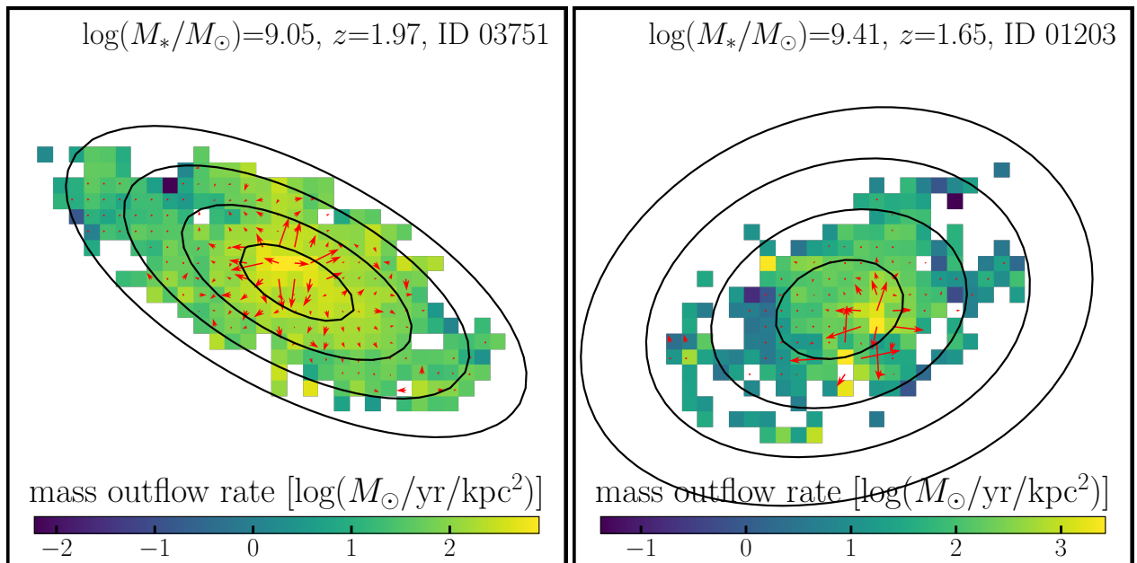
Figure 4.6 Maps of gaseous outflow rates derived from our analysis combining gas regulator models and empirical star-formation laws. The spatial extent and orientation follows that in Figure 4.1. Red arrows show the net direction and magnitude of the gaseous outflows driven by galactic winds. We argue that outflows play a key role in effectively transporting stellar nucleosynthesis yields from the inner regions of these two galaxies to their outskirts.
