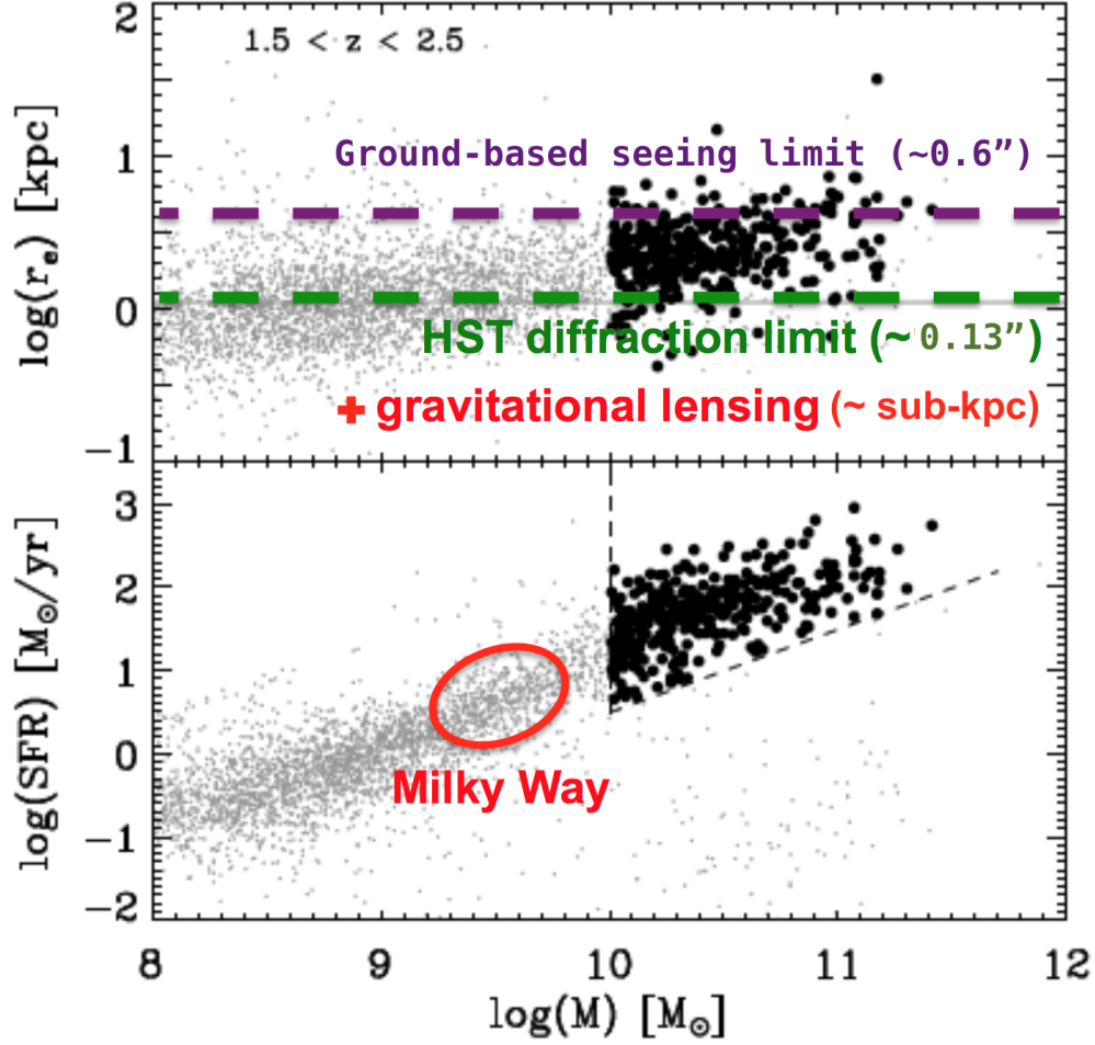
Figure 1.3 The relationship among the effective radius, star-formation rate and stellar mass for galaxies at z \sim 2 covered by the CANDELS survey. The region where MW progenitors reside according to abundance matching is denoted by a red circle. The spatial resolution from natural seeing, native HST, and with gravitational lensing magnification combined are marked by the horizontal lines. We see that the only feasible approach to unambiguously resolve the MW progenitors is through the synergy of HST diffraction limit and lensing magnification. Figure credit: Wuyts et al. (2012b).
