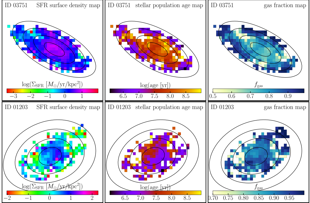
Figure 4.4 Maps of SFR surface density, average stellar population age, and gas fraction for our galaxies, derived from our spatially resolved analysis of stellar continuum and nebular emission. The spatial extent and orientation follows that in Figure 4.1. We see that for both sources compared with their outskirts, their central regions have more active star formation, older stellar population, and lower gas fraction.
