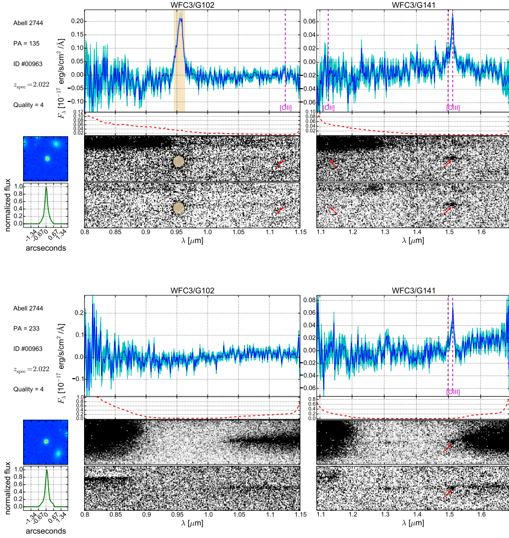
Figure 2.5 Emission line detection results on object ID 00963 (arc 6.1) at the two P.A.s displayed in the two sub-figures accordingly. In each sub-figure, the two panels on the first row show the observed 1D spectra, where the contamination subtracted flux is denoted by the blue solid line and the noise level by the cyan shaded region. The two panels on the second row give the corresponding contamination model in red dashed line. For the four panels directly underneath, the top two display the interlaced 2D spectra whereas the bottom two have contamination subtracted. In the 1- and 2D spectra, the identified emission lines are denoted by vertical dashed lines in magenta and arrows in red, respectively. The wheat colored regions cover contamination model defects. The two panels on the far left refer to the 2D postage stamp created from the HFF co-adds through drizzling (on top) and the 1D collapsed image (on bottom).
