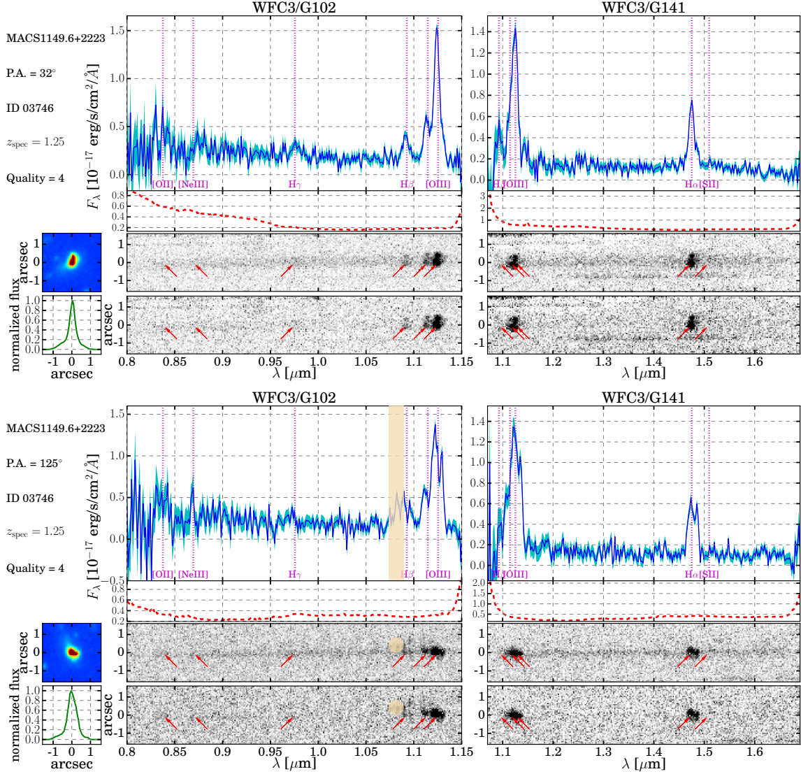
Figure 3.15 The HST grism spectra for one exemplary source in our sample, ID 03746, seen at the two GLASS PAs displayed in the two sub-figures respectively. In each sub-figure, the two small square panels on the left refer to the 2D postage stamp (top) and the 1D collapsed image (bottom). The 2D postage stamp is created from the HFF H_{160} -band co-adds. The eight panels in the middle and right rows show, from top to bottom, the contamination subtracted 1D spectra (where flux is represented by the blue solid line and the noise level by the cyan shaded band), the 1D contamination model in red dashed line, the contamination subtracted 2D spectra and the 2D spectra having source continuum further removed. In the 1D and 2D spectra, the locations of emission lines are highlighted by vertical dotted lines in magenta and arrows in red, respectively, and the wheat colored patches cover contamination model defects.
