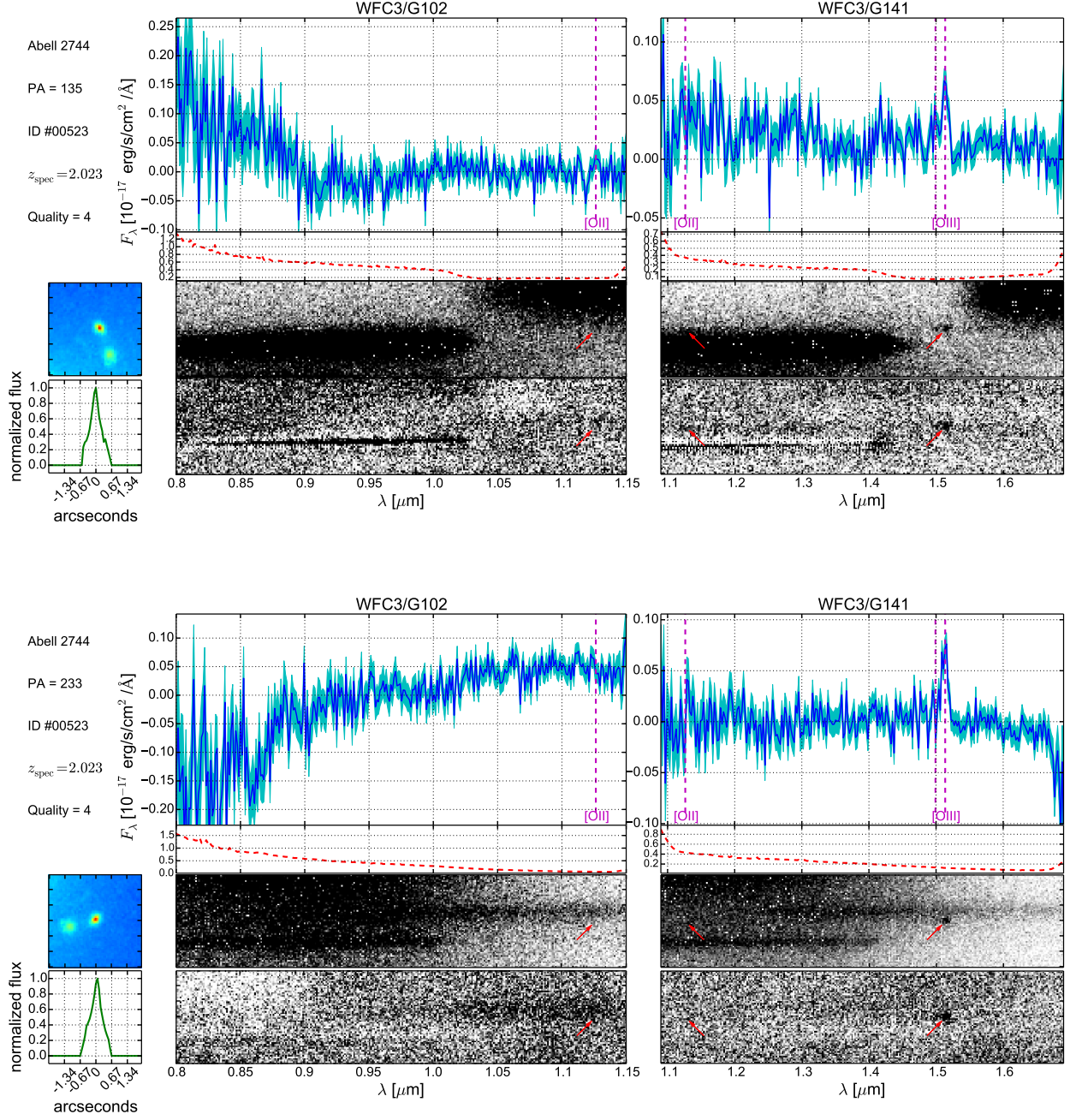
Figure 2.6 Same as Figure 2.5, except that object ID 00523 (arc 6.2) is shown.
