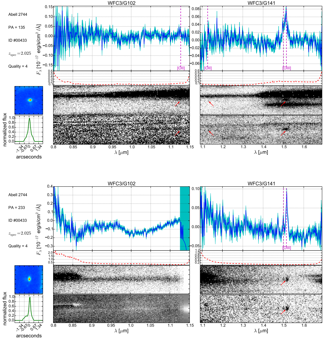
Figure 2.7 Same as Figure 2.5, except that object ID 00433 (arc 6.3) is shown. Note here WFC3/G102 at the second P.A. is cut off on the right due to grism defect.
