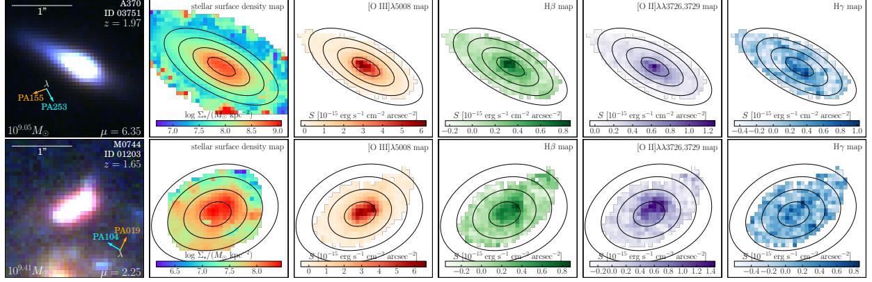
Figure 4.1 Two star-forming dwarf galaxies at z \sim 2 displaying unusually strong inverted metallicity gradients, securely determined at sub-kpc spatial resolution. For each source we show, from left to right: color composite image (created from HST broad-band photometry), stellar surface density map (obtained from SED fitting to HST photometry), and surface brightness map of ELs [O III], H\beta , [O II], and H\gamma . The black contours overlaid represent the source plane de-projected galactocentric radii with 1 kpc interval. The two light-dispersion directions for the grism exposures are denoted by the orange and cyan arrows (see Figures 4.9 and 4.10 for the corresponding spectra). The spatial extent and orientation are unchanged for the two sources in all 2D stamps throughout. North is up and east is to the left.
