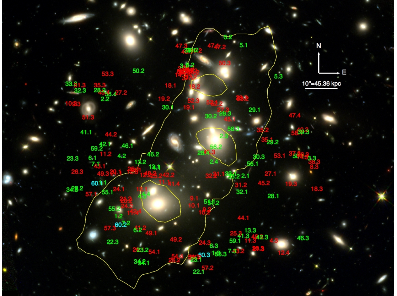
Figure 2.3 All multiple images discovered to date in Abell 2744. Green images are used in the lens model, while red images are unused for reasons discussed in Section 2.4. Cyan images belong to a new multiple image system discovered in this work. The yellow line is the critical curve from our best-fit lens model at z = 9 . The RGB image is a combination of F105W, F125W and F160W.
