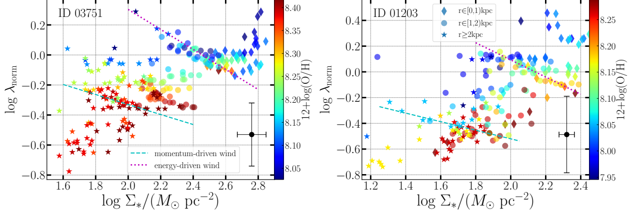
Figure 4.7 Correlation between spatially resolved mass loading factor \lambda (normalized to the value at radius 1 kpc; see Table 4.1) and stellar surface density \Sigma_* , color-coded by metallicity. As in Figure 4.4, the diamond, circle, and star symbols represent measurements derived at a galactocentric radius of r \in [0, 1)\text{kpc} , r \in [1, 2)\text{kpc} , and r \gtrsim 2\text{kpc} , respectively. We overlay as an illustration two scaling relations that are commonly assumed to describe integrated measurements: \lambda \propto \Sigma_*^{-2/3} for an energy-driven wind model marked by magenta dotted lines, and \lambda \propto \Sigma_*^{-1/3} for a momentum-driven wind model by cyan dashed lines. Evidently, a single scaling relation is not sufficient to describe the spatially resolved data, demonstrating the need for a more sophisticated approach. The black point in the lower right corner in each panel displays the median uncertainties for these measurements.
