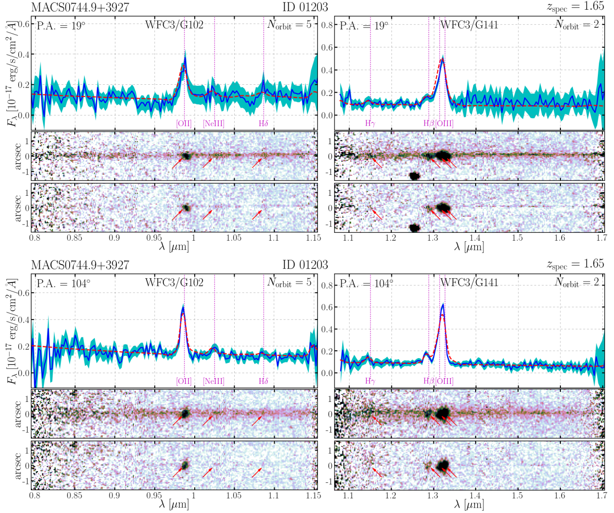
Figure 4.10 Same as Figure 4.9, except that source ID 01203 in the field of MACS0744.9+3927 is shown.
