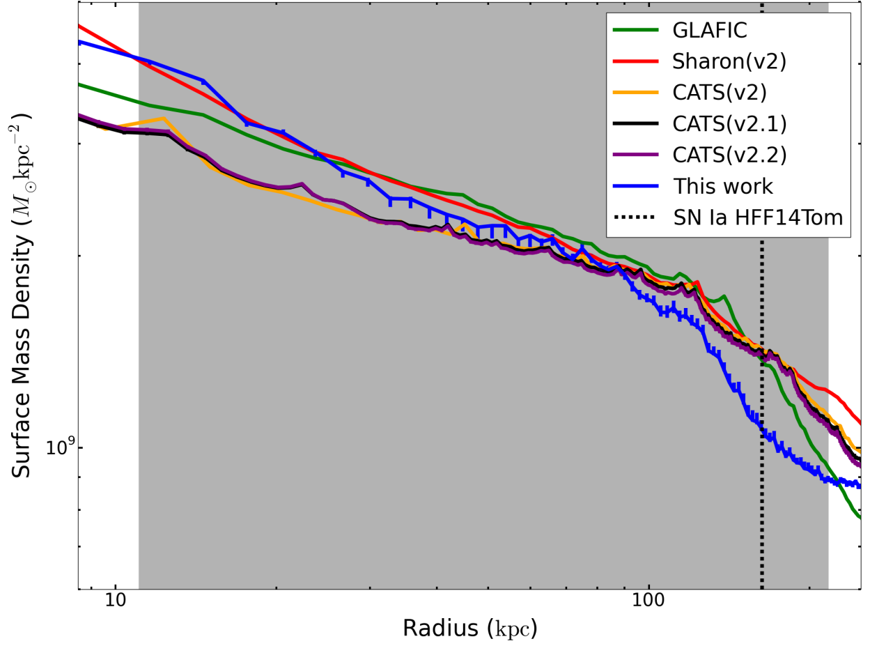
Figure 2.12 Surface mass density profile for the lens model obtained in this work compared to several recently published lens models of Abell 2744. The Sharon v2 model is presented by Johnson et al. (2014), the GLAFIC model by Ishigaki et al. (2015), the CATS(v2) model in Jauzac et al. (2014), and the CATS(v2.1) and CATS(v2.2) models by Jauzac et al. (2015, private communication). The shaded gray region indicates the radii over which multiple image constraints are available. The models agree best within this region, and they begin to significantly disagree at radii \gtrsim 200 kpc. The radius is measured from the center of the BCG. Error bars shown for our model represent 68% confidence. Gaussian 1\text{-}\sigma error bars are included on all three CATS models, but are almost entirely too small to discern.
