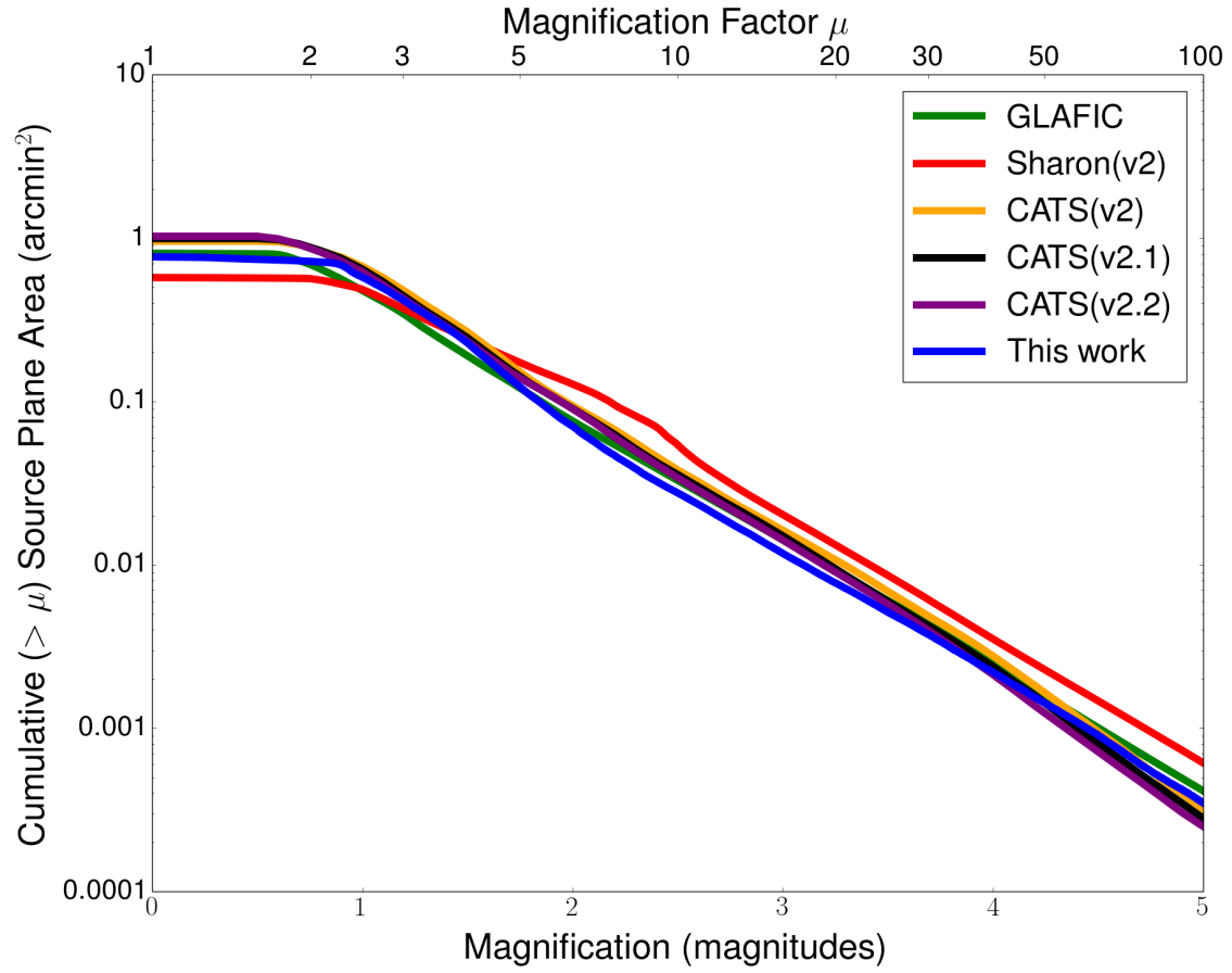
Figure 2.13 Cumulative source plane area versus magnification at z = 9 . The models used in this comparison are the same as those described in Figure 2.12.
