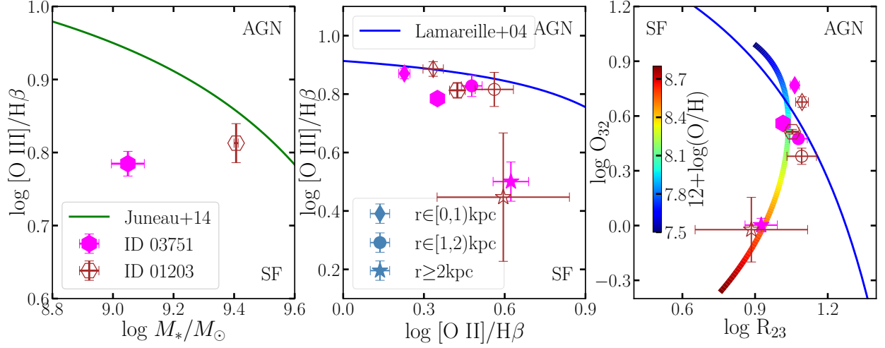
Figure 4.2 The diagnostic diagrams for our sources. On the left, we show the mass-excitation diagram with the demarcation scheme between the loci of AGNs and star-forming (SF) galaxies proposed in Juneau et al. (2014). Our galaxies can be safely classified as the latter. In the middle and right panels, we show the “blue” diagrams with the boundaries described by Lamareille et al. (2004). Following the conventions in the left panel, we use filled symbols to represent measurements for ID03751 whilst empty ones for ID01203. Furthermore, the hexagons correspond to the measurements integrated over the entire galaxies (as in the left panel), whereas the other symbols denote results obtained in different radial annuli, as explained in the legend of the middle panel. Again we see that the contamination from AGN ionization is minimum for our sources, even in the central regions. In the right panel, we also show the gas-phase metallicities given by the Maiolino et al. (2008) calibrations involving R_{23} and \text{O}_{32} . The two galaxies presented in this work share similar evolutionary trends in their excitation and ionization states with respect to galacto-centric radius, strongly indicating that their metallicity increases with galacto-centric radius. All the line flux ratios are corrected for dust extinction following the Cardelli et al. (1989) law with nebular attenuation estimated from the observed Balmer decrement of f_{\text{H}\gamma}/f_{\text{H}\beta} under the assumption of Case B recombination conditions.
