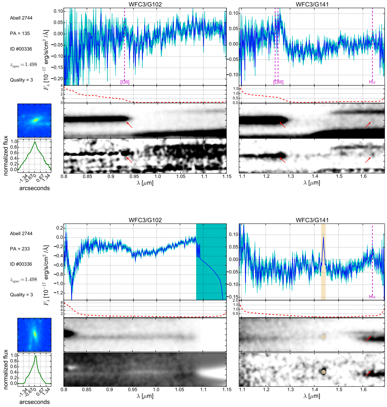
Figure 2.8 Same as Figure 2.5, except that object ID 00336 (arc 1.3) is shown. Moreover, the 2-dimensional spectra are smoothed, whilst the 1-dimensional spectral resolution remains unchanged.
