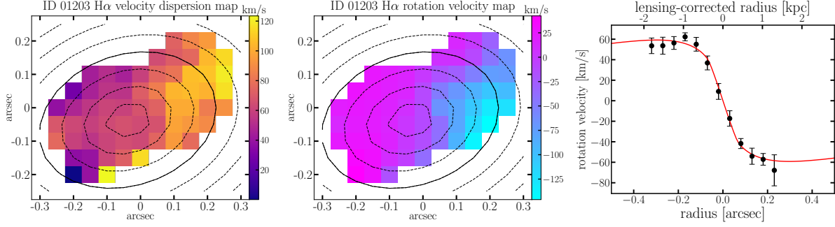
Figure 4.8 H\alpha emission kinematics of ID 01203 from our OSIRIS AO-assisted observations showing the velocity dispersion ( left ), the rotation velocity ( center ), and rotation curve extracted along the major axis ( right ). The overlaid contours in the left and center panels also represent the source plane de-projected galacto-centric radii, but in 0.25 kpc interval. To give relative scale with respect to our HST stamps, the 1 kpc radius contour is still in solid. The red curve in the right panel is the best-fit rotation curve for an exponential disk mass distribution, giving a maximum line-of-sight velocity V \sin i = 94 \pm 7 \text{ km s}^{-1} . The data are in good agreement with a thick disk rotation curve despite a high level of turbulence.
