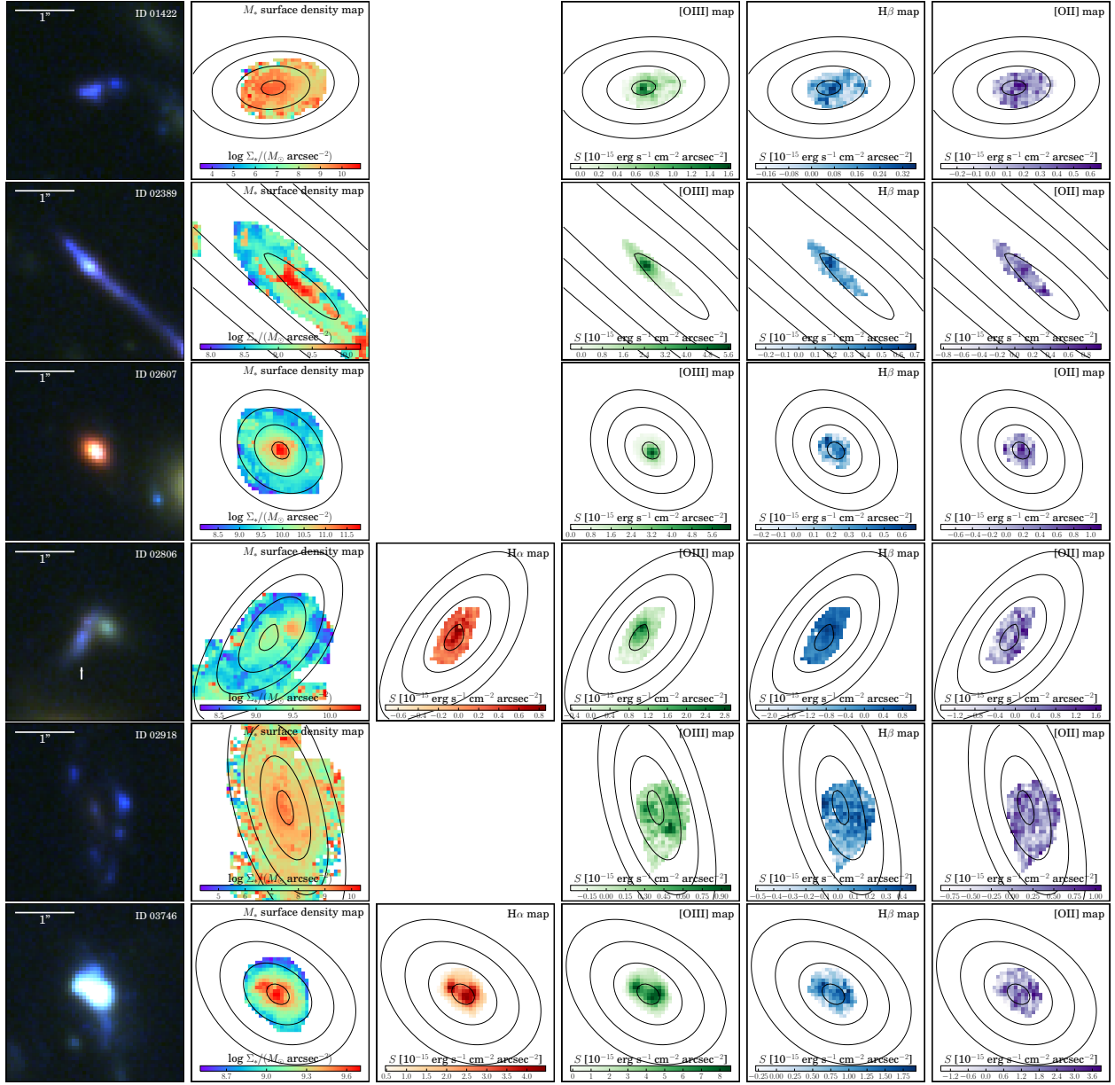
Figure 3.4 Multi-perspective view of our metallicity gradient sample except for the SN Refsdal host which is shown in Figure 3.3. In each row, we show the zoom-in color composite stamp (the same as that in Figure 3.2), the stellar mass surface density map, the combined surface brightness maps of H\alpha (if available given object redshift), [O\ III] , H\beta , [O\ II] for each object. The black contours overlaid represent the source plane de-projected galactocentric radii in 2 kpc interval, starting from 1 kpc. The spatial extent and orientation of the stamps for each object have been fixed. The typical surface brightness 1-\sigma uncertainty in these combined EL maps is 2 \times 10^{-16} \text{ erg s}^{-1} \text{ cm}^{-2} \text{ arcsec}^{-2} .
