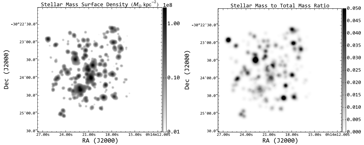
Figure 2.15 Stellar mass surface density (left) and stellar to total mass ratio (right) distributions of Abell 2744. Stellar mass surface density is in the unit of M_{\odot} \text{ kpc}^{-2} .
