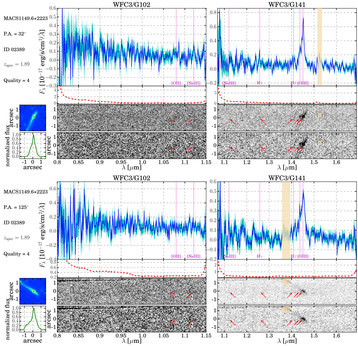
Figure 3.16 Same as Figure 3.15, except that source ID 02389 is shown. The H \alpha EL of this galaxy has shifted out of the grism coverage because of its redshift z = 1.89 .
