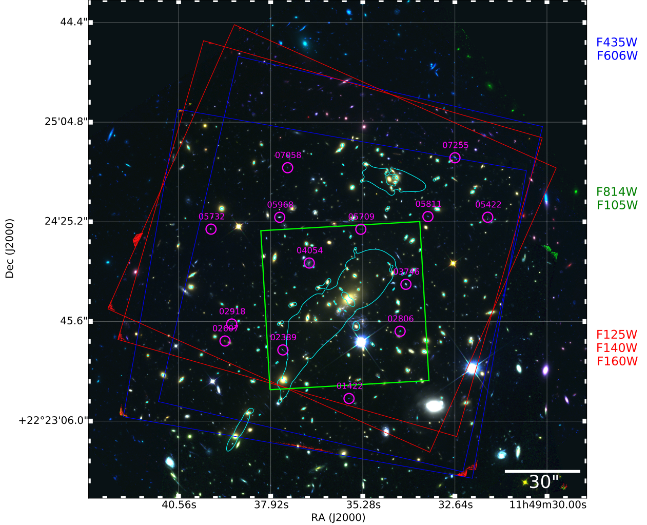
Figure 3.1 Color composite image of MACS1149.6+2223 from the full-depth 7-filter HFF photometry. The blue, green, and red channels are comprised of the HST broad-band filters shown on the right. The blue, red and green squares mark the footprints of GLASS , the Refsdal follow-up, and MUSE programs utilized in this work. The cyan contours are the critical curves at z = 1.8 predicted by the GLAFIC version 3 lens model. The critical curves denote the regions where lensing magnification reaches infinity. Thus the closer proximity between the object and the critical curve at the object’s redshift indicates higher magnification that the object has. The magenta circles show the positions of our metallicity gradient sample. 3 \times 3 arcsec 2 zoom-in postage stamps around these positions are shown in Figure 3.2.
