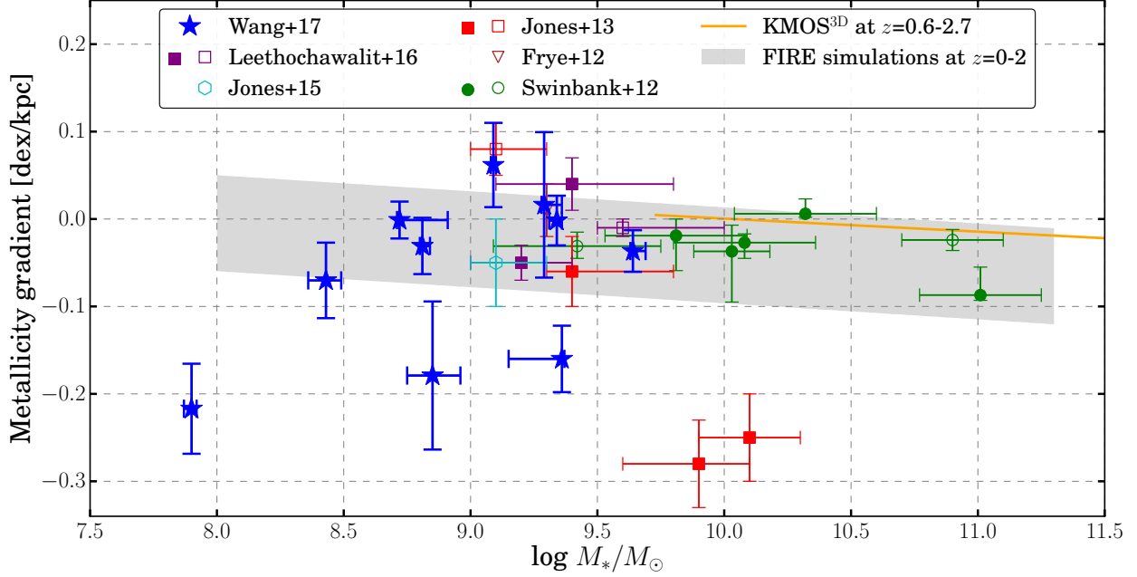
Figure 3.13 Observed metallicity gradients as a function of M_* . The color-coding of symbols is the same as in Figure 3.12. Except for the blue stars, hollow and filled symbols correspond to interacting/merging and isolated systems, respectively. Most of the Leethochawalit et al. (2016) gradient measurements do not have reliable M_* estimates due to the lack of near IR photometry. The orange line shows a simple linear fit to the metallicity gradient results at z=0.6-2.7 from the KMOS^{3D} observations, only covering the stellar mass range of \log(M_*/M_\odot) \in [9.7, 11.5] (Wuyts et al., 2016). The 2\text{-}\sigma interval of the FIRE simulation results presented by Ma et al. (2016) is shown as the shaded region. The only work to date that presents metallicity gradient measurements in the M_* \lesssim 10^9 M_\odot regime is this work, which even extends to below 10^8 M_\odot .
