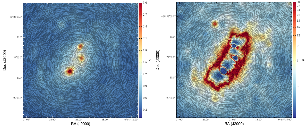
Figure 2.11 Convergence (left), \kappa and flux magnification (right), \mu , maps of Abell 2744 produced by our lens model for a source at z = 9 . Maps cover 3.5 \times 3.5 \text{ arcmin}^2 . In both maps, the gray stick pattern indicates the phase angle of the shear.
