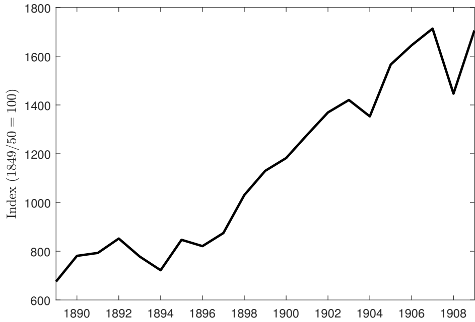
Figure 2.26: Index of industrial production for United States, 1889-1909.
