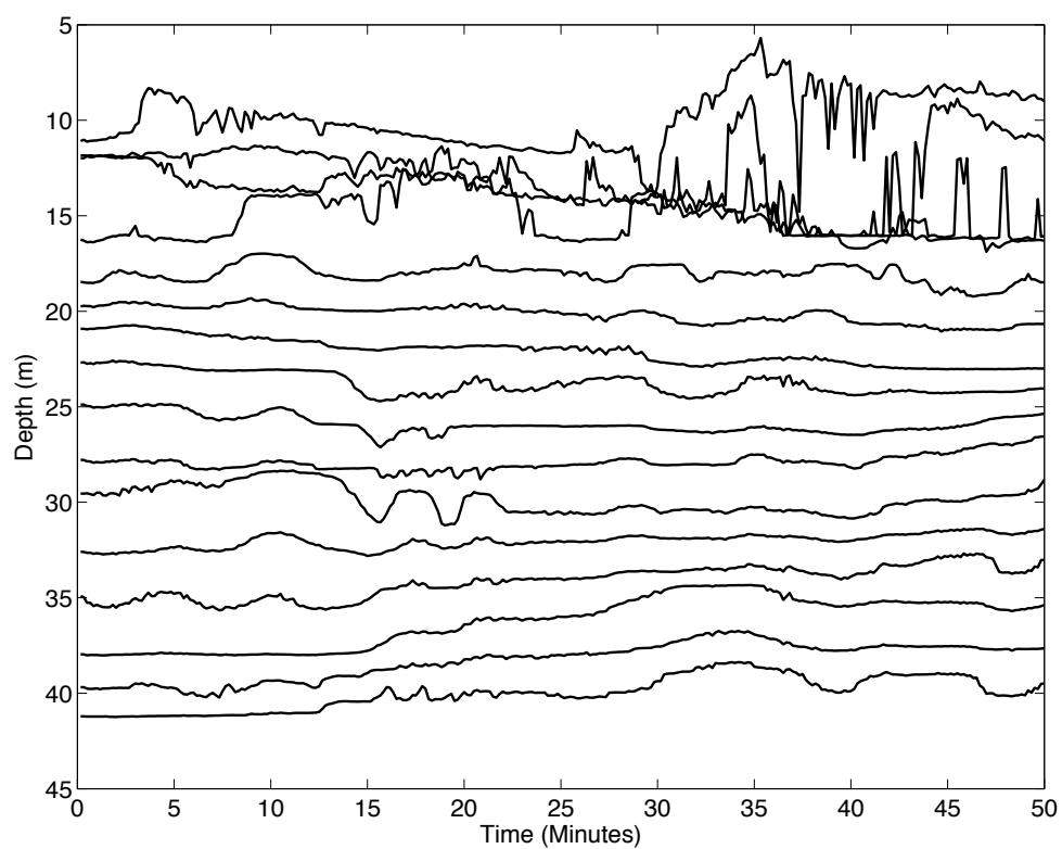
Figure 4.23: Displacement estimates computed using the median of temperature observations for the FAF06 experiment.
