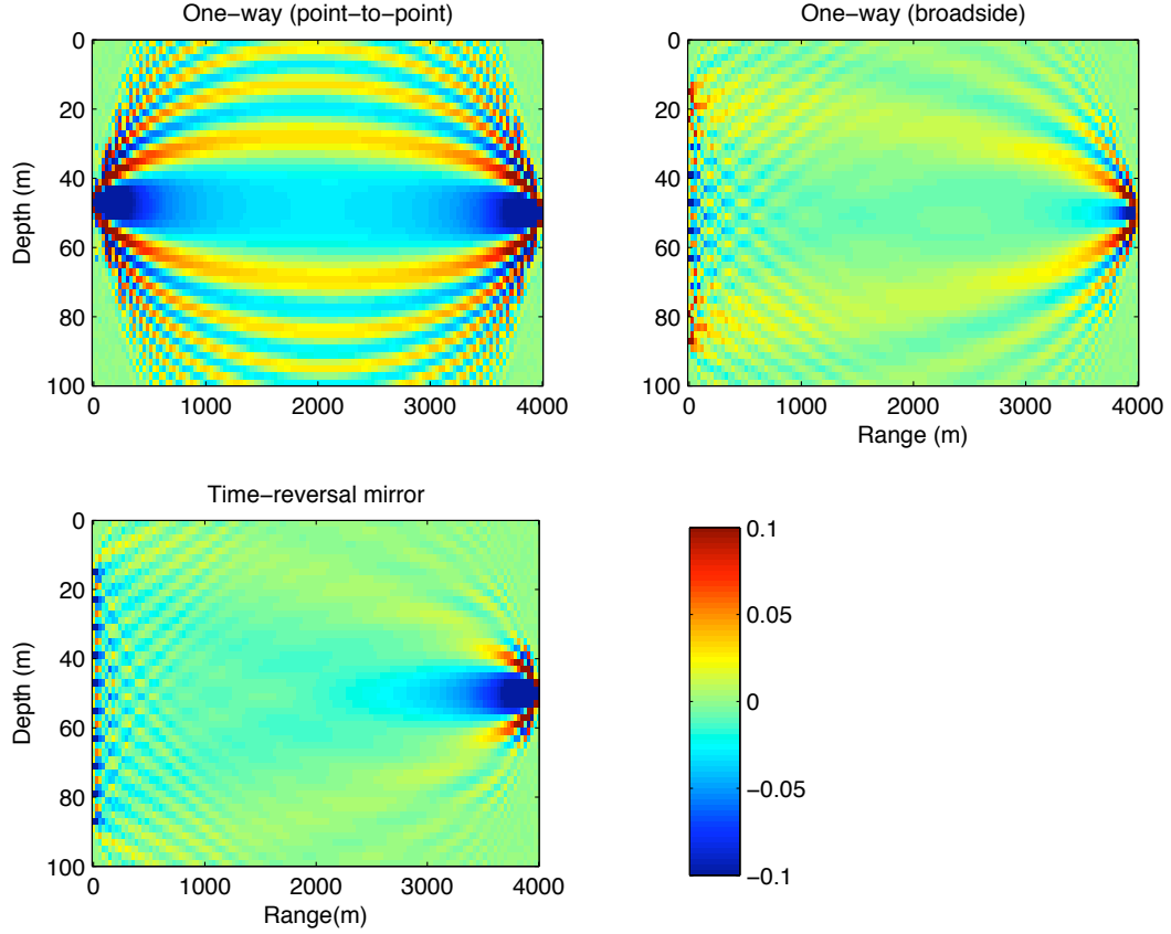
Figure 2.2: Time domain sensitivity kernels ( 10^{-5} \mu Pa \ s \ m^{-4} ) evaluated at the peak of the arrival for: Top Left Point-point one-way, Top Right Array-to-point one-way (broadside) , Bottom Left Array-to-point time-reversal (time-reversal mirror). Receiver is on the right hand side of each plot, at a depth of 50 m.
