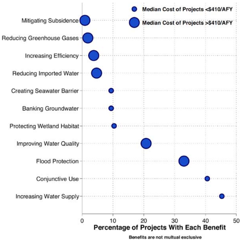
Figure 19 Analysis of managed aquifer recharge (MAR) project benefits with cost information. The size of the dot indicates whether the median costs for projects within each benefit category is below or above the median cost of all the projects (i.e., $0.33 per m 3 /year [$410/acre-feet/year]) from Fig. 3 from the study by Perrone D, Merri Rohde M. Benefits and economic costs of managed aquifer recharge in California . San Franc Estuary Watershed Sci 2016; 14(2).
