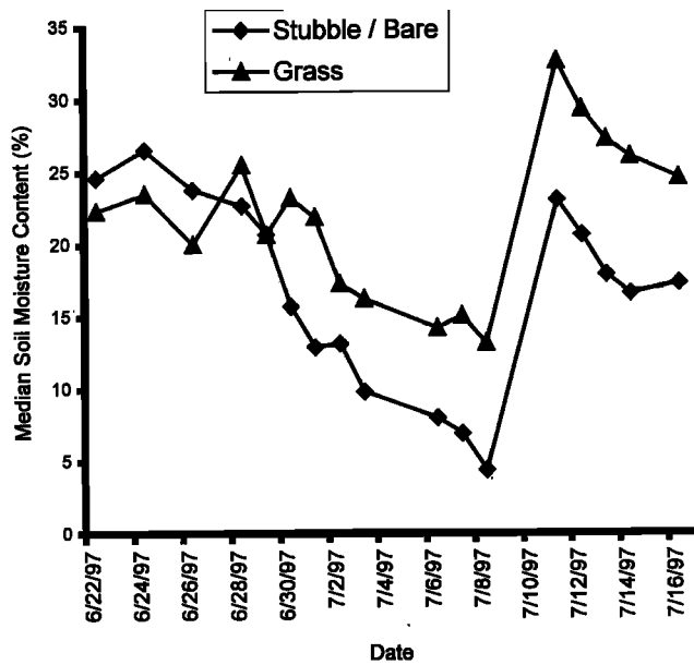
Figure 3. Temporal distribution of median soil moisture contents under different vegetation and land covers.
