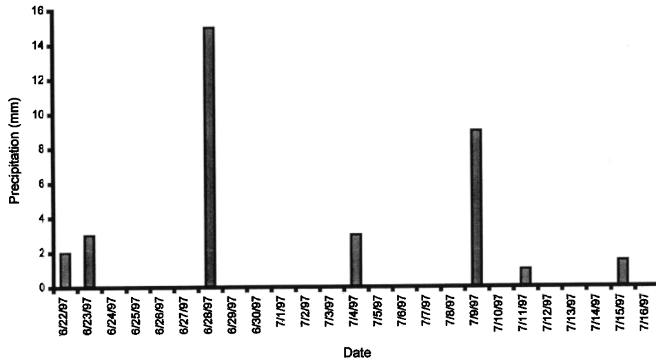
Figure 5. Observed precipitation near LW21 field site (APAC, Oklahoma Mesonet) during the SGP97 campaign.
