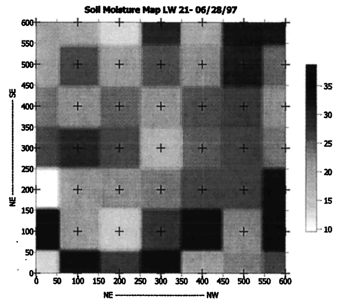
Figure 7. Contour plot of soil moisture content at LW21 on June 28, 1997. Soil moisture contents are in percent, and axes are in meters.
