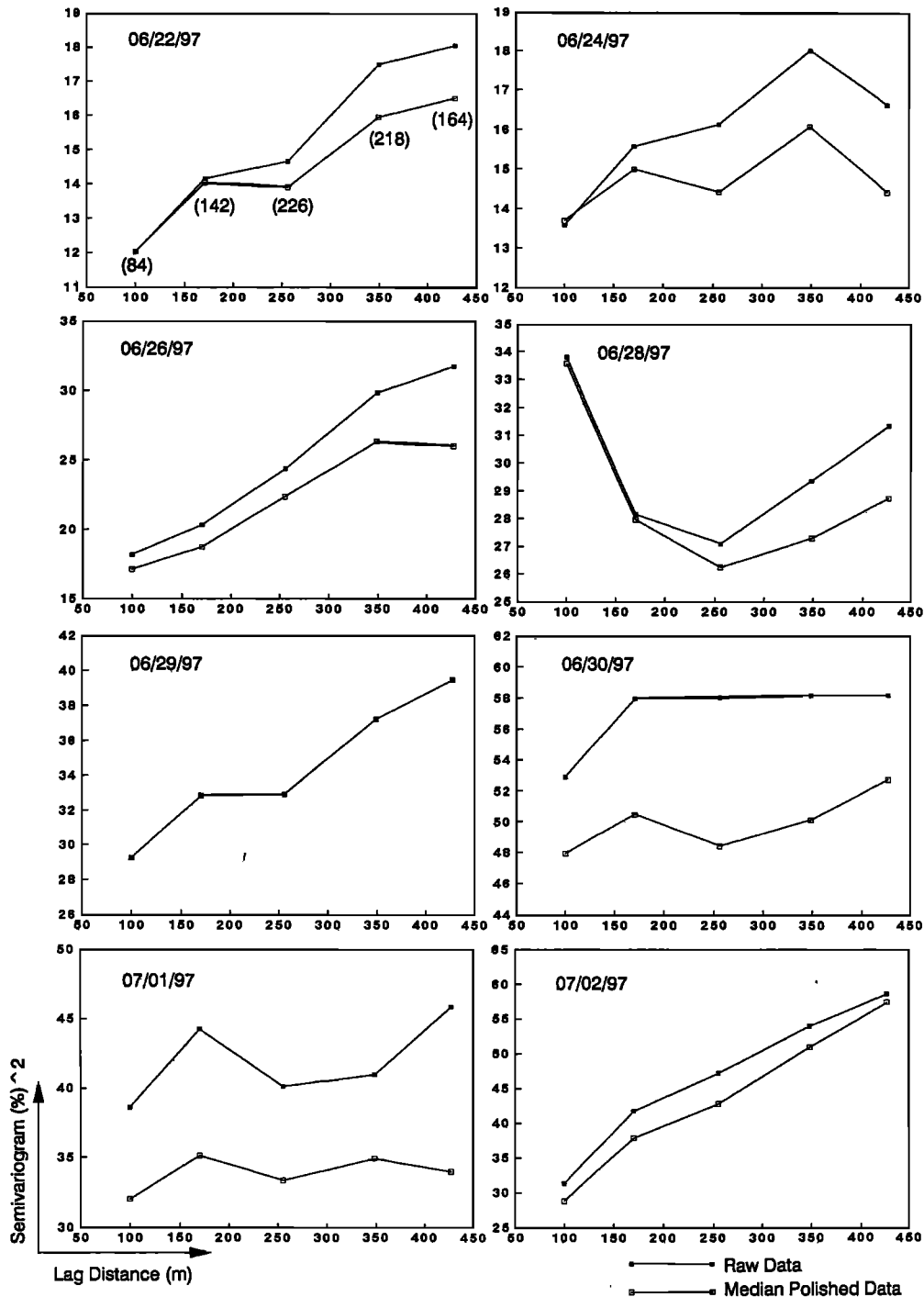
Figure 4. Daily isotropic experimental semivariograms of raw (including vegetation factor) and median polished (excluding vegetation factors) data showing the time evolution of spatial structure of surface soil moisture at LW21. Numbers in the parentheses show the data pairs used for semivariogram estimation for different lag distances. The same number of data pairs were used for each semivariogram estimation.
