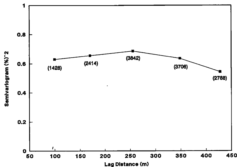
Figure 9. Time-averaged isotropic experimental semivariogram after vegetation and other temporal components were removed from raw soil moisture data using the median polishing scheme. Numbers in the parentheses show the data pairs used for semivariogram estimation for different lag distances.
