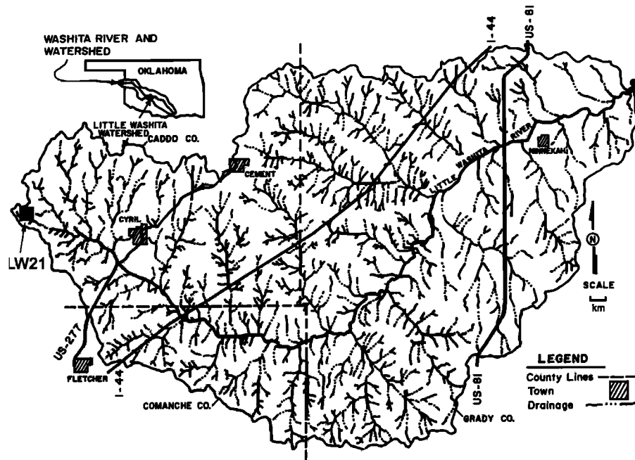
Figure 1. General map of the Little Washita watershed.
