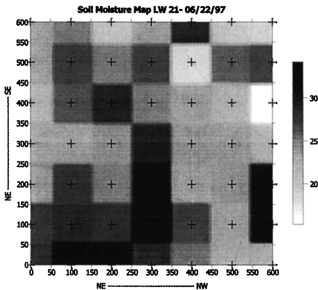
Figure 6. Contour plot of soil moisture content at LW21 on June 22, 1997. Soil moisture contents are in percent, and axes are in meters.
