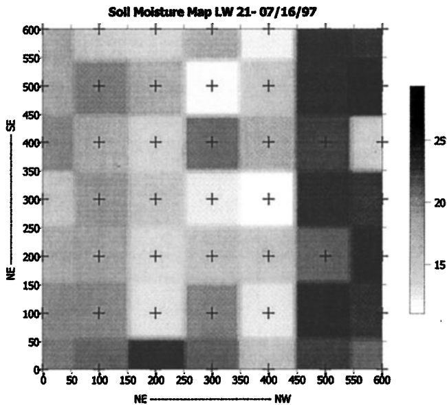
Figure 8. Contour plot of soil moisture content at LW21 on July 16, 1997. Soil moisture contents are in percent, and axes are in meters.
