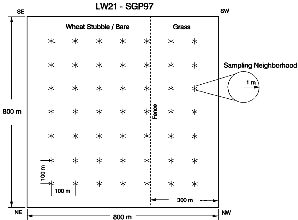
Figure 2. Soil moisture sampling grid in LW21.
