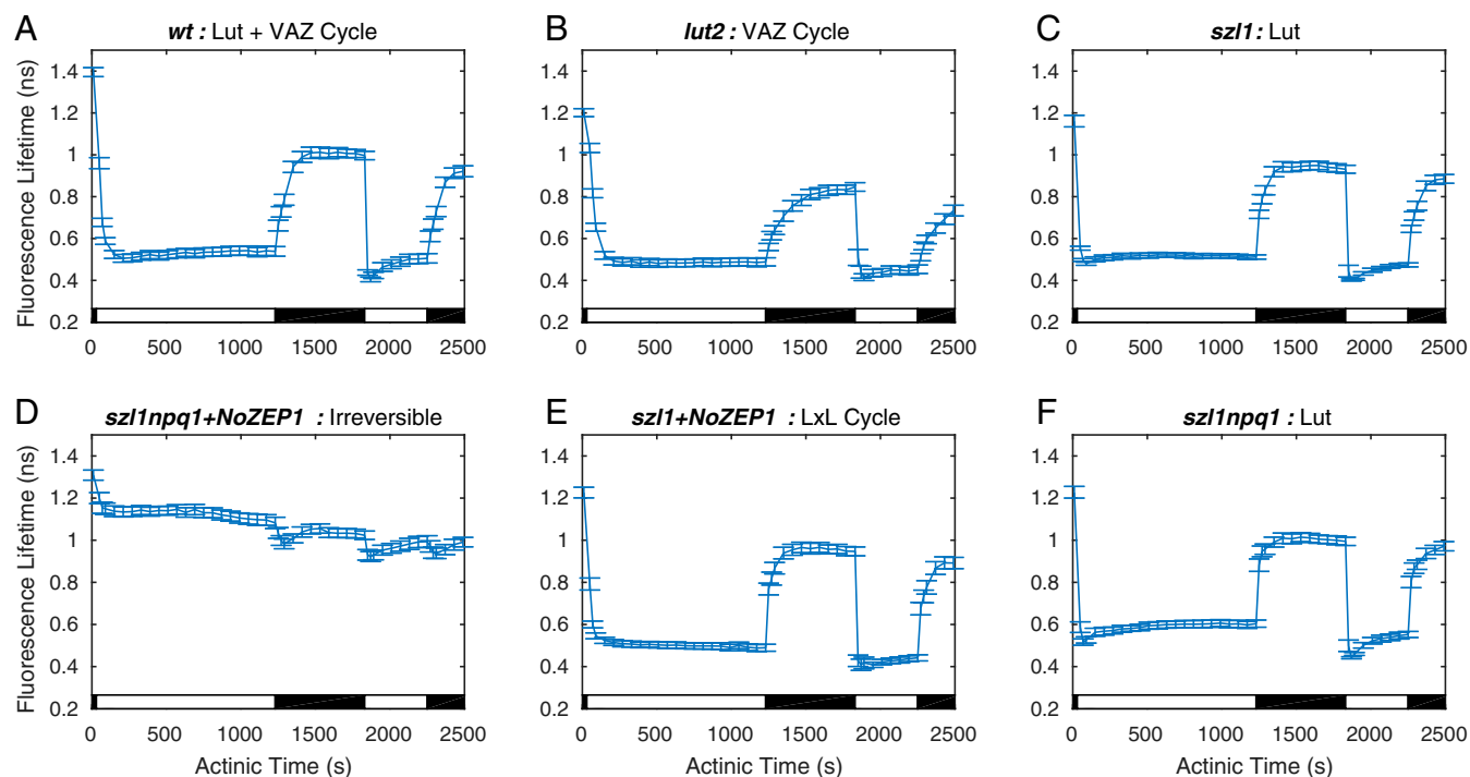
Fig. 2. Average fluorescence lifetime traces over a two-cycle light acclimation scheme shown by the light and dark bars superimposed on the bottom of each plot for six A. thaliana strains. Error bars denote SD for n = 20 . (A) The wt contains lutein and a VAZ cycle to form zeaxanthin in high light conditions. (B) The lut2 lacks lutein and has an active VAZ cycle. (C) The szl1 lacks zeaxanthin because of a partially blocked \beta -carotene biosynthesis pathway and contains more lutein than wt . (D) The szl1npq1+NoZEP1 strain does not have either xanthophyll cycle. (E) The szl1+NoZEP1 lacks zeaxanthin and contains a nonnative zeaxanthin epoxidase that functions on lutein, converting lutein to lutein epoxide that can be converted back to lutein by native VDE in high light. (F) The szl1npq1 contains lutein but lacks zeaxanthin because of blocking of the \beta -carotene biosynthesis pathway and inhibition of VDE.
