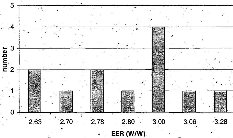
Figure 2.4 Distribution of EER in split air conditioners, C \leq 2500 W
