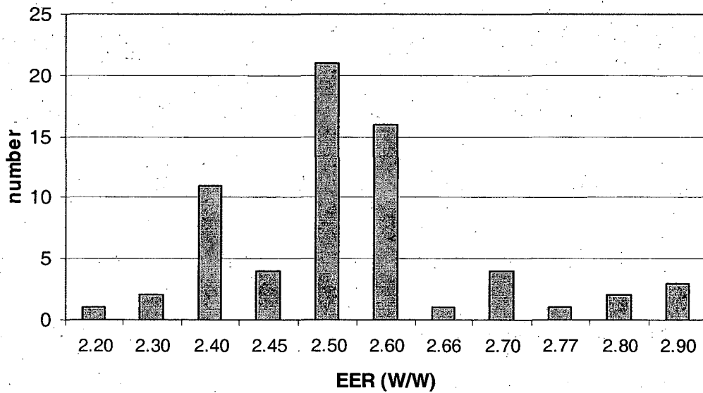
Figure 2.6 Distribution of EER in split air conditioners, 4500 \leq C < 7100 W
