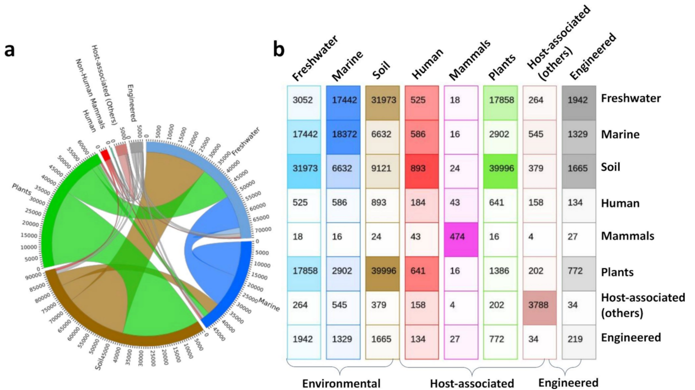
Extended Data Fig. 1 | Distribution of NMPF clusters across the eight ecosystem types. (a) Chord Plot. The distribution of the ecosystems is presented in a chord-like circular diagram. The rim of the diagram represents the total size of the ecosystem types (i.e. number of NMPFs in each ecosystem), with the numbers outside the rim indicating the size scale. The intersections of categories are represented by arcs drawn between them. The size of the arc is proportional to the importance of the flow. (b) 8x8 matrix. Each cell in the
